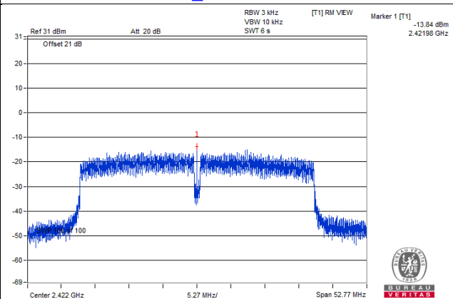
VHT40_Chain 1 / CH3
