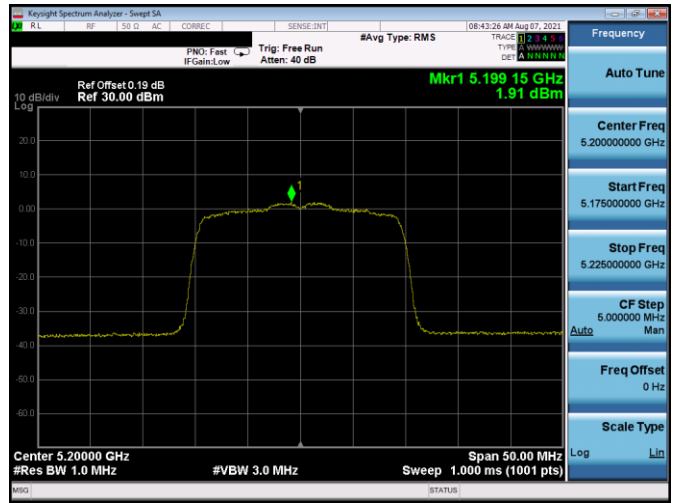
Plot 7-814. ISED PSD SDM Antenna 1b (20MHz BW 11ax(SU) – Ch.40, MCS2)
