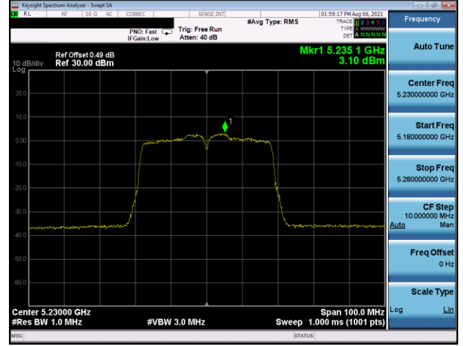
Plot 7-815. ISED PSD SDM Antenna 5T (40MHz BW 11n – Ch.46, MCS10)
