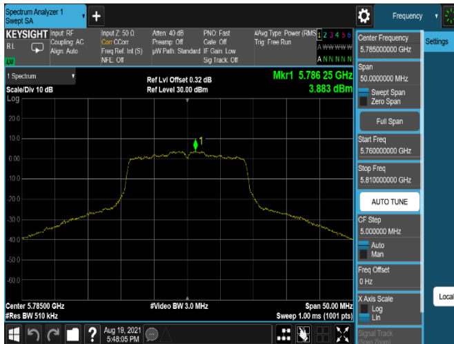
Plot 7-788. PSD CDD Antenna 1b (20MHz BW 802.11n – Ch. 157, MCS11)
