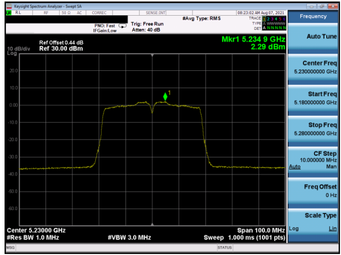
Plot 7-816. ISED PSD SDM Antenna 1b (40MHz BW 11n – Ch.46, MCS10)
