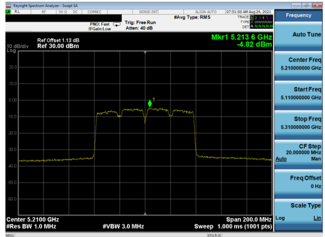
Plot 7-844. ISED PSD SDM Antenna 1b (80MHz BW 11ac – Ch.42, MCS5)
