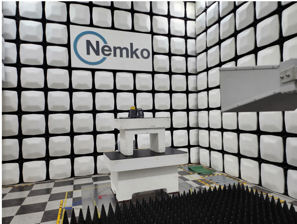
Radiated Test_Above 1GHz_Rear
