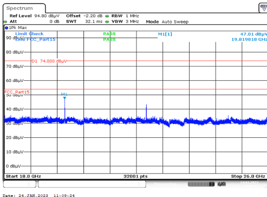
Plot 12: 18 GHz to 26 GHz, TX mode, 2478 MHz, vertical & horizontal polarization, 2 Msp/s
