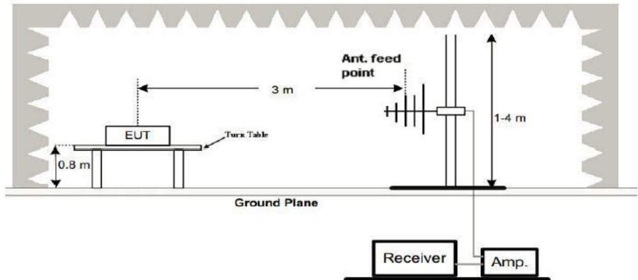
(B) Radiated Emission Test-Up Frequency 30MHz~1GHz
