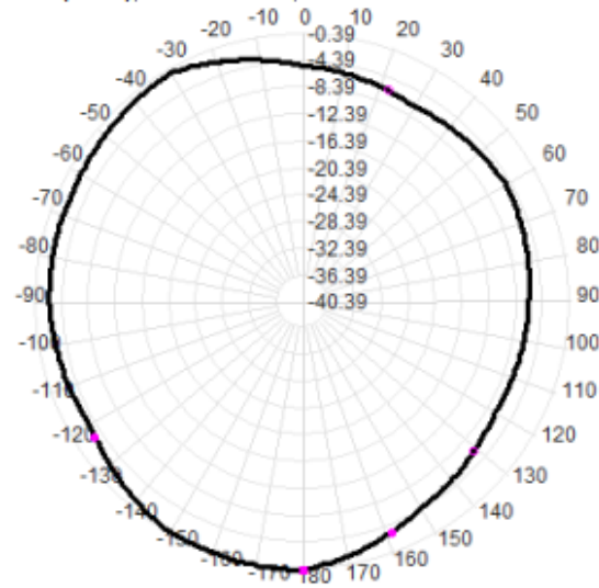
Total(H-XY), Max=-0.44dBi, CirD=6.89
