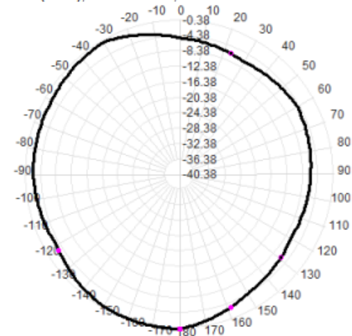
Total(H-XY), Max= -0.44dBi, CirD=6.74
