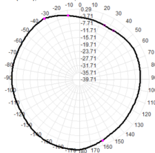
Total(H-XY), Max= 0.29dBi, CirD=6.34
