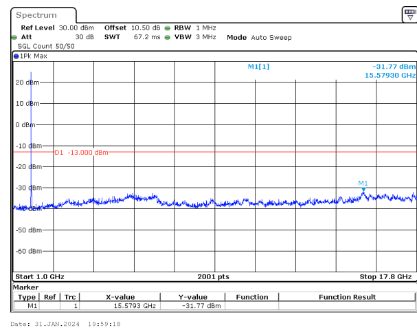
30MHz_15kHz_1765MHz_DFT-s-OFDM QPSK_RB1@0&-31.77 dBm
