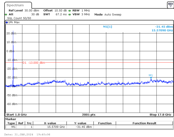
20MHz_15kHz_1770MHz_DFT-s-OFDM QPSK_RB1@105&-31.45 dBm
