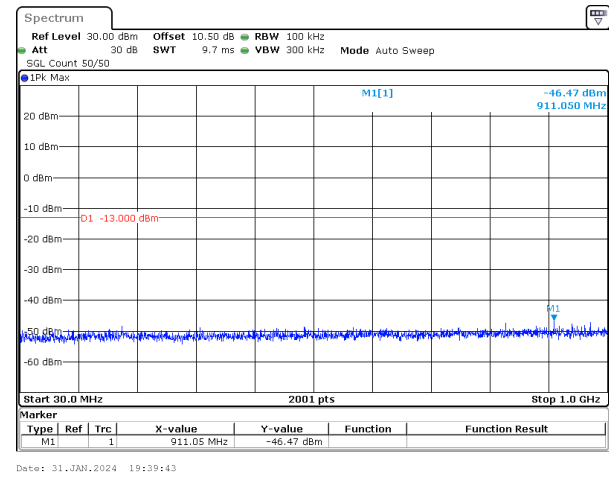
20MHz_15kHz_1770MHz_DFT-s-OFDM QPSK_RB1@105&-46.47 dBm
