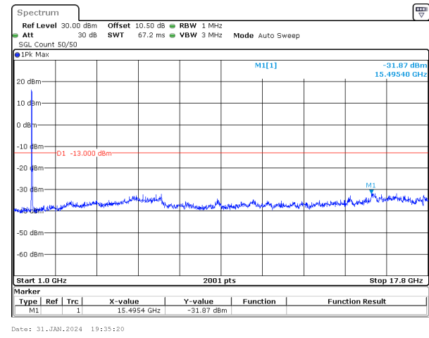
20MHz_15kHz_1720MHz_DFT-s-OFDM QPSK_RB100@0&-31.87 dBm
