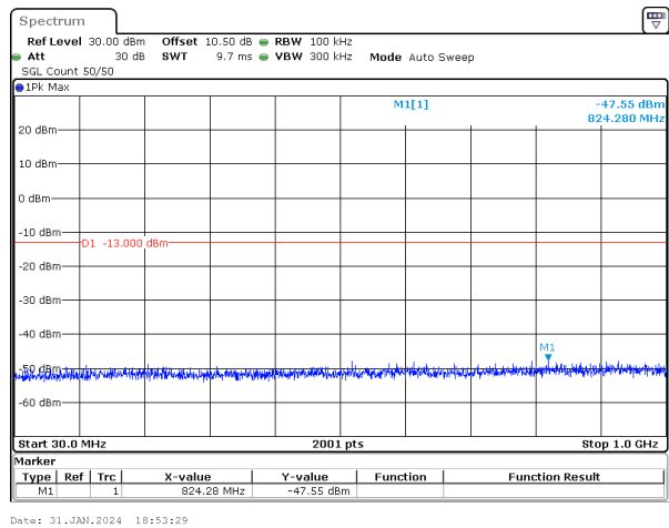
5MHz_15kHz_1745MHz_DFT-s-OFDM QPSK_RB1@24&-47.55 dBm
