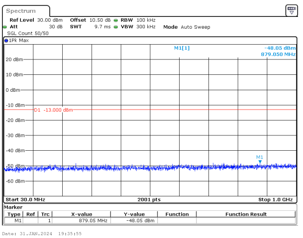
20MHz_15kHz_1745MHz_DFT-s-OFDM QPSK_RB1@0&-48.05 dBm
