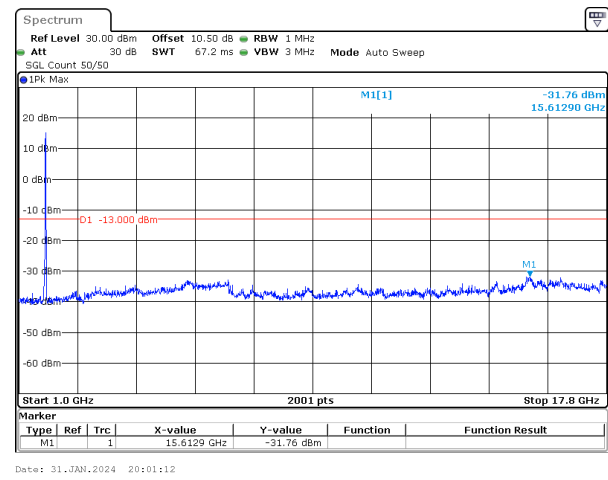
30MHz_15kHz_1765MHz_DFT-s-OFDM QPSK_RB160@0&-31.76 dBm
