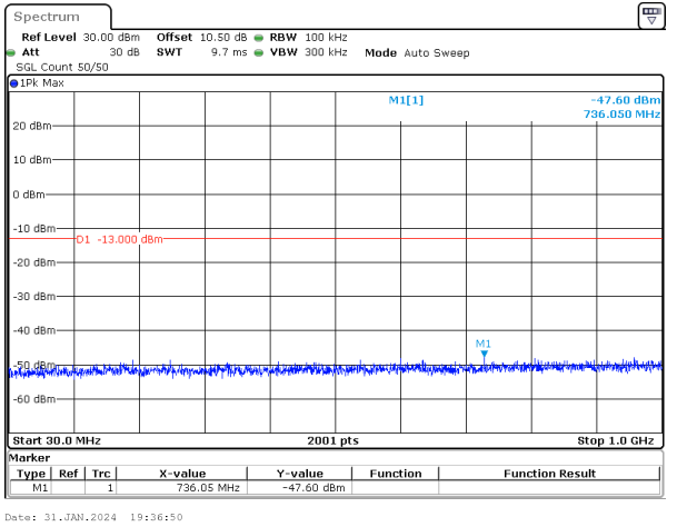
20MHz_15kHz_1745MHz_DFT-s-OFDM QPSK_RB1@105&-47.60 dBm
