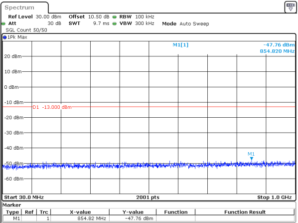
5MHz_15kHz_1777.5MHz_DFT-s-OFDM QPSK_RB1@0&-47.76 dBm
