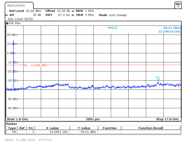
30MHz_15kHz_1725MHz_DFT-s-OFDM QPSK_RB160@0&-30.61 dBm
