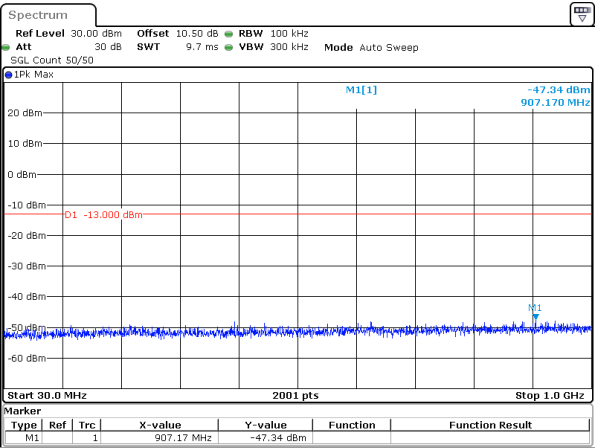
5MHz_15kHz_1712.5MHz_DFT-s-OFDM QPSK_RB1@0&-47.34 dBm
