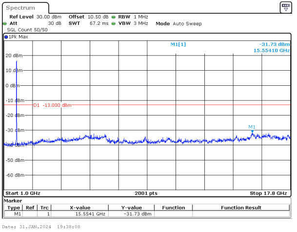
20MHz_15kHz_1745MHz_DFT-s-OFDM QPSK_RB100@0&-31.73 dBm
