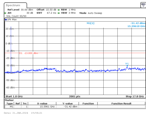
30MHz_15kHz_1745MHz_DFT-s-OFDM QPSK_RB1@0&-31.42 dBm
