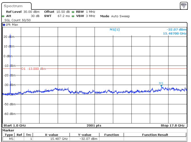
10MHz_15kHz_1715MHz_DFT-s-OFDM QPSK_RB1@0&-32.07 dBm
