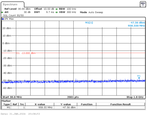
40MHz_15kHz_1745MHz_DFT-s-OFDM QPSK_RB1@215&-47.56 dBm
