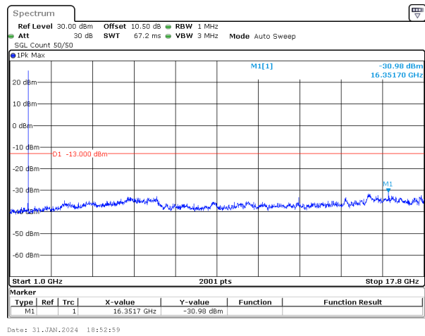
5MHz_15kHz_1745MHz_DFT-s-OFDM QPSK_RB1@0&-30.98 dBm
