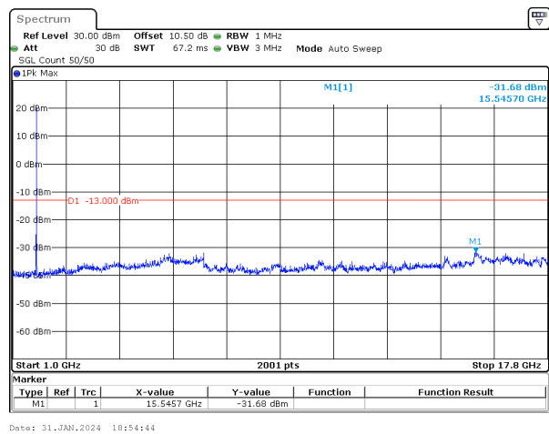
5MHz_15kHz_1745MHz_DFT-s-OFDM QPSK_RB25@0&-31.68 dBm
