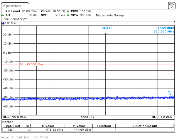
40MHz_15kHz_1745MHz_DFT-s-OFDM QPSK_RB216@0&-47.69 dBm
