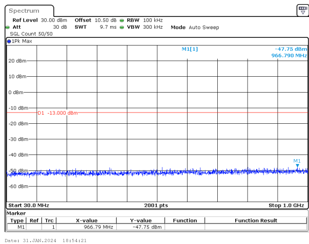
5MHz_15kHz_1745MHz_DFT-s-OFDM QPSK_RB25@0&-47.75 dBm
