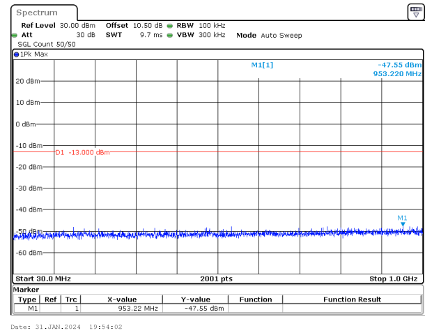
30MHz_15kHz_1725MHz_DFT-s-OFDM QPSK_RB1@159&-47.55 dBm
