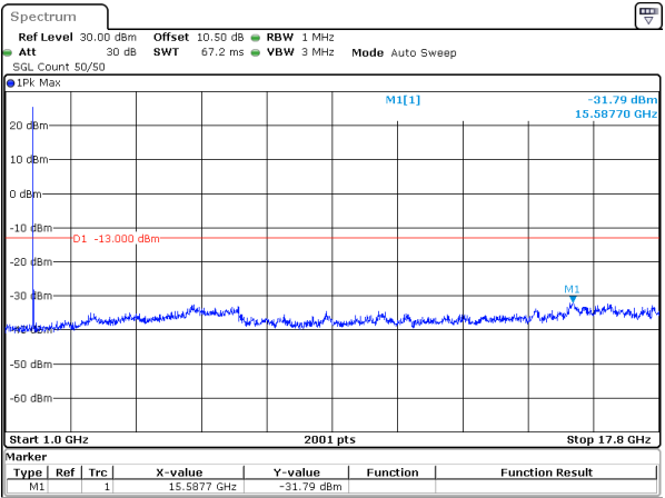
5MHz_15kHz_1712.5MHz_DFT-s-OFDM QPSK_RB1@0&-31.79 dBm
