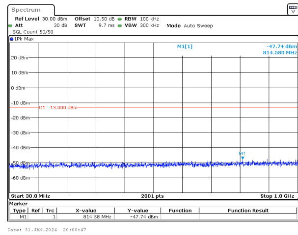
30MHz_15kHz_1765MHz_DFT-s-OFDM QPSK_RB160@0&-47.74 dBm
