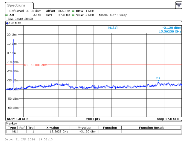
30MHz_15kHz_1745MHz_DFT-s-OFDM QPSK_RB160@0&-31.20 dBm
