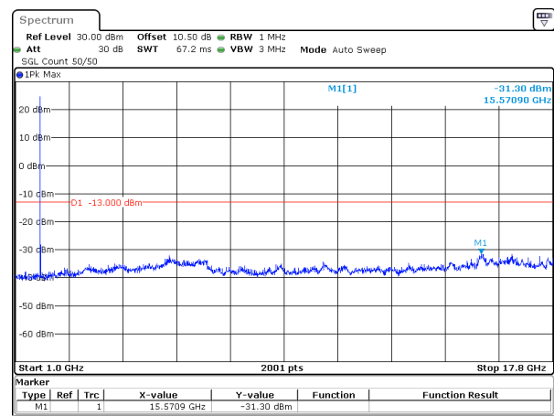
10MHz_15kHz_1775MHz_DFT-s-OFDM QPSK_RB1@0&-31.30 dBm
