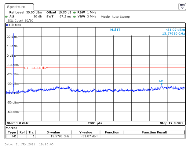
25MHz_15kHz_1745MHz_DFT-s-OFDM QPSK_RB1@0&-31.07 dBm
