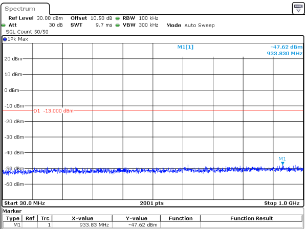
5MHz_15kHz_1777.5MHz_DFT-s-OFDM QPSK_RB1@24&-47.62 dBm
