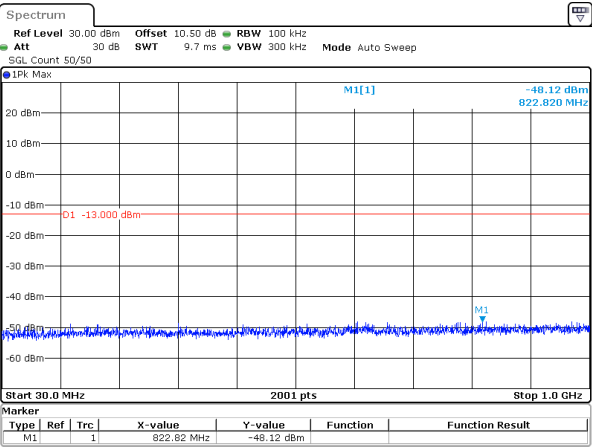
15MHz_15kHz_1772.5MHz_DFT-s-OFDM QPSK_RB1@0&-48.12 dBm
