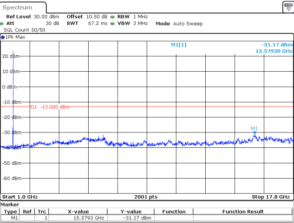
15MHz_15kHz_1717.5MHz_DFT-s-OFDM QPSK_RB1@78&-31.17 dBm
