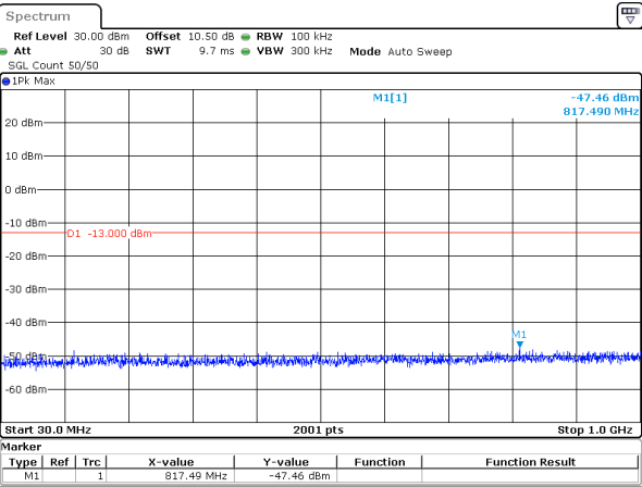
15MHz_15kHz_1772.5MHz_DFT-s-OFDM QPSK_RB1@78&-47.46 dBm
