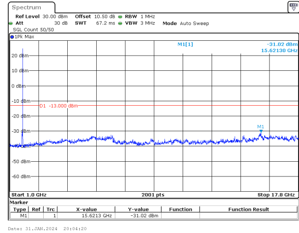
40MHz_15kHz_1730MHz_DFT-s-OFDM QPSK_RB1@215&-31.02 dBm
