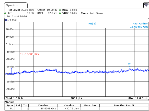
40MHz_15kHz_1730MHz_DFT-s-OFDM QPSK_RB1@0&-30.72 dBm
