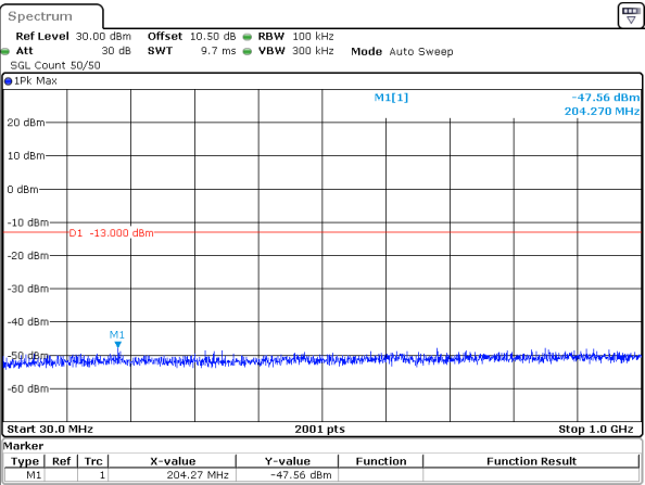
25MHz_15kHz_1767.5MHz_DFT-s-OFDM QPSK_RB1@0&-47.56 dBm
