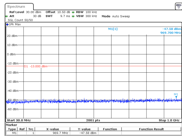
40MHz_15kHz_1745MHz_DFT-s-OFDM QPSK_RB1@0&-47.58 dBm
