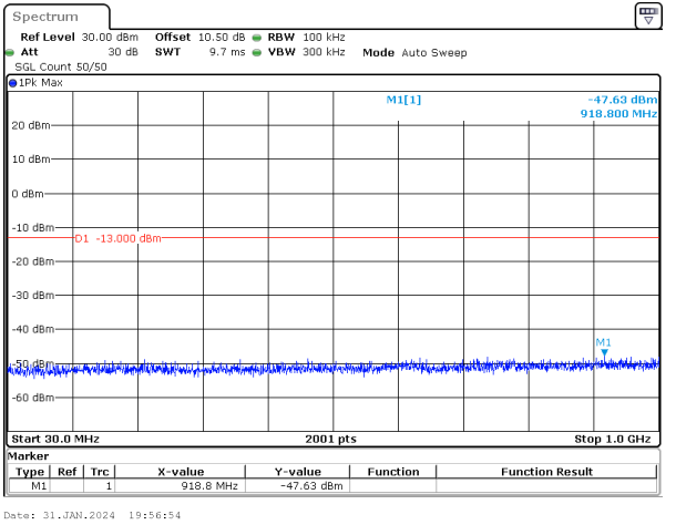
30MHz_15kHz_1745MHz_DFT-s-OFDM QPSK_RB1@159&-47.63 dBm
