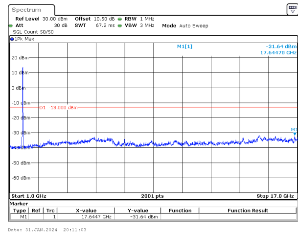
40MHz_15kHz_1760MHz_DFT-s-OFDM QPSK_RB216@0&-31.64 dBm
