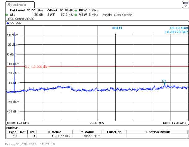
30MHz_15kHz_1745MHz_DFT-s-OFDM QPSK_RB1@159&-32.19 dBm
