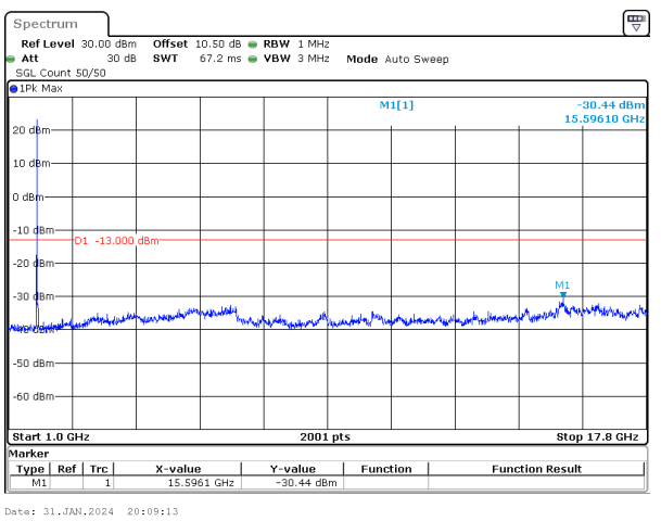
40MHz_15kHz_1760MHz_DFT-s-OFDM QPSK_RB1@0&-30.44 dBm
