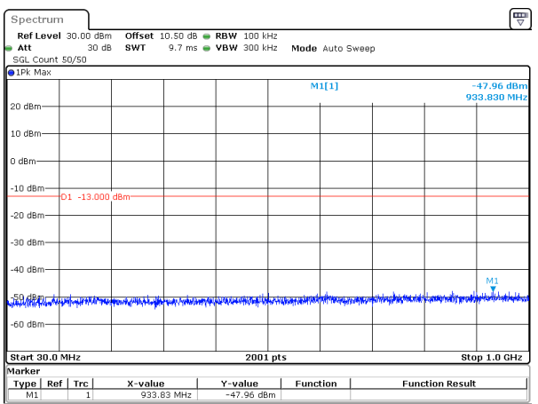
10MHz_15kHz_1745MHz_DFT-s-OFDM QPSK_RB1@0&-47.96 dBm
