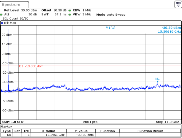
15MHz_15kHz_1772.5MHz_DFT-s-OFDM QPSK_RB1@78&-30.50 dBm
