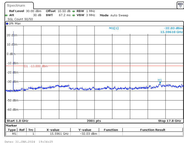
20MHz_15kHz_1720MHz_DFT-s-OFDM QPSK_RB1@105&-32.03 dBm
