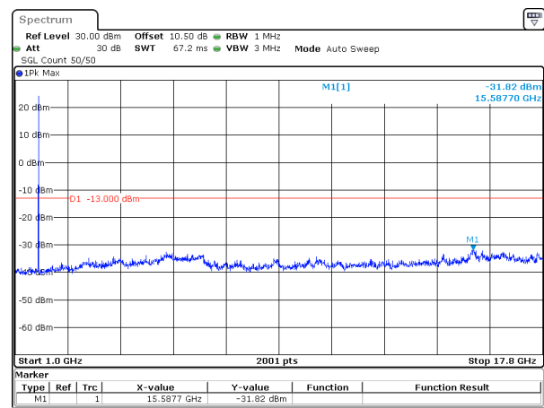
10MHz_15kHz_1745MHz_DFT-s-OFDM QPSK_RB1@0&-31.82 dBm
