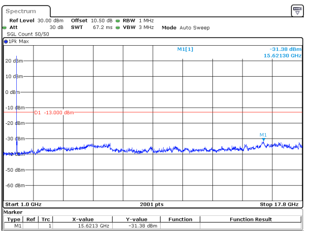
40MHz_15kHz_1745MHz_DFT-s-OFDM QPSK_RB1@0&-31.38 dBm
