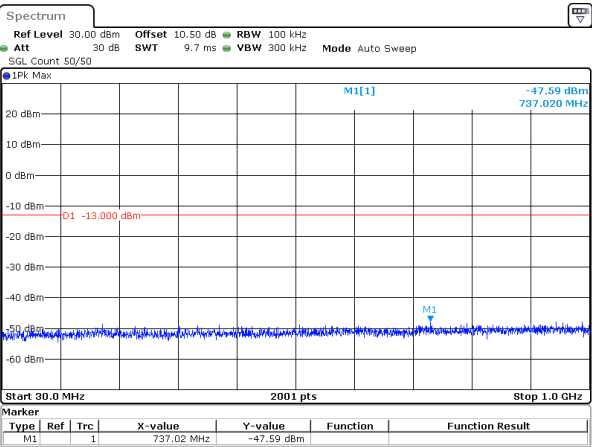
15MHz_15kHz_1717.5MHz_DFT-s-OFDM QPSK_RB75@0&-47.59 dBm
