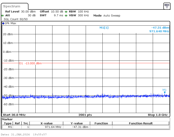
30MHz_15kHz_1745MHz_DFT-s-OFDM QPSK_RB1@0&-47.31 dBm
