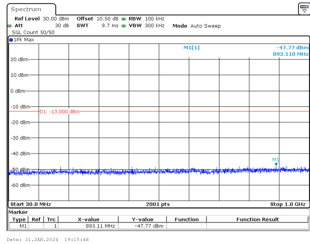
10MHz_15kHz_1775MHz_DFT-s-OFDM QPSK_RB1@51&-47.77 dBm
