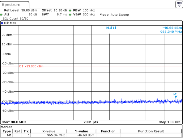
15MHz_15kHz_1717.5MHz_DFT-s-OFDM QPSK_RB1@0&-46.68 dBm
