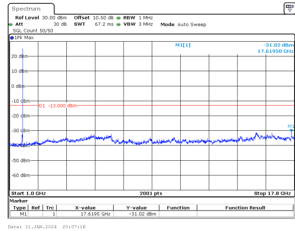
40MHz_15kHz_1745MHz_DFT-s-OFDM QPSK_RB1@215&-31.02 dBm
