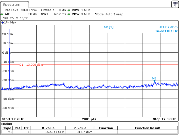
25MHz_15kHz_1767.5MHz_DFT-s-OFDM QPSK_RB1@132&-31.87 dBm
