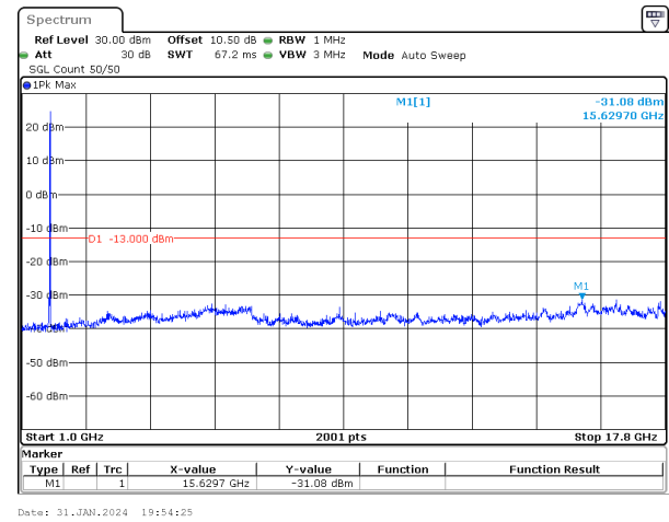
30MHz_15kHz_1725MHz_DFT-s-OFDM QPSK_RB1@159&-31.08 dBm
