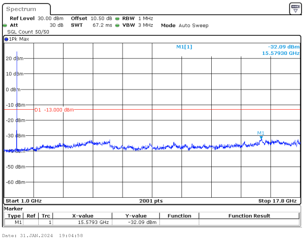
10MHz_15kHz_1715MHz_DFT-s-OFDM QPSK_RB1@51&-32.09 dBm
