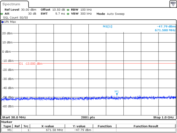
5MHz_15kHz_1712.5MHz_DFT-s-OFDM QPSK_RB1@24&-47.79 dBm
