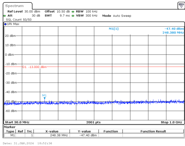
5MHz_15kHz_1745MHz_DFT-s-OFDM QPSK_RB1@0&-47.40 dBm
