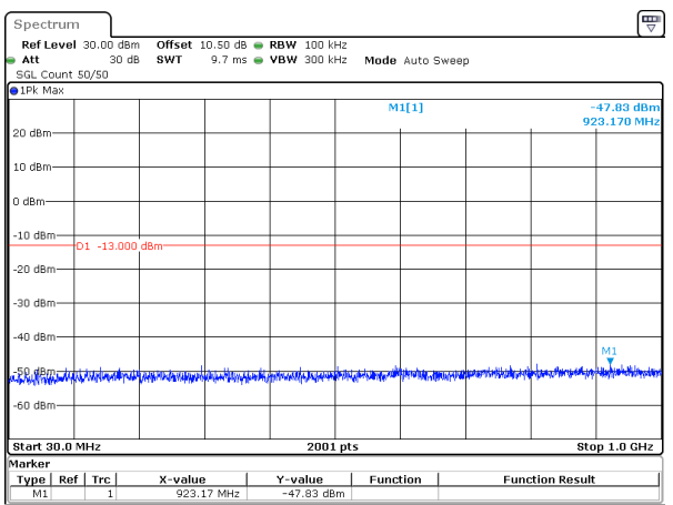
10MHz_15kHz_1775MHz_DFT-s-OFDM QPSK_RB1@0&-47.83 dBm
