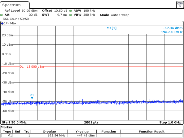
25MHz_15kHz_1767.5MHz_DFT-s-OFDM QPSK_RB128@0&-47.45 dBm
