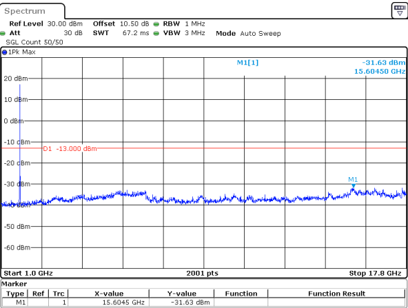
15MHz_15kHz_1772.5MHz_DFT-s-OFDM QPSK_RB75@0&-31.63 dBm
