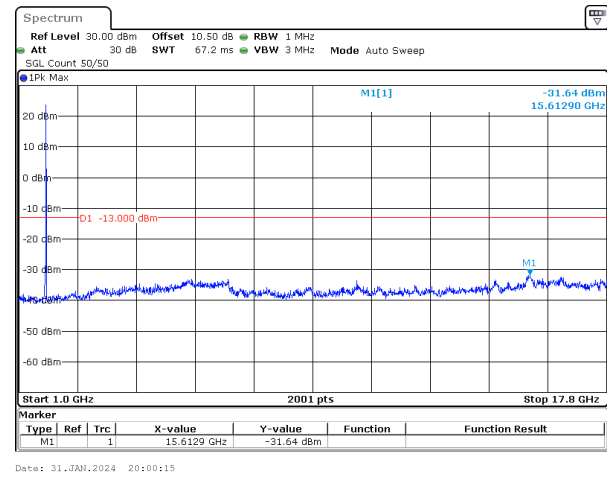
30MHz_15kHz_1765MHz_DFT-s-OFDM QPSK_RB1@159&-31.64 dBm
