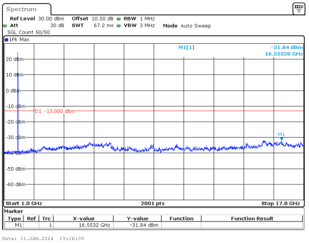
10MHz_15kHz_1775MHz_DFT-s-OFDM QPSK_RB1@51&-31.84 dBm
