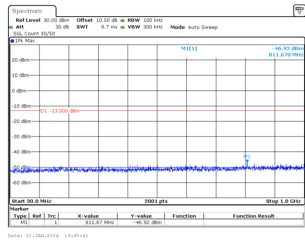
25MHz_15kHz_1745MHz_DFT-s-OFDM QPSK_RB1@0&-46.92 dBm
