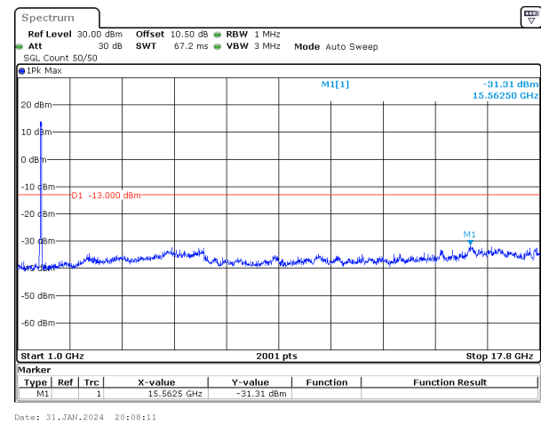
40MHz_15kHz_1745MHz_DFT-s-OFDM QPSK_RB216@0&-31.31 dBm
