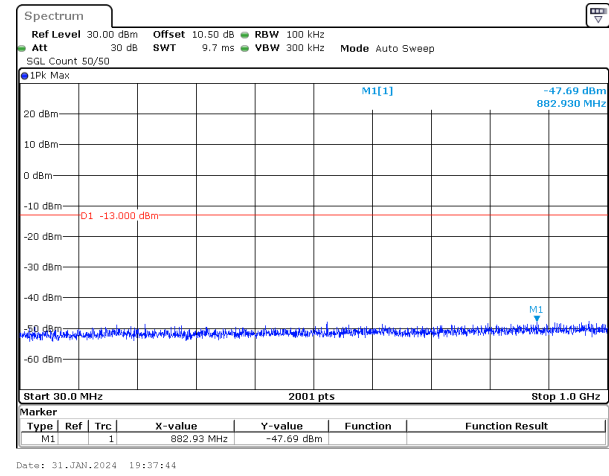
20MHz_15kHz_1745MHz_DFT-s-OFDM QPSK_RB100@0&-47.69 dBm
