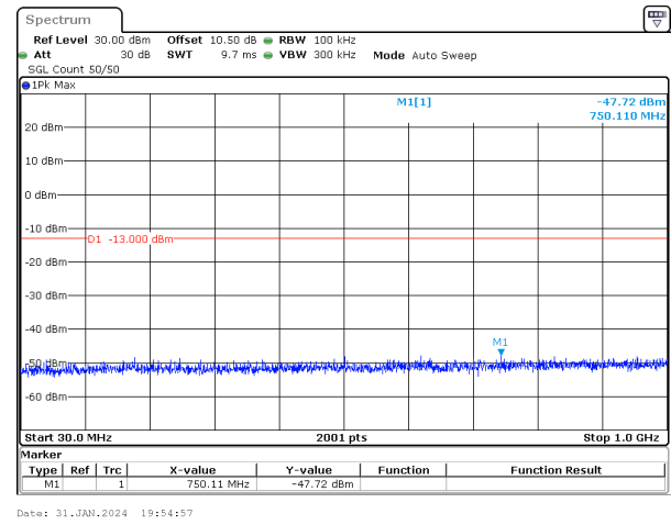
30MHz_15kHz_1725MHz_DFT-s-OFDM QPSK_RB160@0&-47.72 dBm
