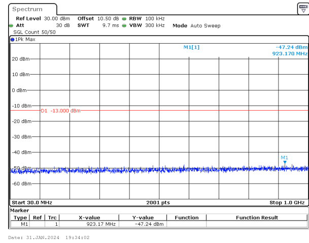
20MHz_15kHz_1720MHz_DFT-s-OFDM QPSK_RB1@105&-47.24 dBm
