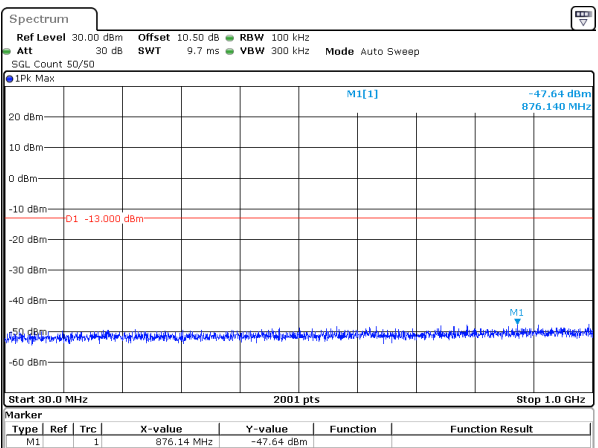
5MHz_15kHz_1777.5MHz_DFT-s-OFDM QPSK_RB25@0&-47.64 dBm
