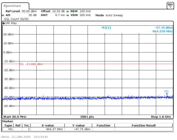
40MHz_15kHz_1760MHz_DFT-s-OFDM QPSK_RB216@0&-47.75 dBm
