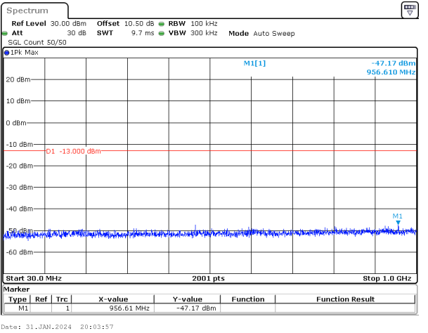
40MHz_15kHz_1730MHz_DFT-s-OFDM QPSK_RB1@215&-47.17 dBm
