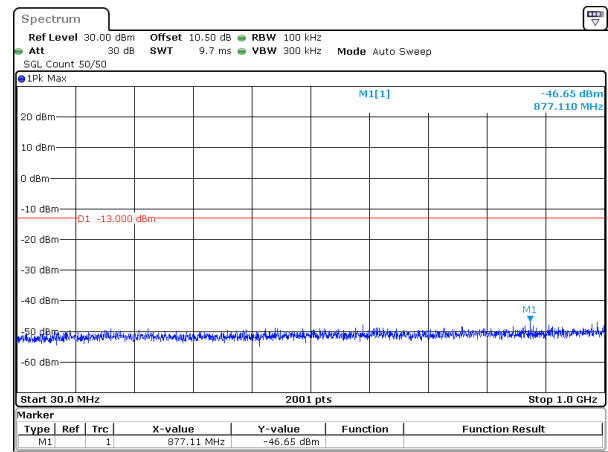
10MHz_15kHz_1715MHz_DFT-s-OFDM QPSK_RB1@0&-46.65 dBm
