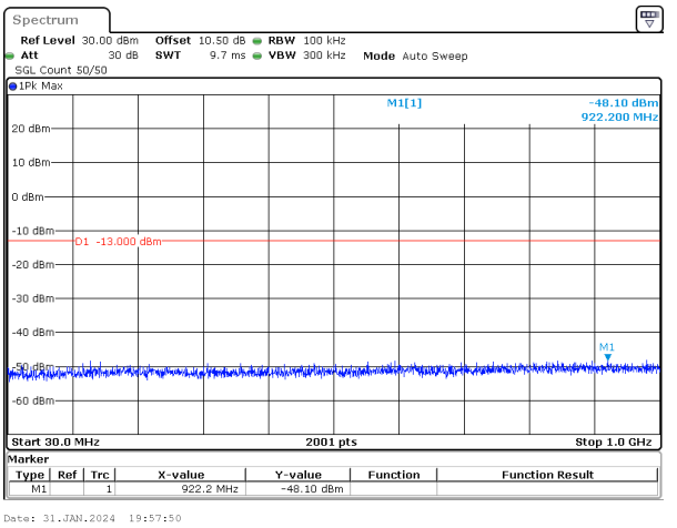
30MHz_15kHz_1745MHz_DFT-s-OFDM QPSK_RB160@0&-48.10 dBm
