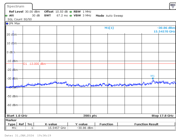
20MHz_15kHz_1745MHz_DFT-s-OFDM QPSK_RB1@0&-30.86 dBm
