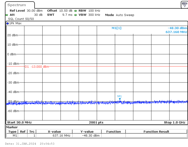
40MHz_15kHz_1730MHz_DFT-s-OFDM QPSK_RB216@0&-48.30 dBm
