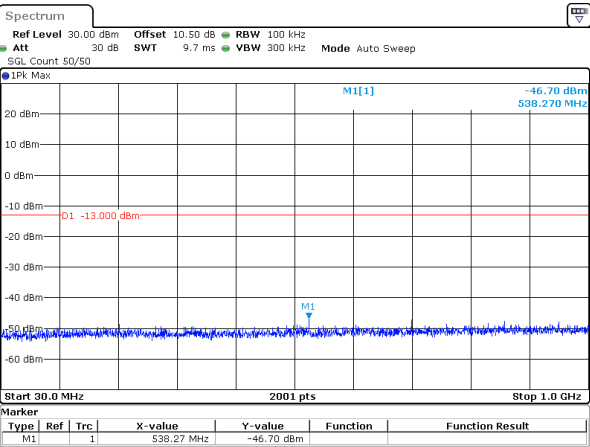
15MHz_15kHz_1772.5MHz_DFT-s-OFDM QPSK_RB75@0&-46.70 dBm
