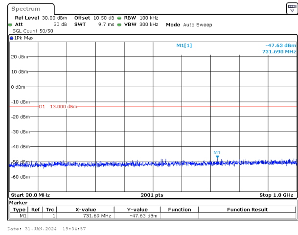
20MHz_15kHz_1720MHz_DFT-s-OFDM QPSK_RB100@0&-47.63 dBm
