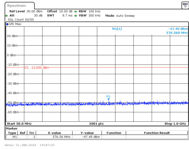
25MHz_15kHz_1745MHz_DFT-s-OFDM QPSK_RB128@0&-47.49 dBm
