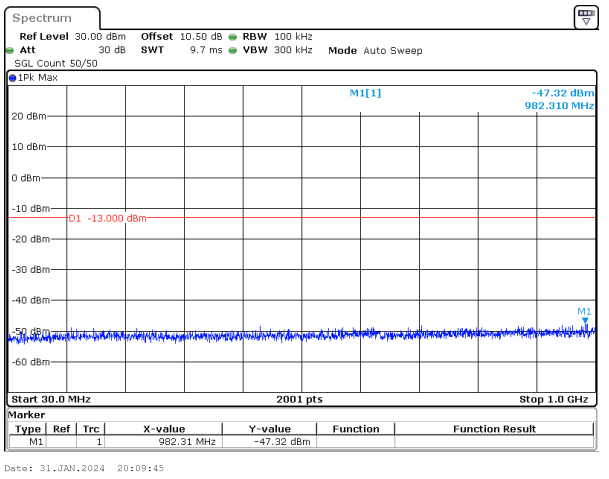
40MHz_15kHz_1760MHz_DFT-s-OFDM QPSK_RB1@215&-47.32 dBm
