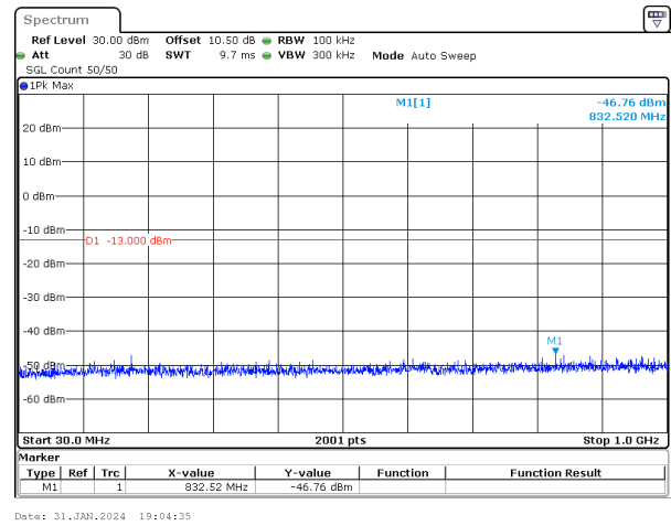
10MHz_15kHz_1715MHz_DFT-s-OFDM QPSK_RB1@51&-46.76 dBm
