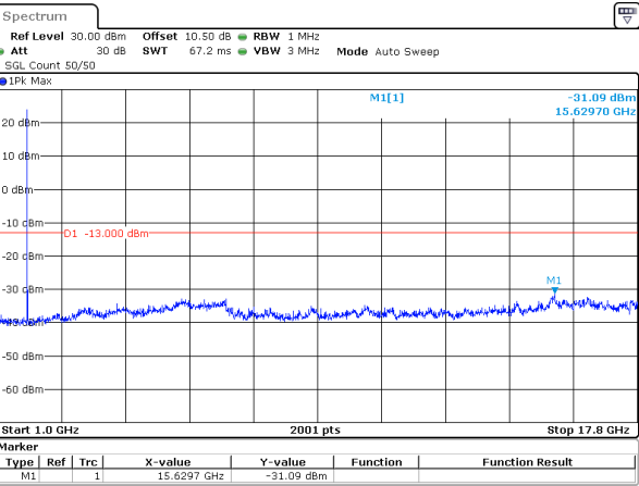
5MHz_15kHz_1777.5MHz_DFT-s-OFDM QPSK_RB1@0&-31.09 dBm
