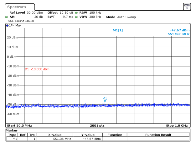
30MHz_15kHz_1725MHz_DFT-s-OFDM QPSK_RB1@0&-47.67 dBm
