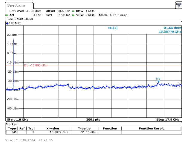
25MHz_15kHz_1745MHz_DFT-s-OFDM QPSK_RB128@0&-31.65 dBm
