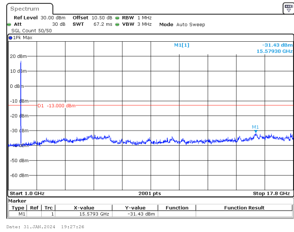
15MHz_15kHz_1745MHz_DFT-s-OFDM QPSK_RB75@0&-31.43 dBm
