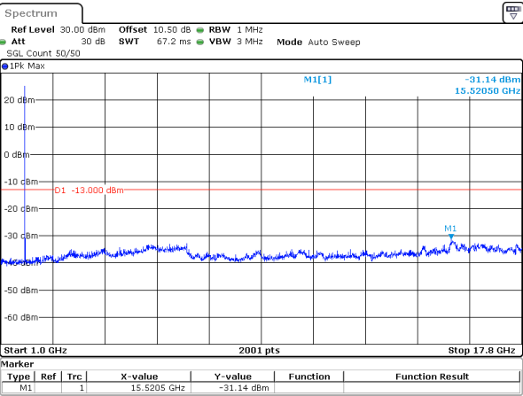
15MHz_15kHz_1772.5MHz_DFT-s-OFDM QPSK_RB1@0&-31.14 dBm
