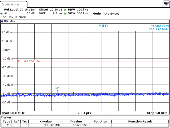
25MHz_15kHz_1767.5MHz_DFT-s-OFDM QPSK_RB1@132&-47.63 dBm
