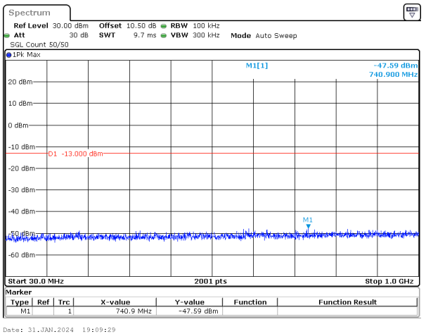
10MHz_15kHz_1745MHz_DFT-s-OFDM QPSK_RB1@51&-47.59 dBm
