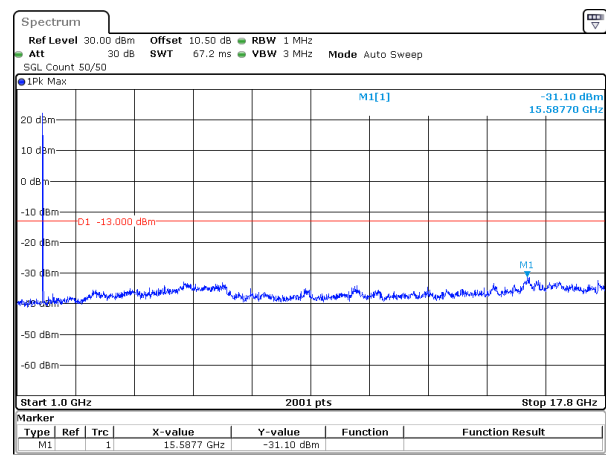
15MHz_15kHz_1745MHz_DFT-s-OFDM QPSK_RB1@0&-31.10 dBm
