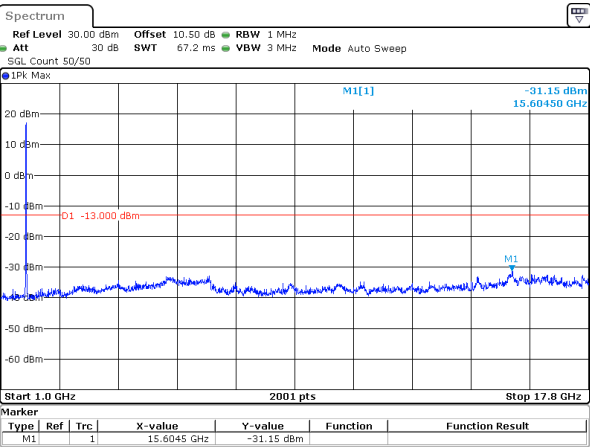
15MHz_15kHz_1717.5MHz_DFT-s-OFDM QPSK_RB75@0&-31.15 dBm
