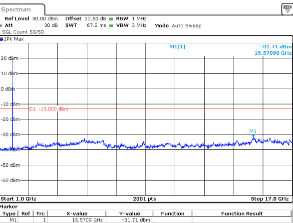
5MHz_15kHz_1777.5MHz_DFT-s-OFDM QPSK_RB25@0&-31.71 dBm
