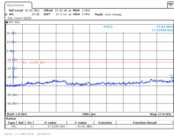
25MHz_15kHz_1745MHz_DFT-s-OFDM QPSK_RB1@132&-31.81 dBm
