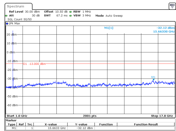
30MHz_15kHz_1725MHz_DFT-s-OFDM QPSK_RB1@0&-32.12 dBm
