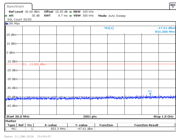
30MHz_15kHz_1765MHz_DFT-s-OFDM QPSK_RB1@0&-47.61 dBm
