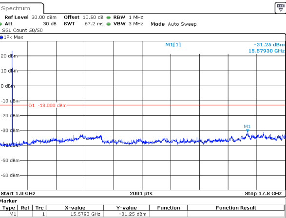
5MHz_15kHz_1777.5MHz_DFT-s-OFDM QPSK_RB1@24&-31.25 dBm
