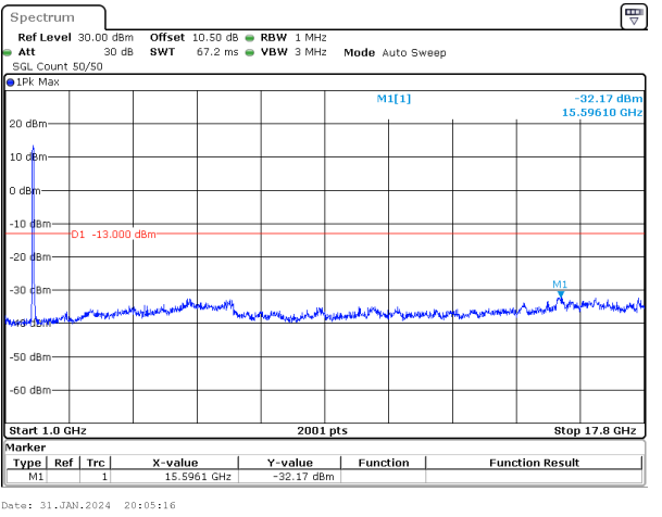
40MHz_15kHz_1730MHz_DFT-s-OFDM QPSK_RB216@0&-32.17 dBm
