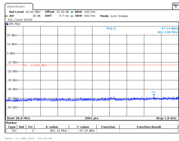
40MHz_15kHz_1760MHz_DFT-s-OFDM QPSK_RB1@0&-47.14 dBm
