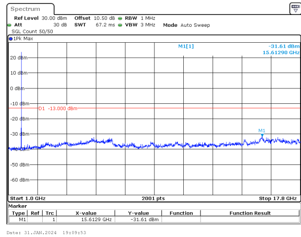
10MHz_15kHz_1745MHz_DFT-s-OFDM QPSK_RB1@51&-31.61 dBm
