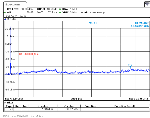
15MHz_15kHz_1745MHz_DFT-s-OFDM QPSK_RB1@78&-31.25 dBm
