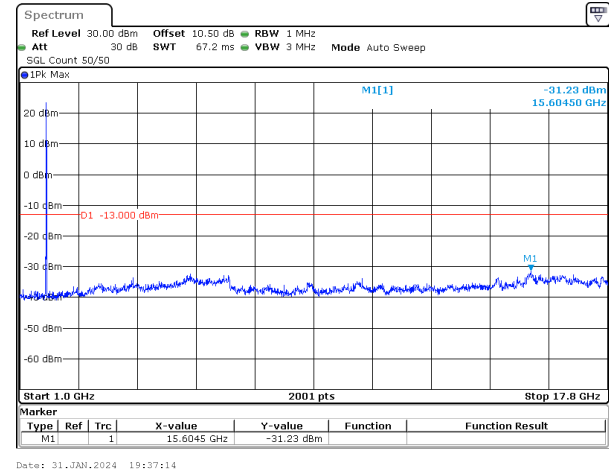
20MHz_15kHz_1745MHz_DFT-s-OFDM QPSK_RB1@105&-31.23 dBm
