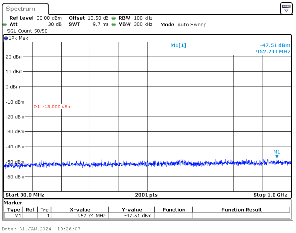
15MHz_15kHz_1745MHz_DFT-s-OFDM QPSK_RB1@78&-47.51 dBm
