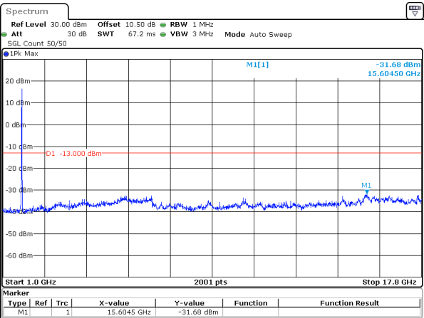
25MHz_15kHz_1767.5MHz_DFT-s-OFDM QPSK_RB128@0&-31.68 dBm
