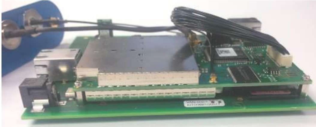
Figure 3 – Main PCB
