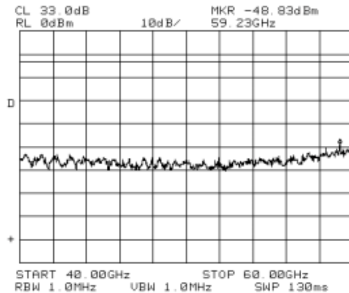
Fig. A-36 (Conducted Spurious Emissions, 16QAM, 2 carriers, 40 – 60GHz)
