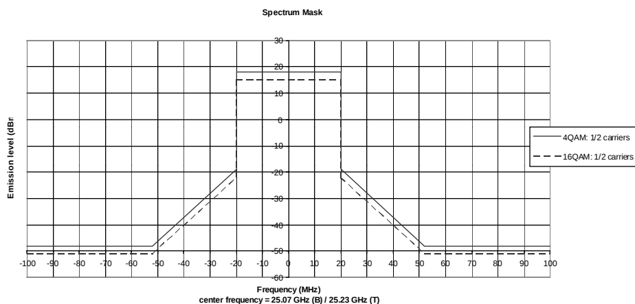
Fig. 5-1: Spectrum Mask limit
