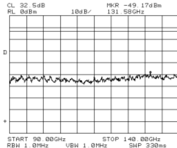
Fig. A-20 (Conducted Spurious Emissions, 4QAM, 1 carrier, 90 – 140GHz)
