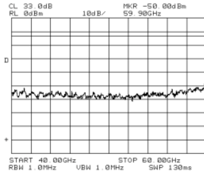
Fig. A-18 (Conducted Spurious Emissions, 4QAM, 1 carrier, 40 – 60GHz)
