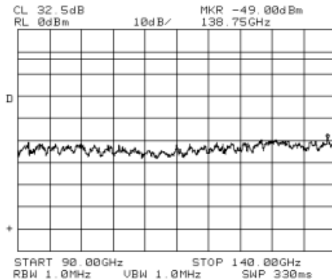
Fig. A-38 (Conducted Spurious Emissions, 16QAM, 2 carriers, 90 – 140GHz)
