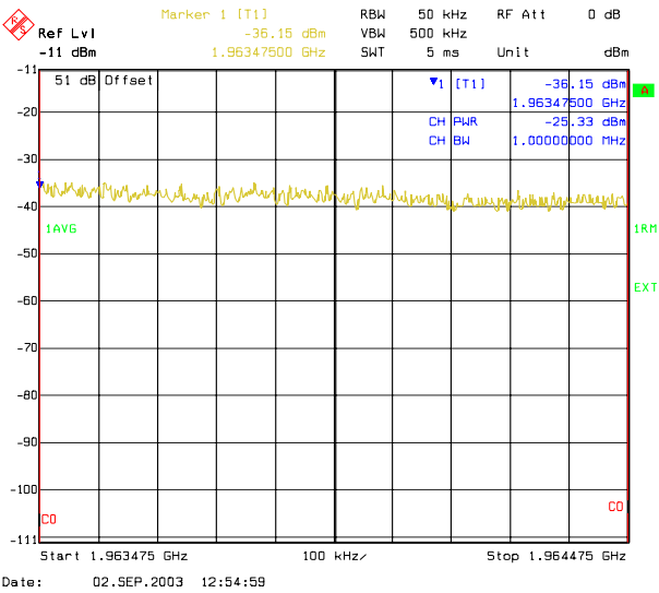
1963.475 MHz-1964.475 MHz
