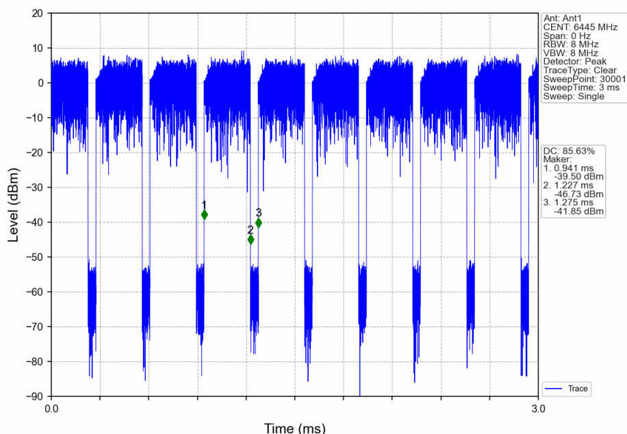
802.11ax(HEW40)_LCH_6445MHz_RU484_Left_Ant1_NTNV
