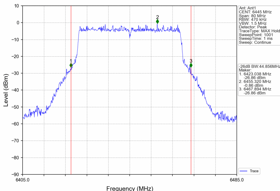
802.11ax(HEW40)_LCH_6445MHz_RU484_Left_Ant1_NTNV
