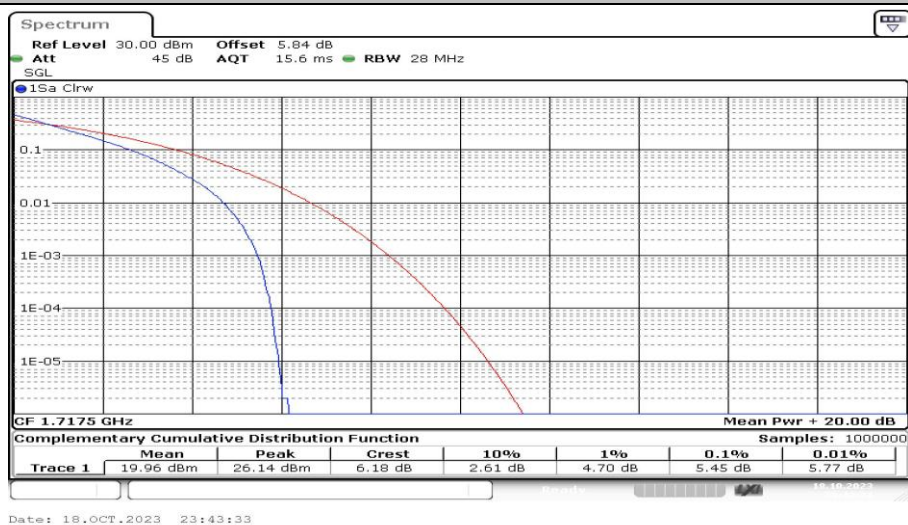
Band4-15MHz-QPSK-20025-75RB#0-PASS
