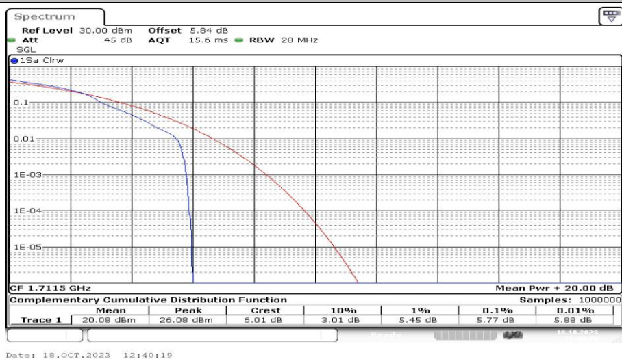
Band4-3MHz-16QAM-19965-1RB#0-PASS
