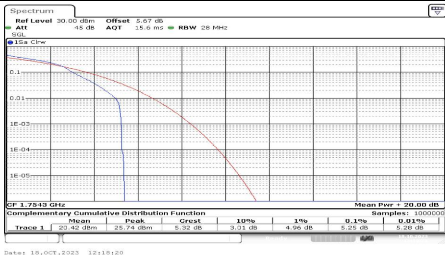
Band4-1.4MHz-16QAM-20393-1RB#0-PASS
