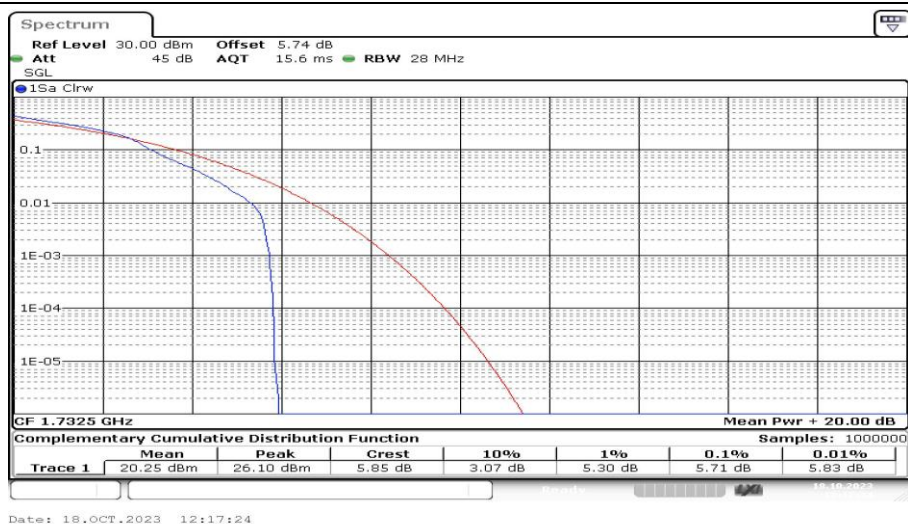
Band4-1.4MHz-16QAM-20175-1RB#0-PASS
