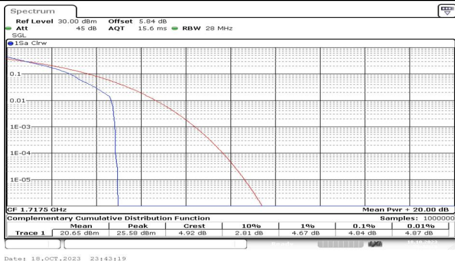
Band4-15MHz-QPSK-20025-1RB#0-PASS
