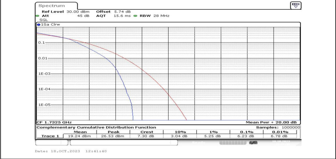
Band4-3MHz-16QAM-20175-15RB#0-PASS
