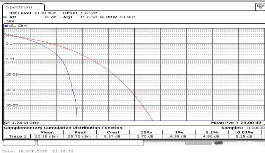
Band4-1.4MHz-QPSK-20393-6RB#0-PASS
