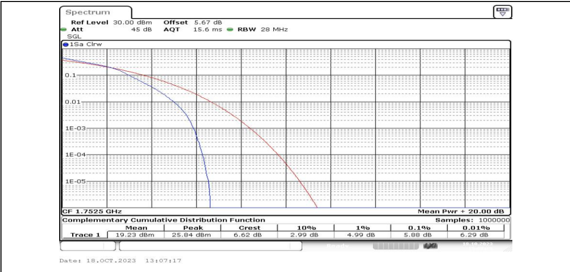
Band4-5MHz-16QAM-20375-25RB#0-PASS
