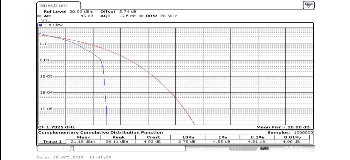
Band4-3MHz-QPSK-20175-1RB#0-PASS
