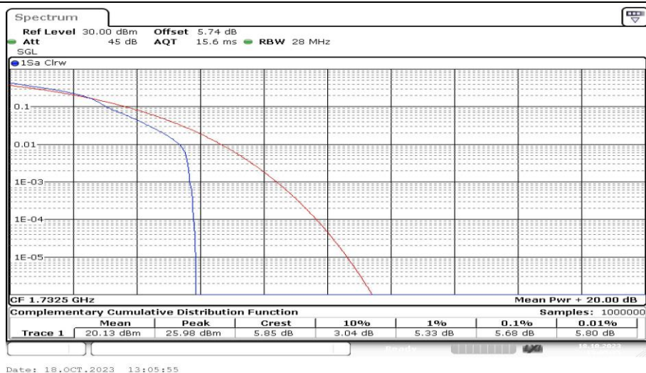
Band4-5MHz-16QAM-20175-1RB#0-PASS
