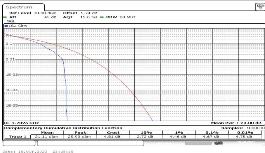
Band4-10MHz-QPSK-20175-1RB#0-PASS
