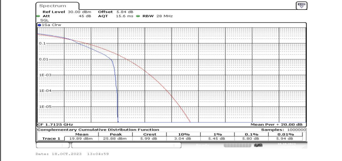
Band4-5MHz-16QAM-19975-1RB#0-PASS
