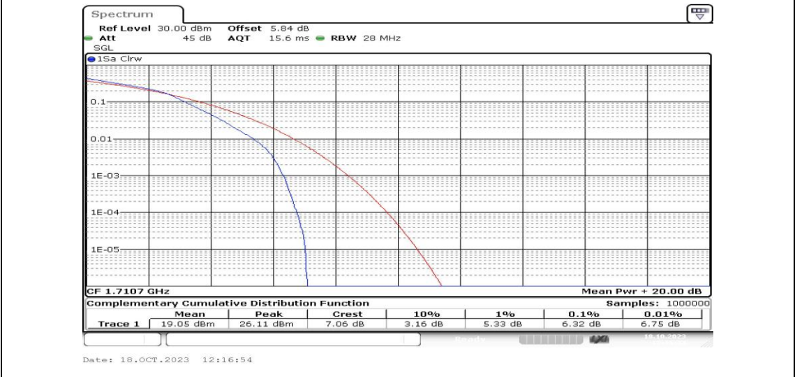
Band4-1.4MHz-16QAM-19957-6RB#0-PASS
