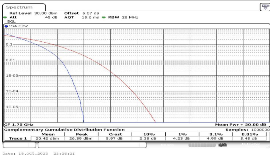
Band4-10MHz-QPSK-20350-50RB#0-PASS
