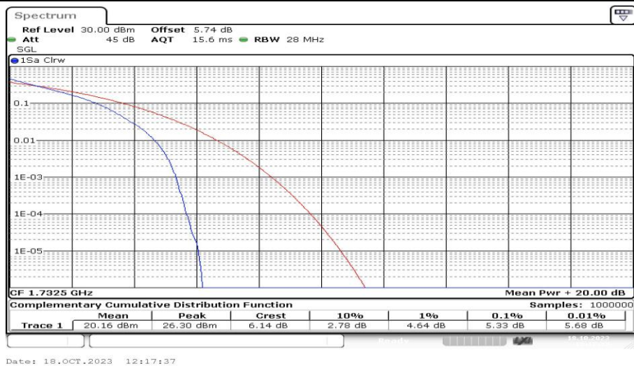
Band4-1.4MHz-QPSK-20175-6RB#0-PASS
