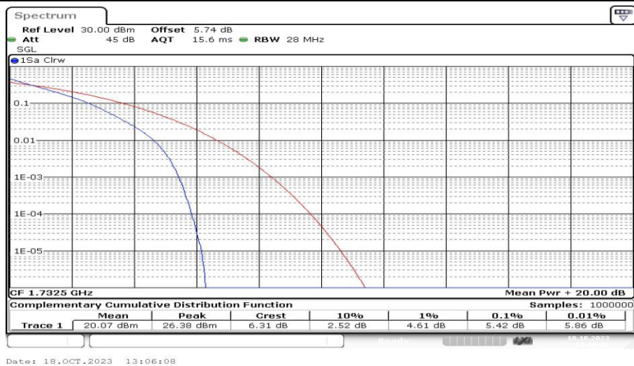
Band4-5MHz-QPSK-20175-25RB#0-PASS
