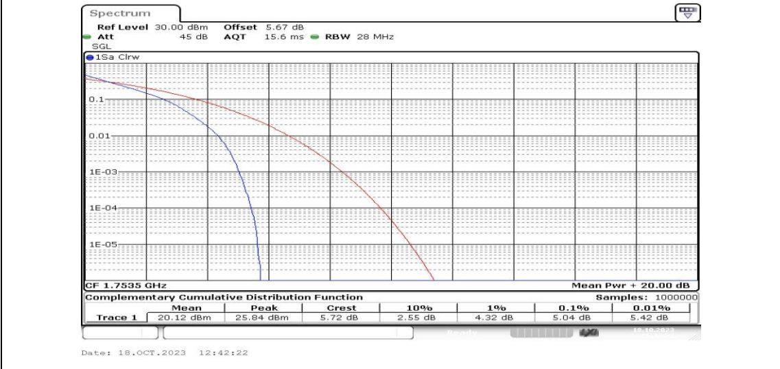
Band4-3MHz-QPSK-20385-15RB#0-PASS
