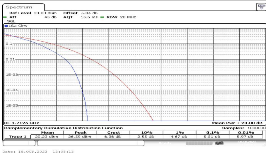
Band4-5MHz-QPSK-19975-25RB#0-PASS
