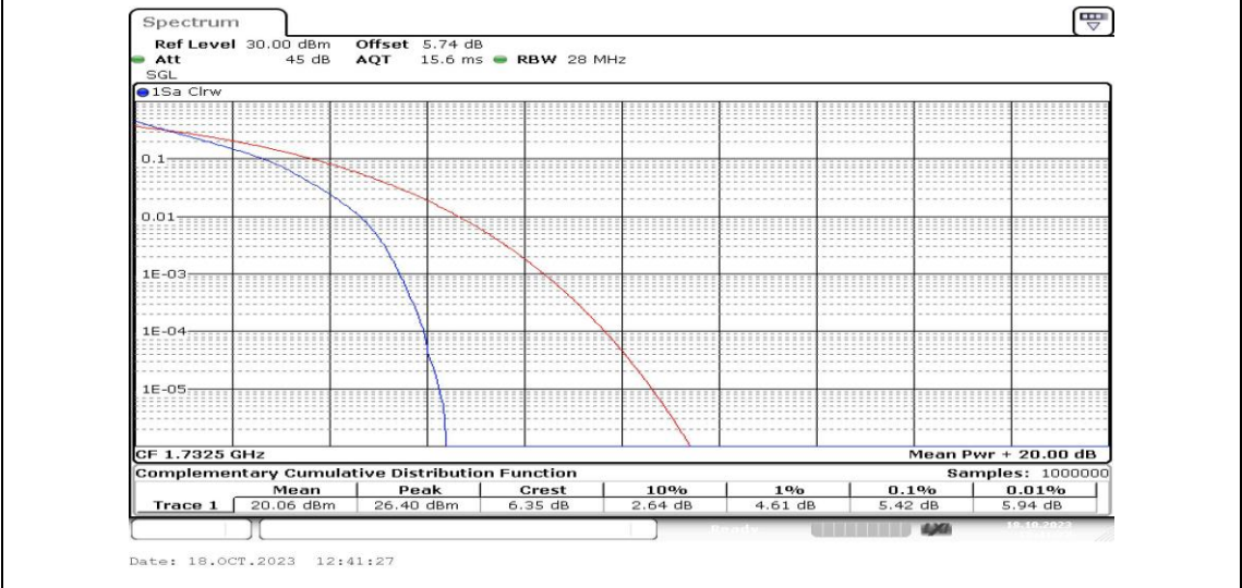
Band4-3MHz-QPSK-20175-15RB#0-PASS
