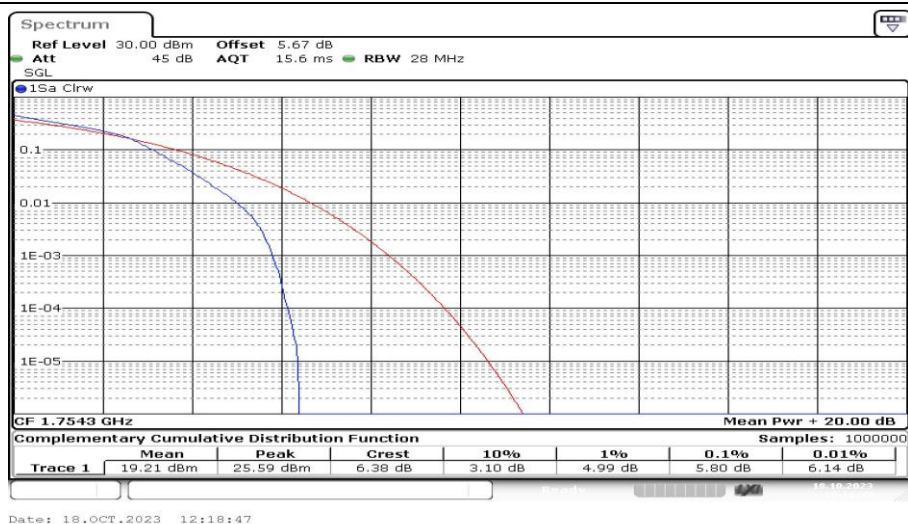
Band4-1.4MHz-16QAM-20393-6RB#0-PASS
