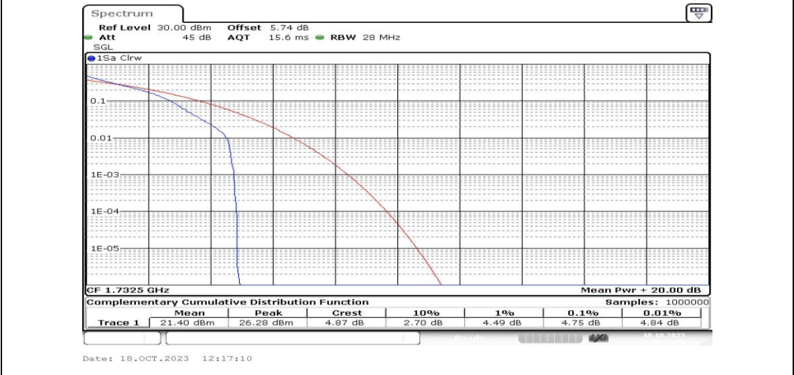
Band4-1.4MHz-QPSK-20175-1RB#0-PASS
