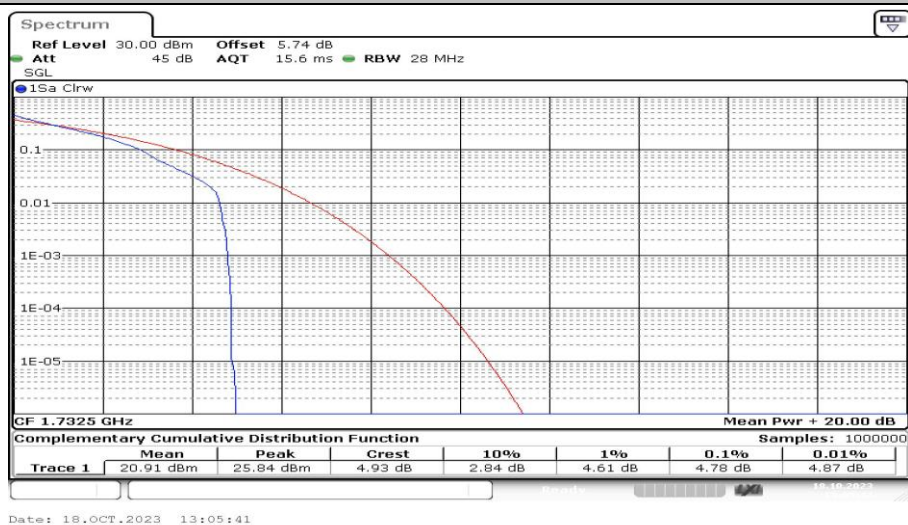
Band4-5MHz-QPSK-20175-1RB#0-PASS
