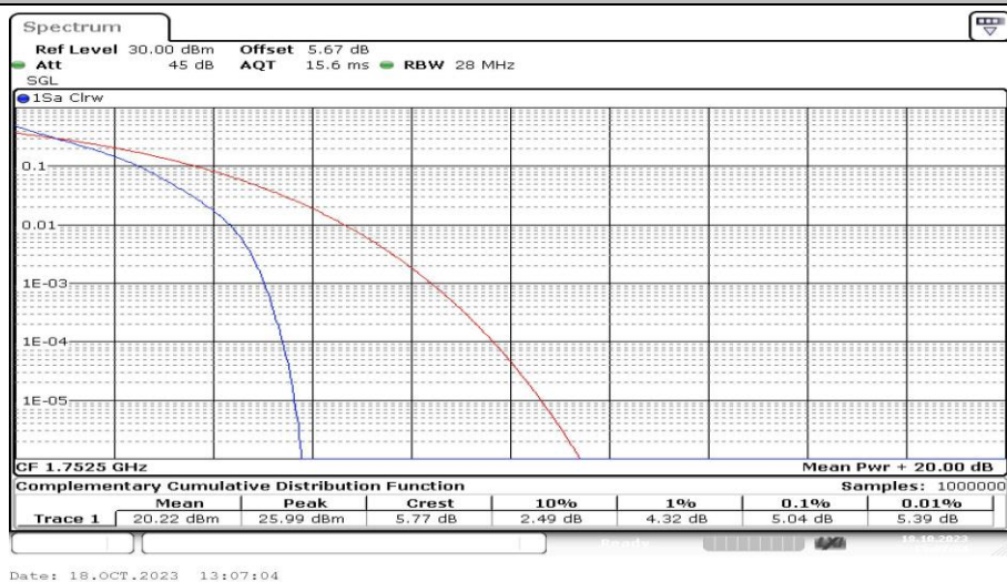
Band4-5MHz-QPSK-20375-25RB#0-PASS
