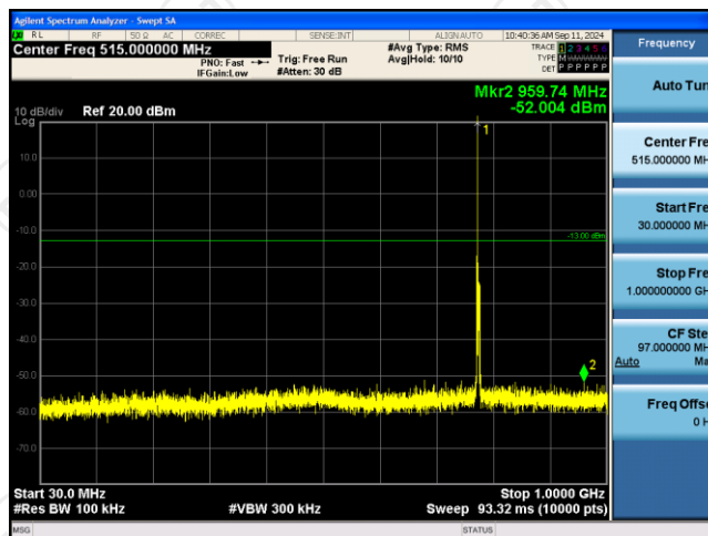
Band13-5MHz-16QAM-23205-1RB#0-Range1:30~1000MHz
