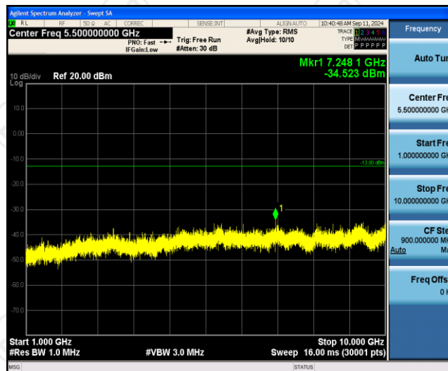
Band13-5MHz-16QAM-23205-1RB#0-Range2:1000~10000MHz
