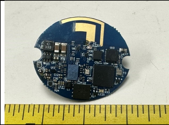
EUT PCBA1 top view
