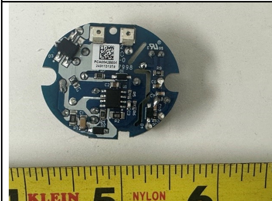
EUT PCBA2 bottom view
