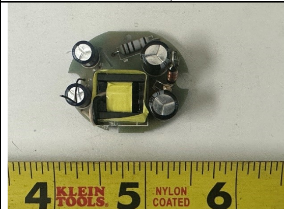
EUT PCBA2 top view
