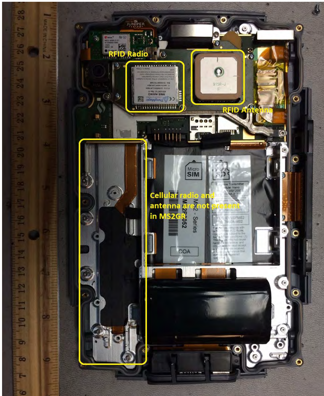
RFID radio and antenna in MS2GR
