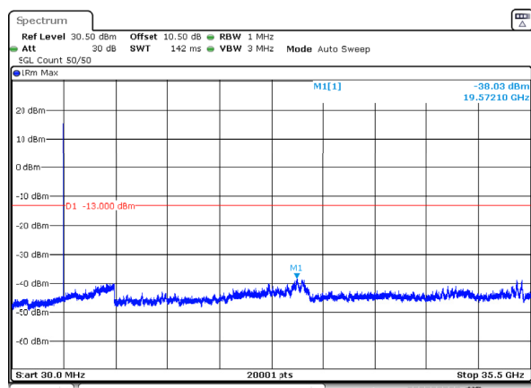
n78_1_20MHz_30kHz_3540MHz_DFT-s-OFDM QPSK_RB1@50 -38.03dBm
