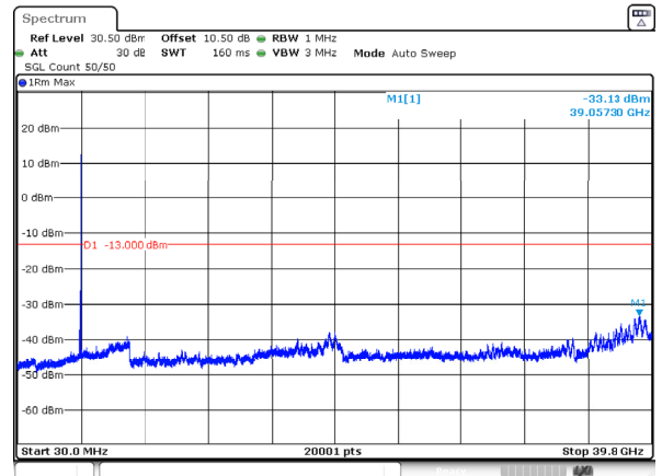
n77_3_100MHz_30kHz_3930MHz_DFT-s-OFDM QPSK_RB1@272 -33.13dBm
