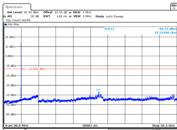
n78_1_30MHz_30kHz_3500MHz_DFT-s-OFDM QPSK_RB1@77 -38.27dBm
