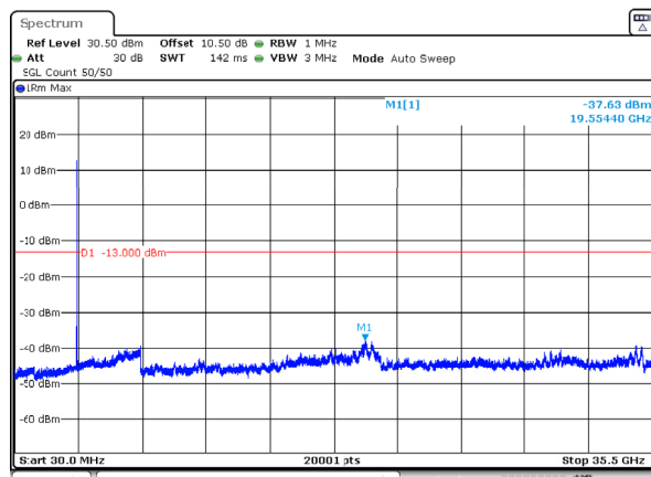
n78_1_50MHz_30kHz_3475MHz_DFT-s-OFDM QPSK_RB1@132 -37.63dBm
