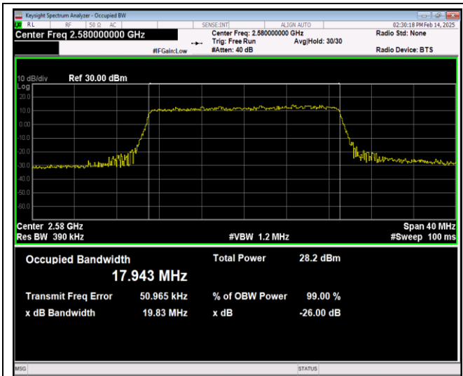
Band38-20MHz-64QAM-38150-100RB#0
