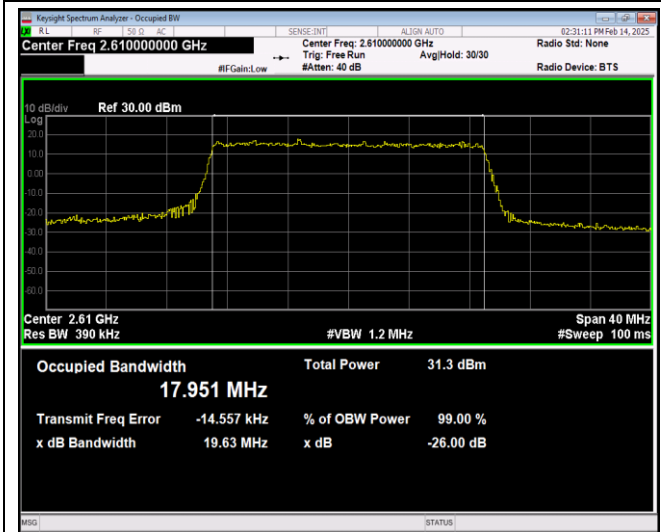
Band38-20MHz-16QAM-38000-100RB#0
