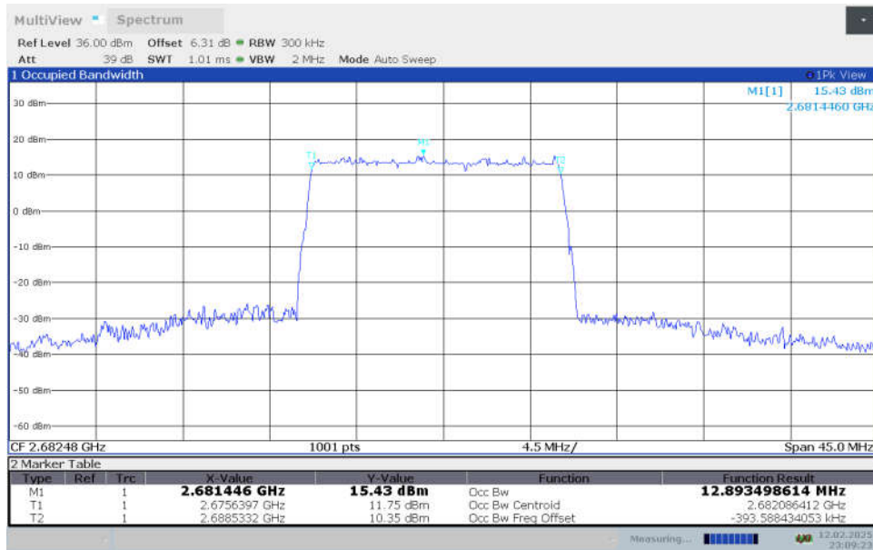
n41,15MHz Bandwidth,CP-QPSK (99% OBW)
