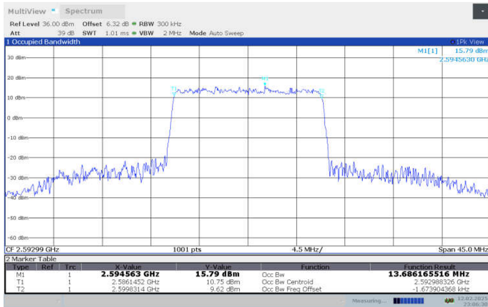
n41,15MHz Bandwidth,CP-256QAM (99% OBW)
