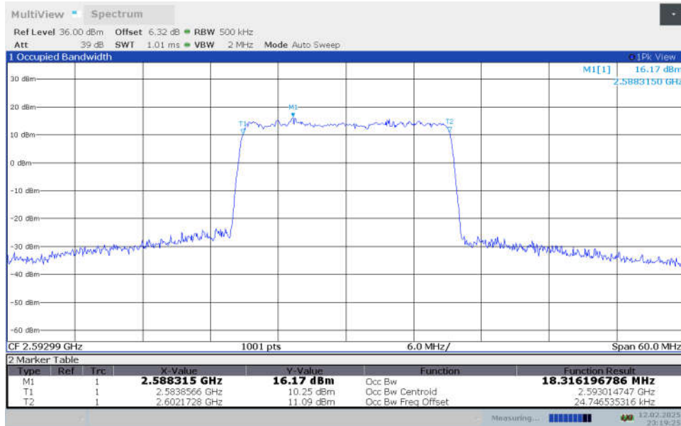
n41,20MHz Bandwidth,CP-256QAM (99% OBW)
