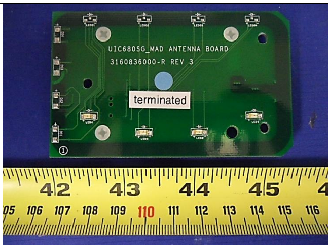
EUT-RFID Antenna Board Front View
