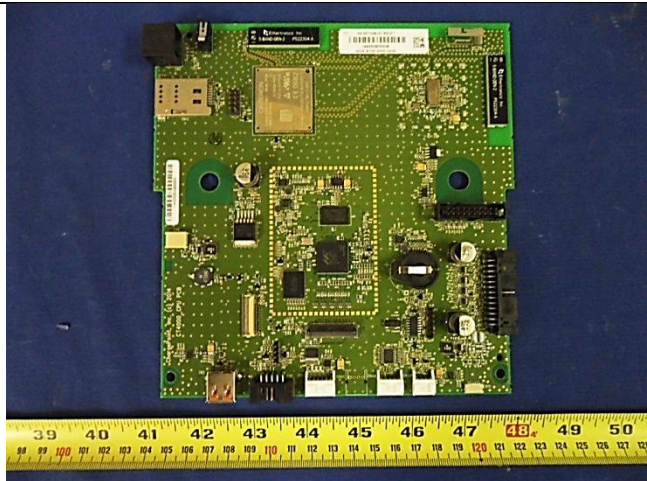
EUT-Wlan Board Front View
