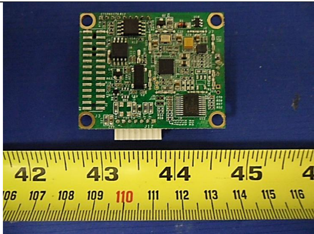
EUT-RFID Board Front View
