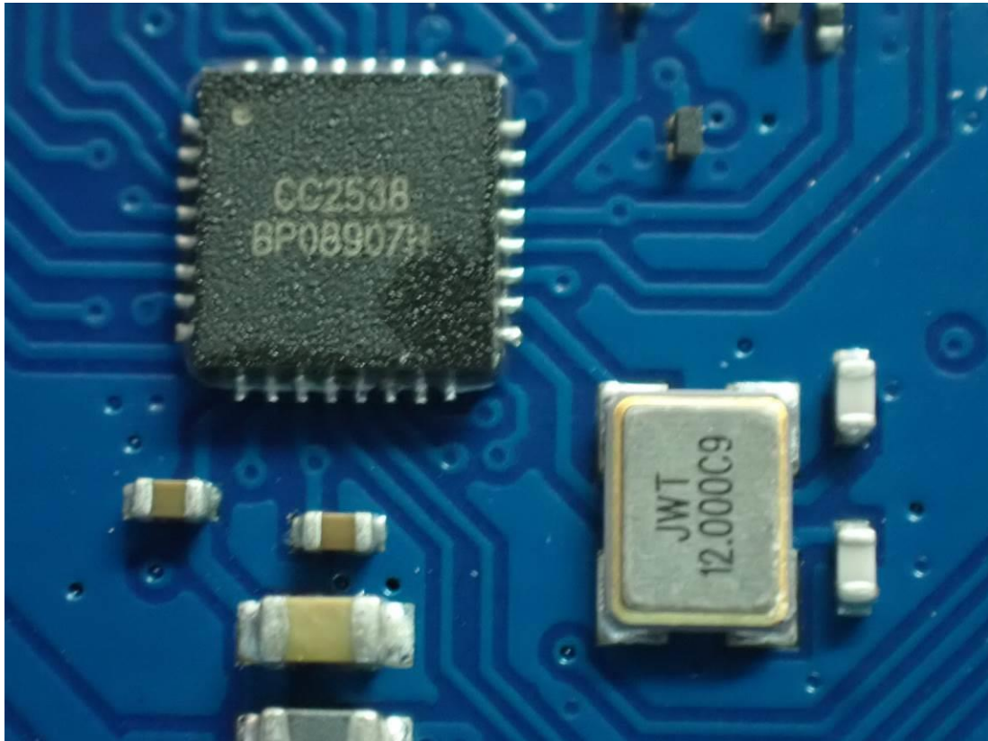
Figure 5 MCU: CC2538 / Oscillator View
