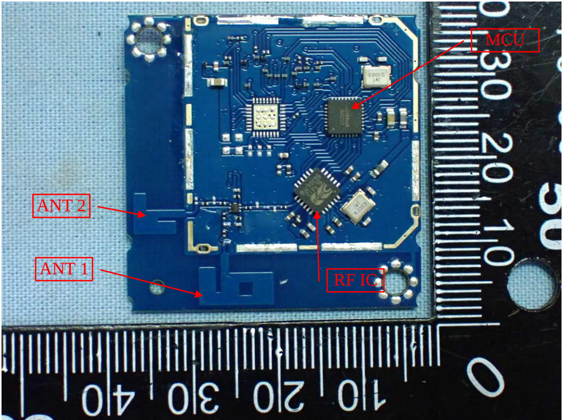
Figure 4 Antenna View
