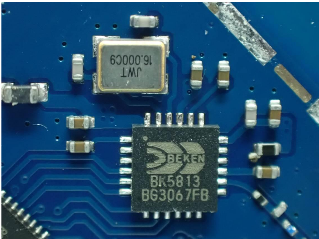
Figure 6 RF IC: BK5813 / Oscillator View
