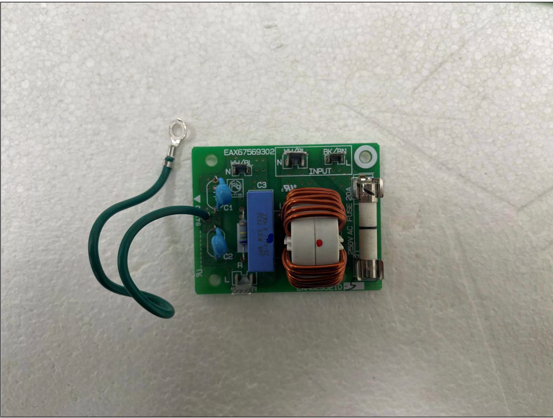
Front View of Fuse Board
