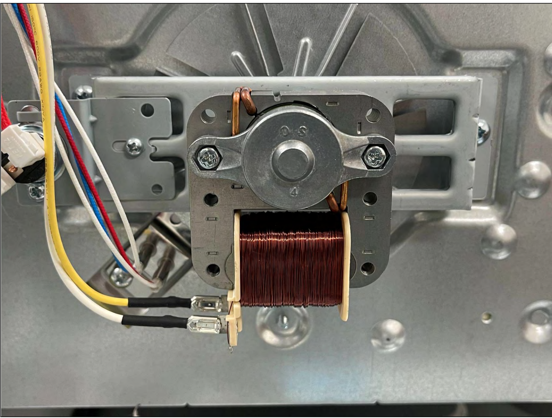
View of Fan Motor
