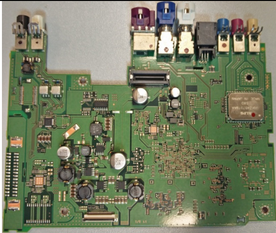
Powerboard TOP
