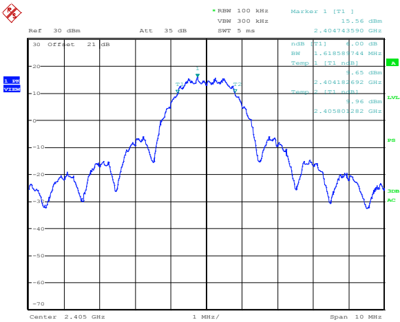
Figure 8.1-1: 6 dB bandwidth (2405 MHz)
