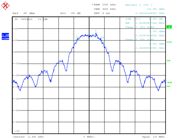
Figure 8.1-2: 6 dB bandwidth (2440 MHz)
