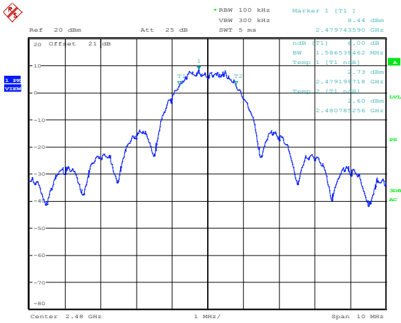
Figure 8.1-4: 6 dB bandwidth (2480 MHz)
