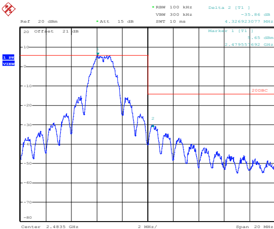
Figure 8.3-8: Upper band edge, Conducted (TX 2480 MHz) @ -14 dBm
