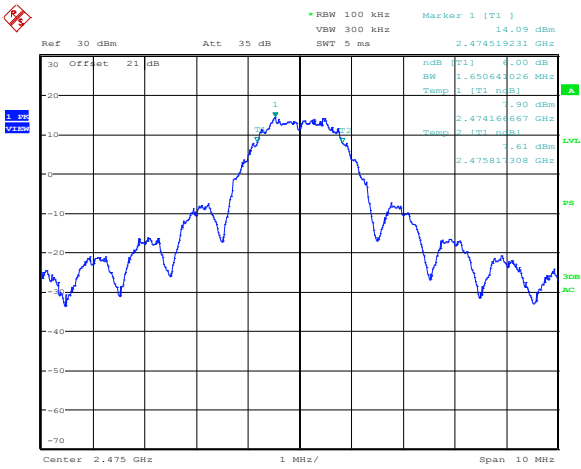
Figure 8.1-3: 6 dB bandwidth (2475 MHz)
