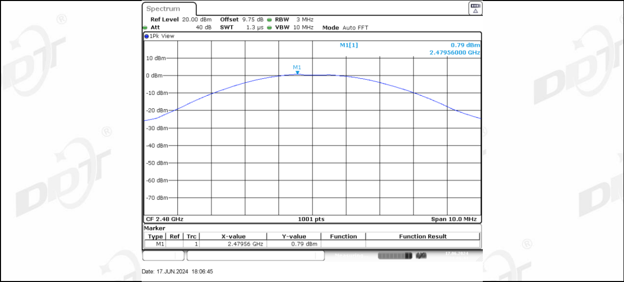
3DH5_Right side_2480
