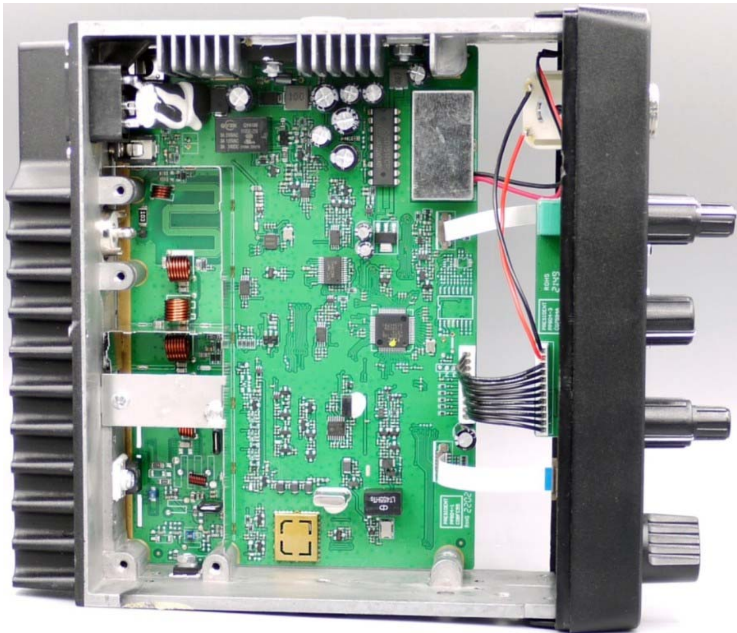
Figure E16.2 – Internal – Bottom Cover Removed
