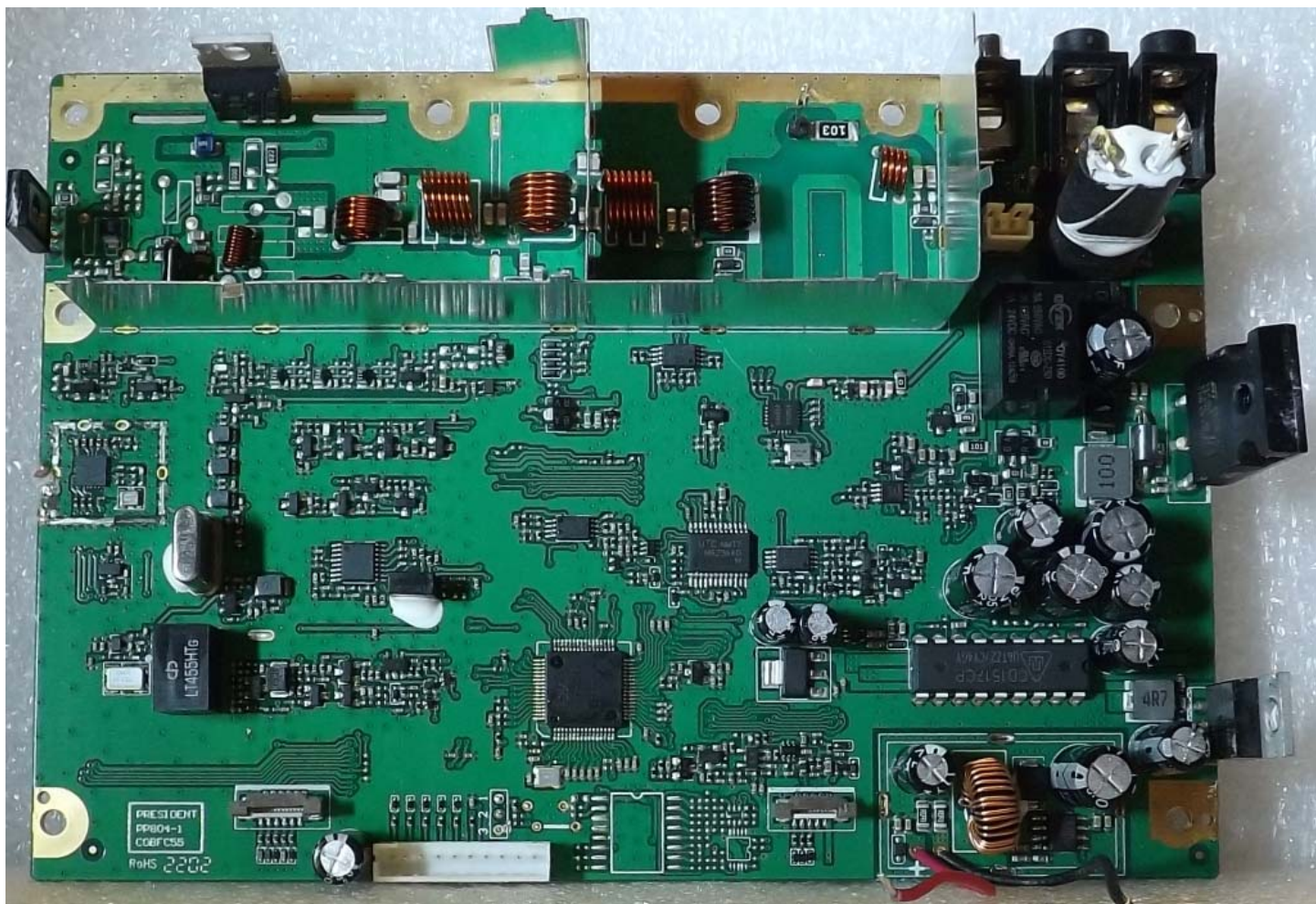
Figure E16.4 – Internal – PCB Top
