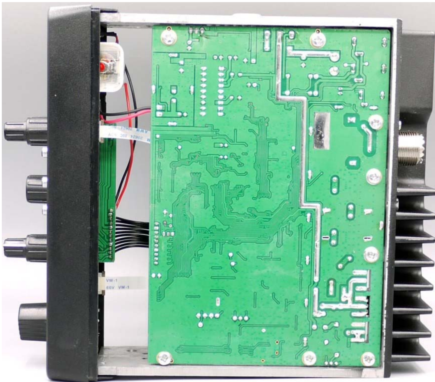
Figure E16.1 – Internal – Top Cover Removed
