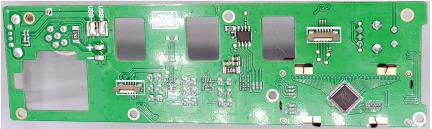
Figure E16.8 – Internal – Front Controls, Bottom View
