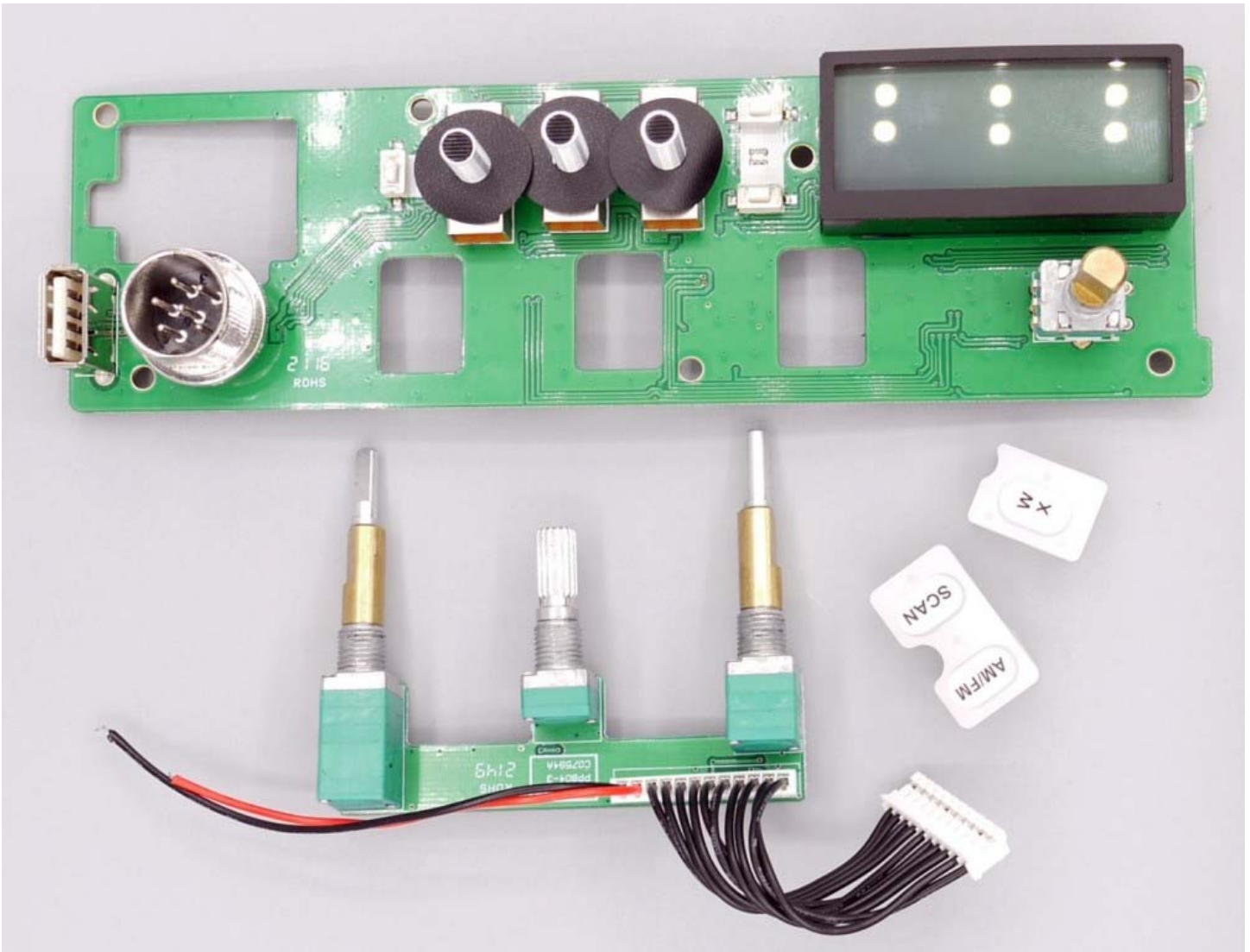
Figure E16.9 – Internal – Control Assembly
