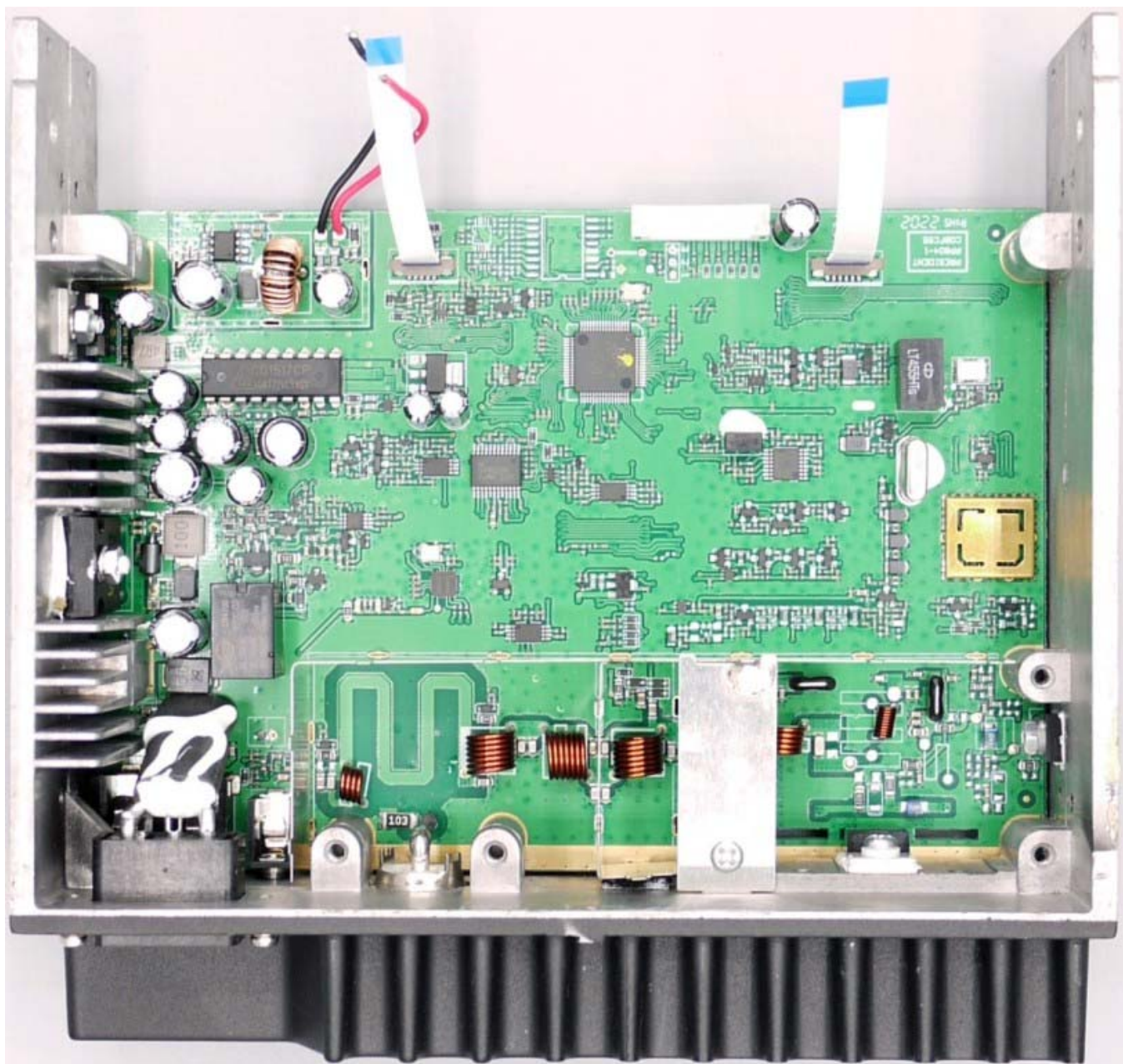
Figure E16.3 – Internal – Front Controls Removed
