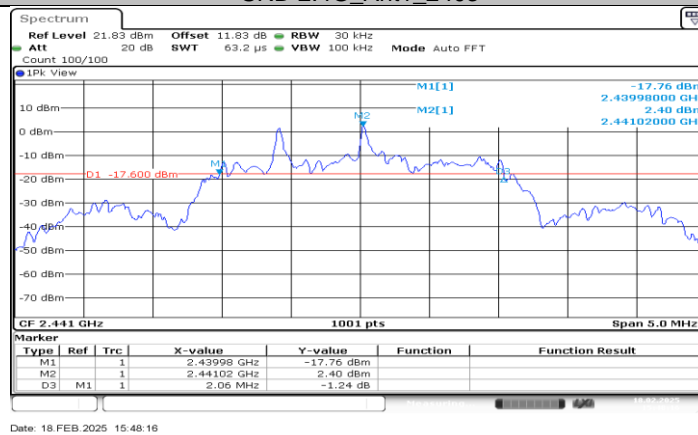
SRD 2.4G_Ant1_2441
