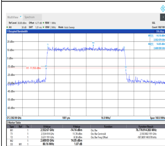
1-N41--30-80-M-3-DFT-16QAM-Outer_Full-2 16@0-Ant1-76.777-80.160-≤80-PASS
