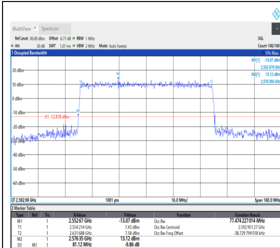
1-N41--30-80-M-7-CP-16QAM-Outer_Full-21 7@0-Ant1-77.474-81.120-≤80-PASS
