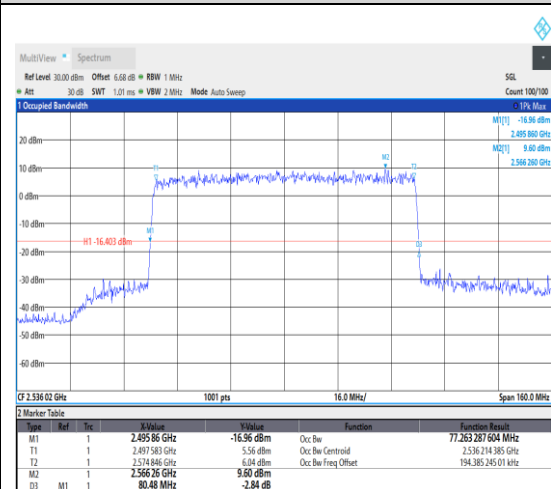
1-N41--30-80-L-9-CP-256QAM-Outer_Full-21 7@0-Ant1-77.263-80.480-≤80-PASS
