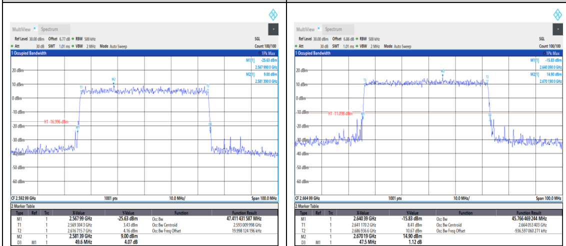
1-N41--30-50-M-9-CP-256QAM-Outer_Full-1 33@0-Ant1-47.411-49.600-≤50-PASS
