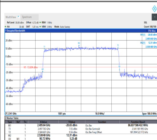
1-N41--30-90-L-6-CP-QPSK-Outter_Full-245@0-Ant1-86.838-90.720-≤90-PASS
