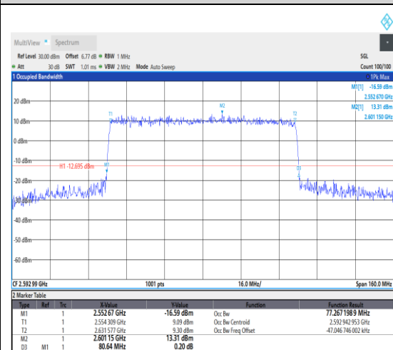
1-N41--30-80-M-6-CP-QPSK-Outer_Full-217 @0-Ant1-77.267-80.640-≤80-PASS
