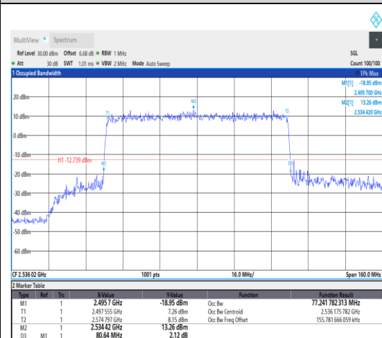
1-N41--30-80-L-7-CP-16QAM-Outer_Full-217 @0-Ant1-77.242-80.640-≤80-PASS
