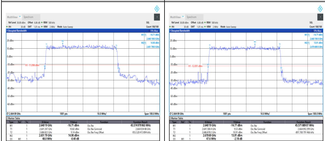
1-N41--30-50-H-2-DFT-PI2BPSK-Outer_Full- 128@0-Ant1-45.575-48.000-≤50-PASS
