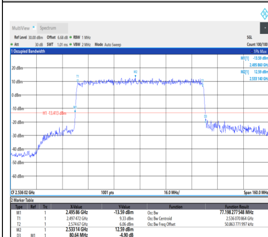
1-N41--30-80-L-8-CP-64QAM-Outer_Full-217 @0-Ant1-77.198-80.640-≤80-PASS
