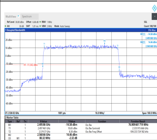
1-N41--30-80-L-3-DFT-16QAM-Outer_Full-21 6@0-Ant1-76.91-80.320-≤80-PASS
