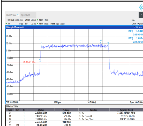
1-N41--30-80-L-6-CP-QPSK-Outer_Full-217 @0-Ant1-25.676-27.200-≤80-PASS
