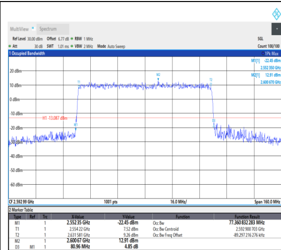
1-N41--30-80-M-8-CP-64QAM-Outer_Full-21 7@0-Ant1-77.361-80.960-≤80-PASS
