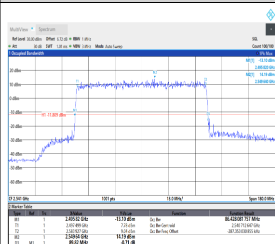
1-N41--30-90-L-4-DFT-64QAM-Outter_Full-243@0-Ant1-86.428-89.820-≤90-PASS
