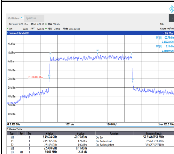
1-N41--30-60-L-9-CP-256QAM-Outer_Full-16 2@0-Ant1-57.815-59.640-≤60-PASS
