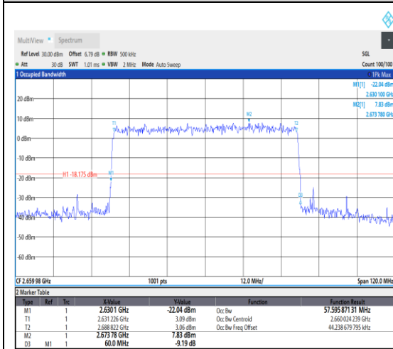
1-N41--30-60-H-9-CP-256QAM-Outer_Full-1 62@0-Ant1-57.596-60.000-≤60-PASS
