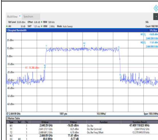
1-N41--30-50-H-8-CP-64QAM-Outer_Full-13 3@0-Ant1-47.409-49.400-≤50-PASS
