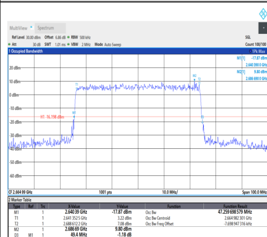
1-N41--30-50-H-9-CP-256QAM-Outer_Full-1 33@0-Ant1-47.26-49.400-≤50-PASS
