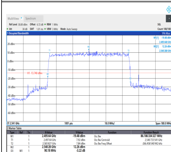
1-N41--30-90-L-5-DFT-256QAM-Outter_Full-243@0-Ant1-86.186-90.180-≤90-PASS
