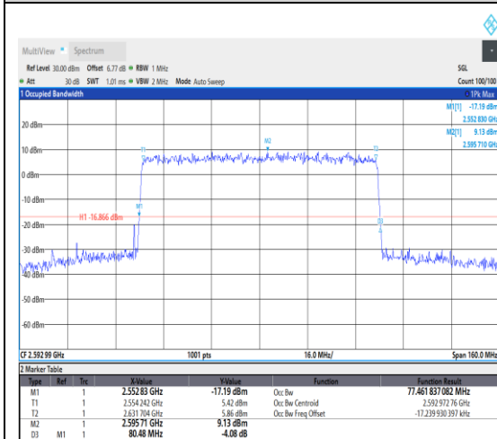
1-N41--30-80-M-9-CP-256QAM-Outer_Full-2 17@0-Ant1-77.462-80.480-≤80-PASS
