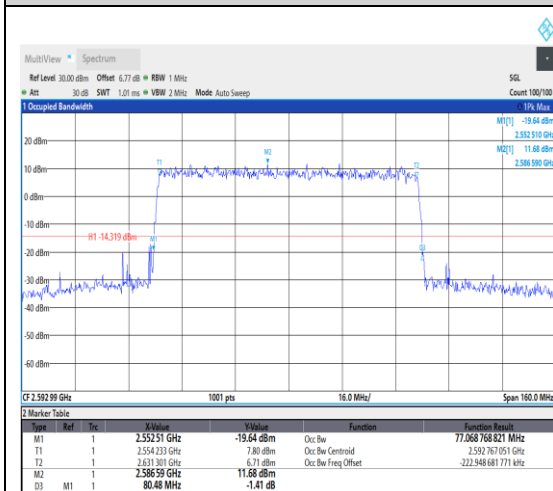
1-N41--30-80-M-5-DFT-256QAM-Outer_Full- 216@0-Ant1-77.069-80.480-≤80-PASS
