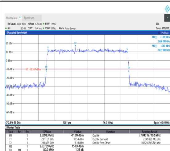
1-N41--30-80-H-3-DFT-16QAM-Outer_Full-2 16@0-Ant1-77.04-80.000-≤80-PASS
