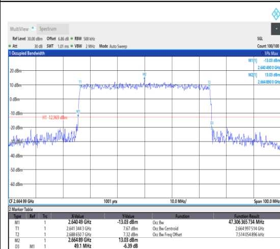
1-N41--30-50-H-7-CP-16QAM-Outer_Full-13 3@0-Ant1-47.306-49.100-≤50-PASS
