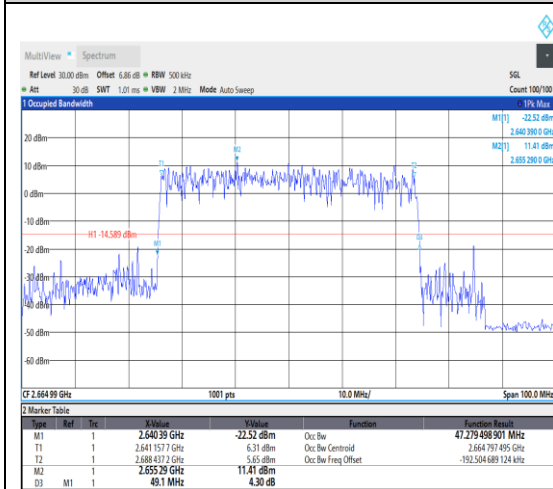
1-N41--30-50-H-6-CP-QPSK-Outer_Full-133 @0-Ant1-47.279-49.100-≤50-PASS
