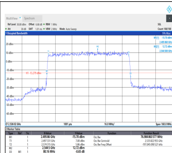
1-N41--30-80-L-5-DFT-256QAM-Outer_Full-2 16@0-Ant1-76.985-80.160-≤80-PASS
