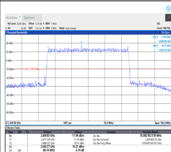
1-N41--30-80-H-1-DFT-QPSK-Outer_Full-21 6@0-Ant1-76.983-80.160-≤80-PASS
