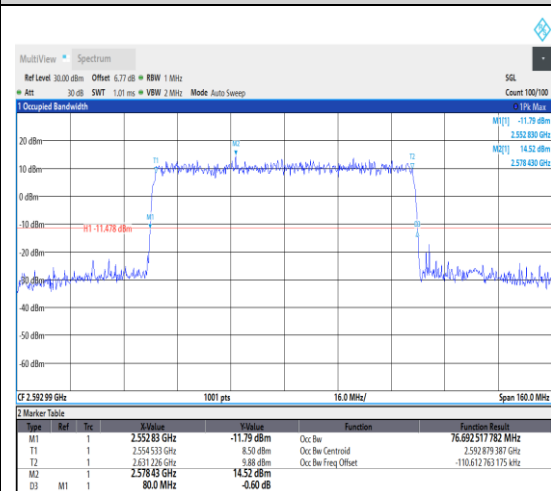
1-N41--30-80-M-4-DFT-64QAM-Outer_Full-2 16@0-Ant1-76.693-80.000-≤80-PASS
