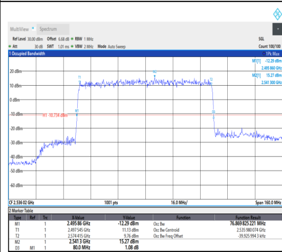
1-N41--30-80-L-1-DFT-QPSK-Outer_Full-216 @0-Ant1-76.87-80.000-≤80-PASS
