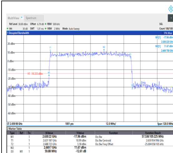
1-N41--30-60-H-7-CP-16QAM-Outer_Full-16 2@0-Ant1-57.536-59.880-≤60-PASS
