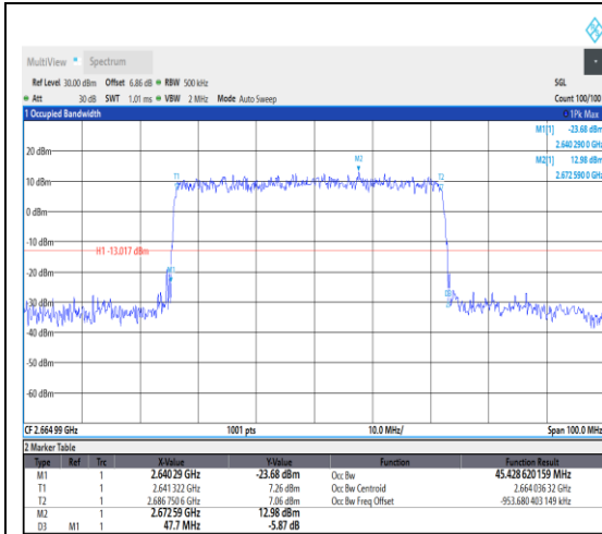
1-N41--30-50-H-4-DFT-64QAM-Outer_Full-1 28@0-Ant1-45.429-47.700-≤50-PASS
