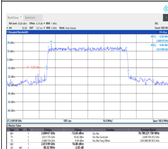
1-N41--30-80-H-2-DFT-PI2BPSK-Outer_Full-216@0-Ant1-76.78-80.320-≤80-PASS
