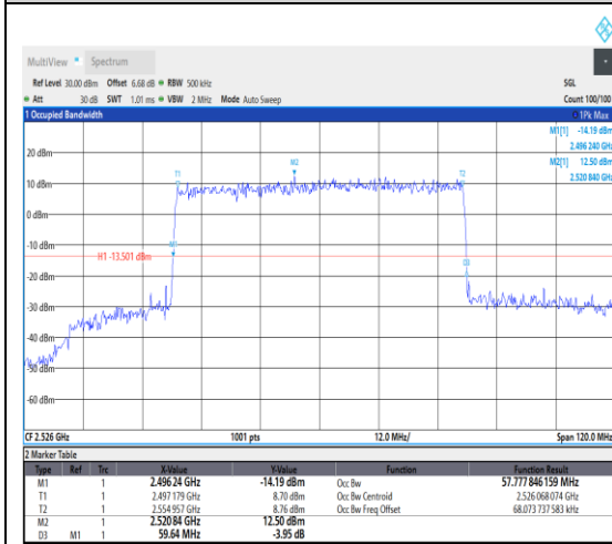
1-N41--30-60-L-3-DFT-16QAM-Outer_Full-162@0-Ant1-57.778-59.640-≤60-PASS
