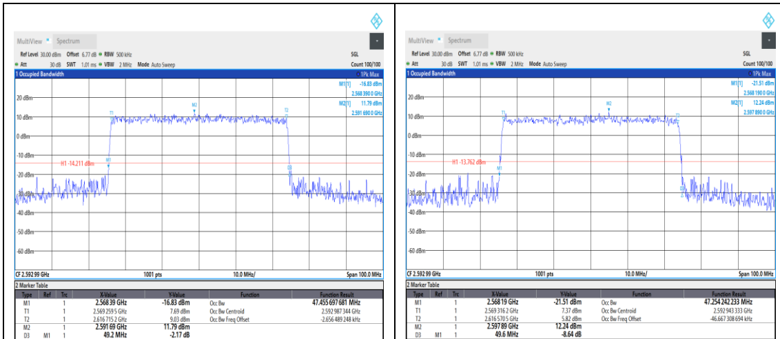
1-N41--30-50-M-7-CP-16QAM-Outer_Full-13 3@0-Ant1-47.456-49.200-≤50-PASS
