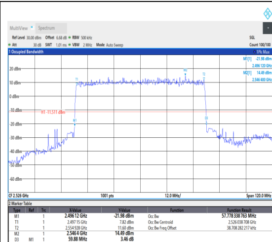
1-N41--30-60-L-2-DFT-PI2BPSK-Outer_Full-162@0-Ant1-57.778-59.880-≤60-PASS
