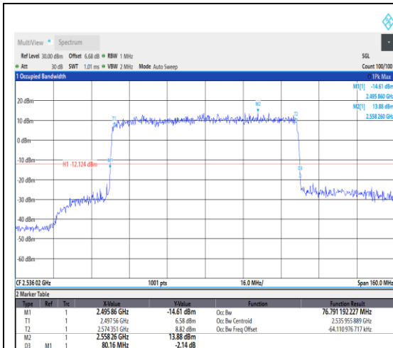
1-N41--30-80-L-4-DFT-64QAM-Outer_Full-21 6@0-Ant1-76.791-80.160-≤80-PASS
