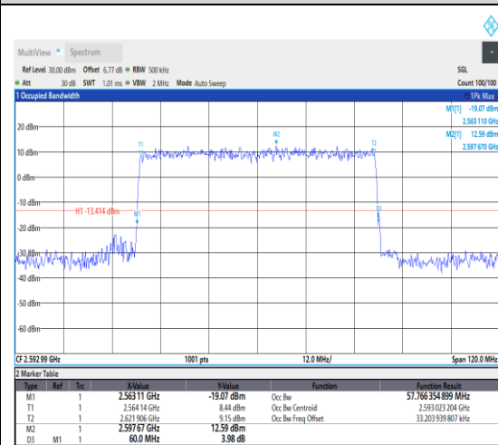
1-N41--30-60-M-1-DFT-QPSK-Outer_Full-16 2@0-Ant1-57.766-60.000-≤60-PASS
