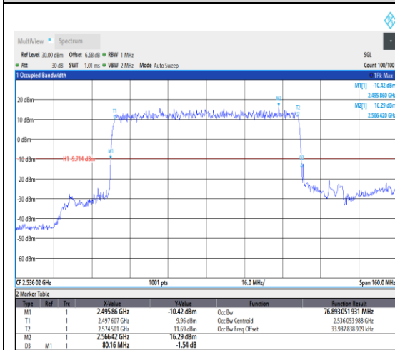
1-N41--30-80-L-2-DFT-PI2BPSK-Outer_Full-216@0-Ant1-76.893-80.160-≤80-PASS
