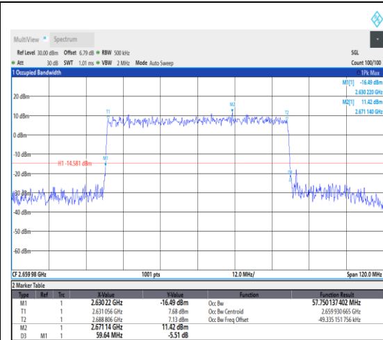
1-N41--30-60-H-8-CP-64QAM-Outer_Full-16 2@0-Ant1-57.75-59.640-≤60-PASS
