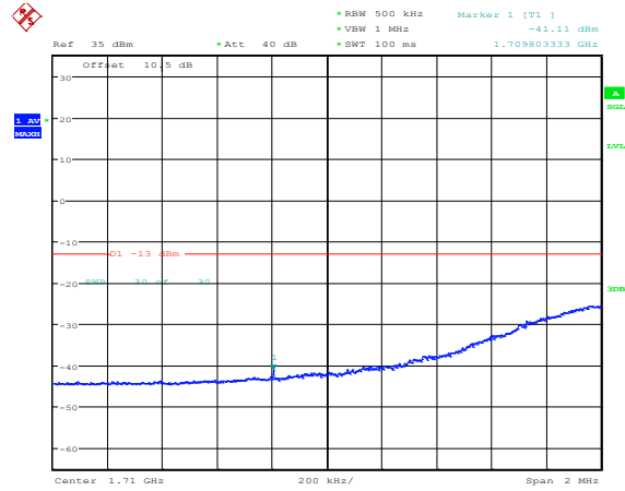
Band4-20MHz-16QAM-20050-100RB#0
