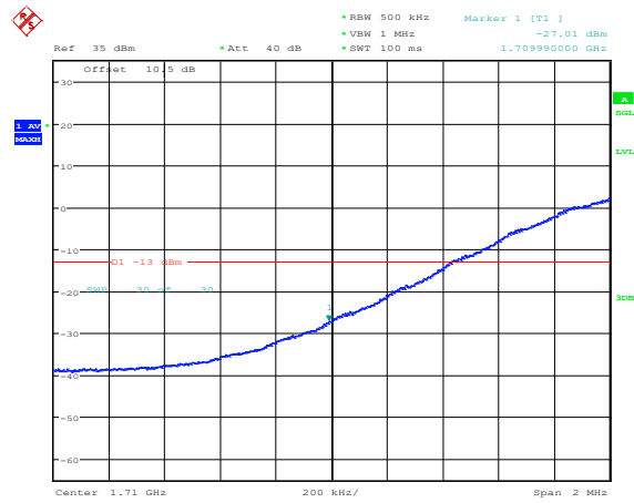
Band4-20MHz-16QAM-20050-100RB#0
