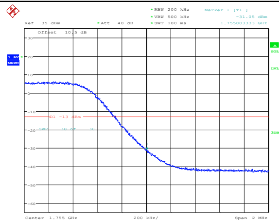
Band4-10MHz-QPSK-20350-50RB#0
