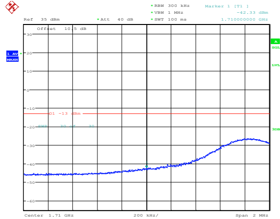
Band4-15MHz-QPSK-20025-75RB#0
