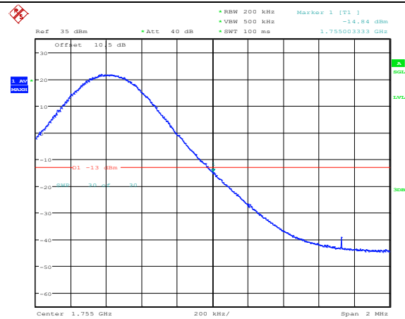
Band4-10MHz-QPSK-20350-50RB#0
