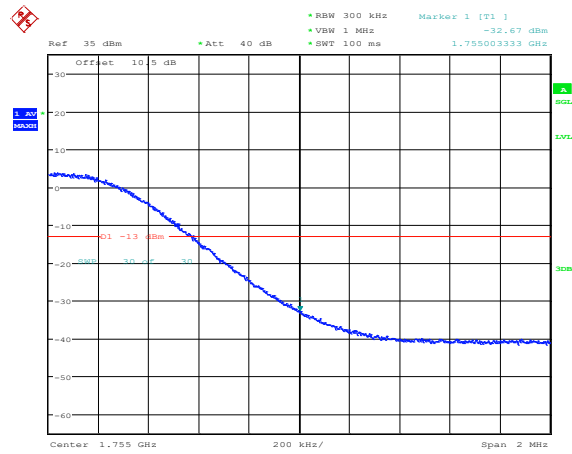
Band4-15MHz-16QAM-20325-75RB#0
