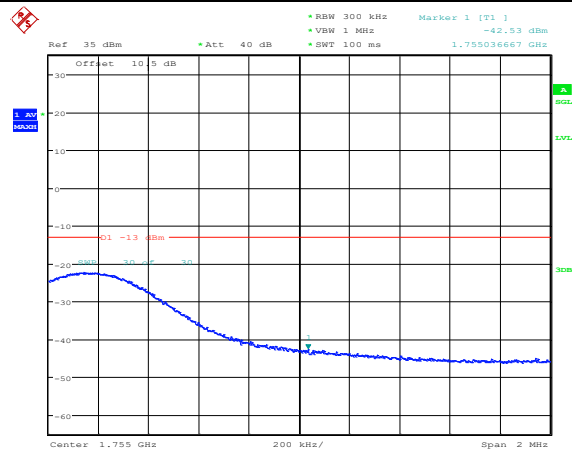
Band4-15MHz-QPSK-20325-1RB#0
