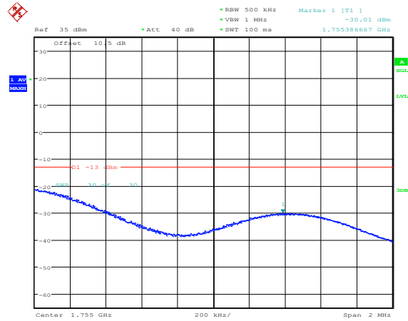
Band4-20MHz-16QAM-20300-1RB#0
