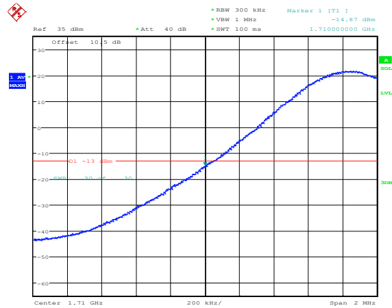
Band4-15MHz-16QAM-20025-1RB#0
