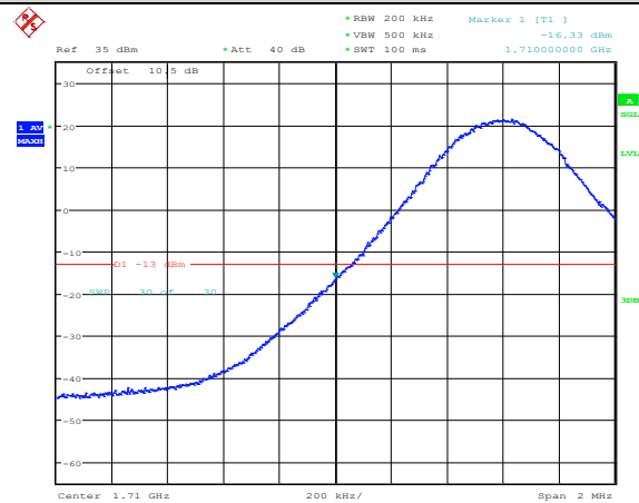
Band4-10MHz-16QAM-20000-1RB#0
