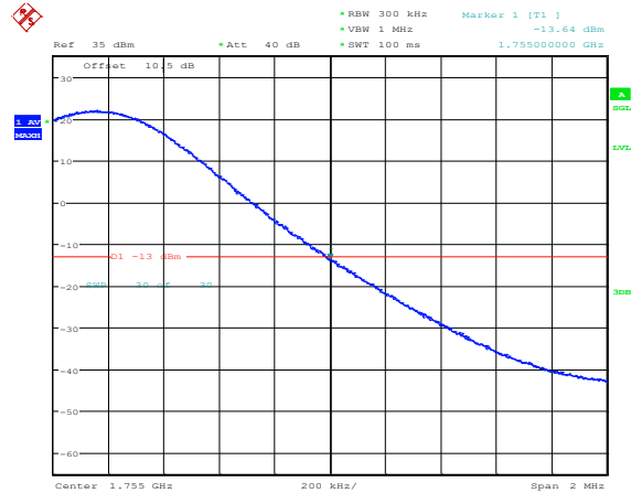
Band4-15MHz-QPSK-20325-75RB#0
