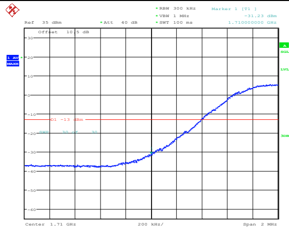
Band4-15MHz-QPSK-20025-75RB#0
