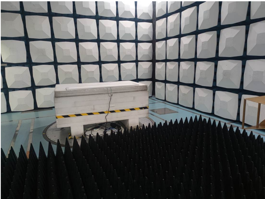
Radiated Emissions Above 1G side View
