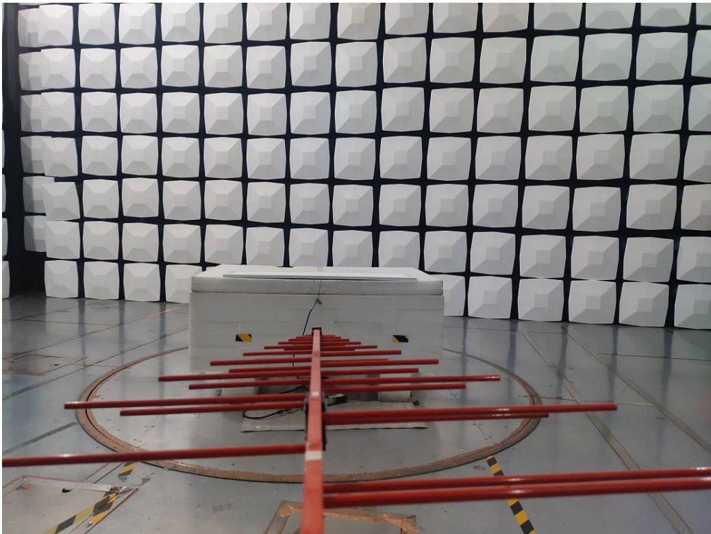
Radiated Emissions Below 1G side View
