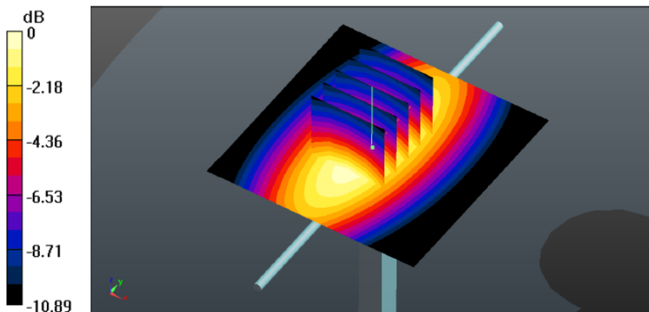
System Performance Check 835MHz Head 250mW
