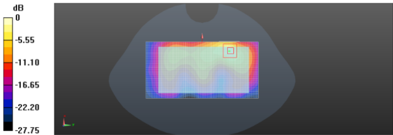
Rear side (WLAN 802.11b)
