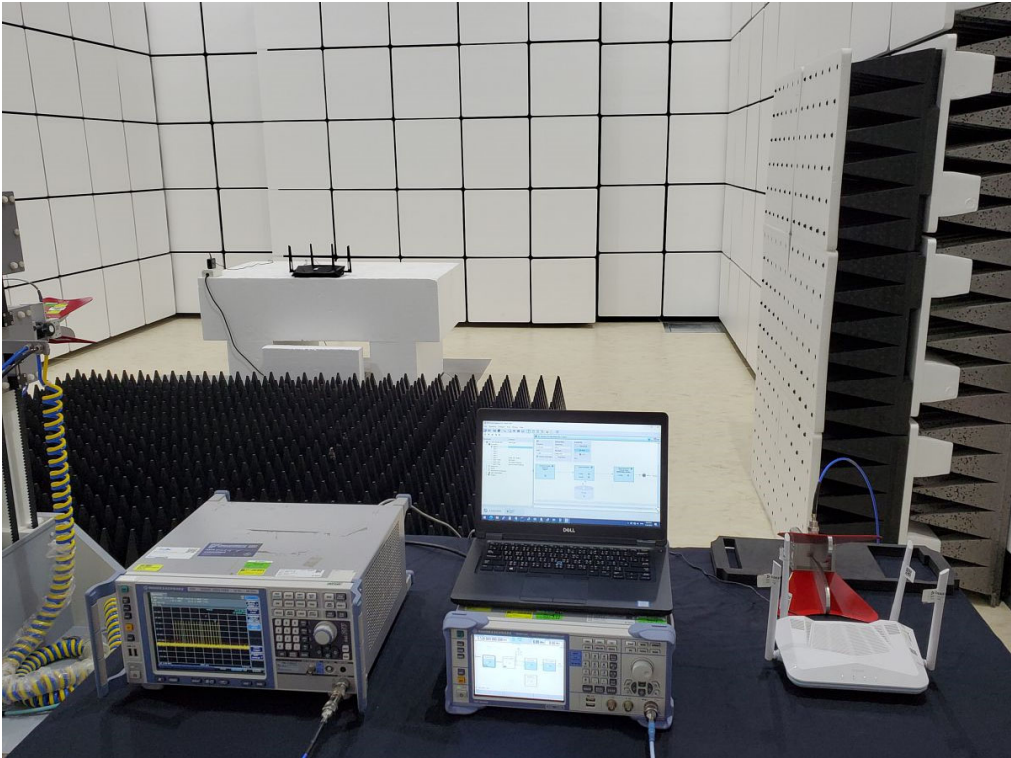
DFS Set-up Photo: Slave Mode
