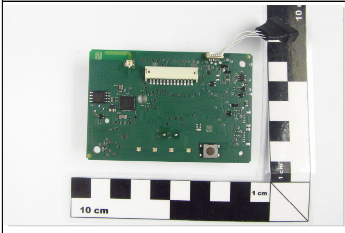
PCB top view
