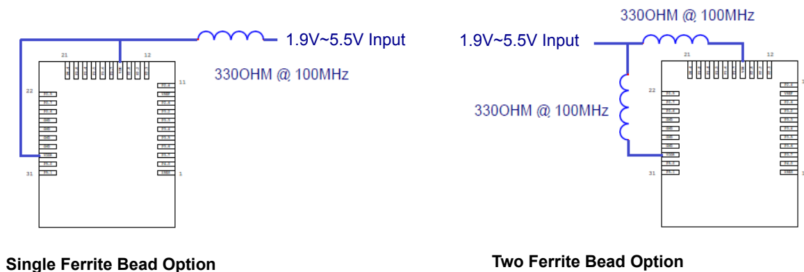
Figure 5. Recommended Host Schematic Options for a Single Supply Option
