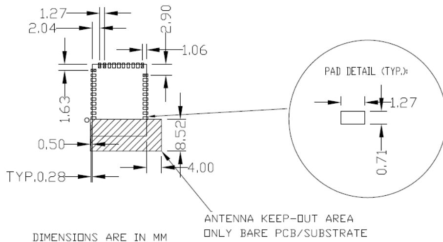
Figure 4. Recommended Host PCB Keep Out Area Around the CYBLE-212019-00 Antenna
