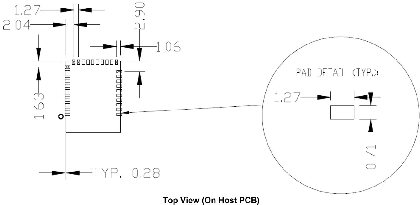
Figure 3. Recommended PCB Layout Pattern for CYBLE-212019-00 Module
