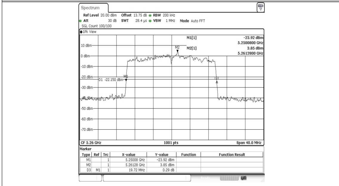
11AX20SISO-Ant1-5260
