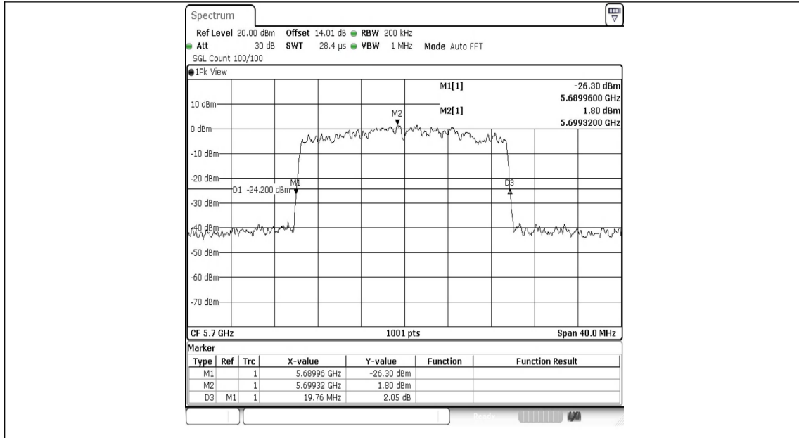
11AX20SISO-Ant1-5700
