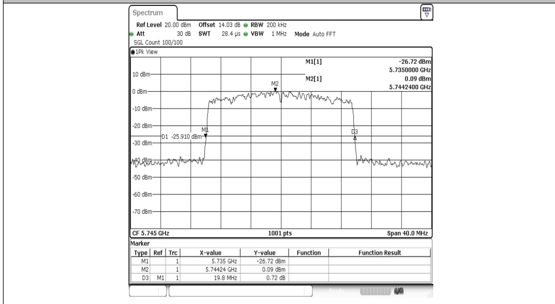
11AX20SISO-Ant1-5745
