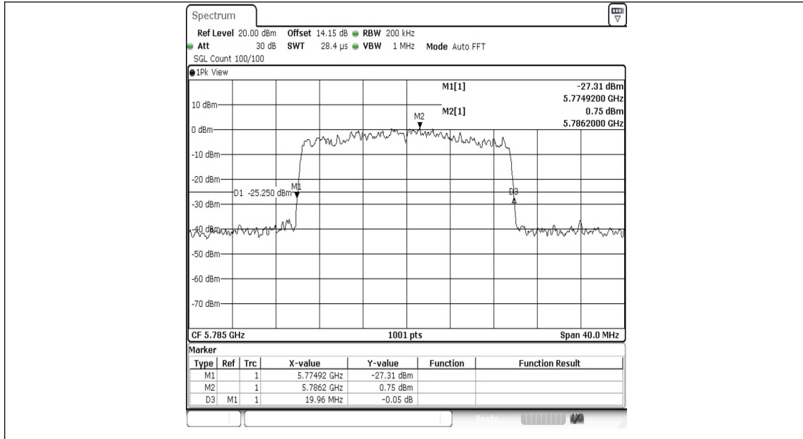
11AX20SISO-Ant1-5785
