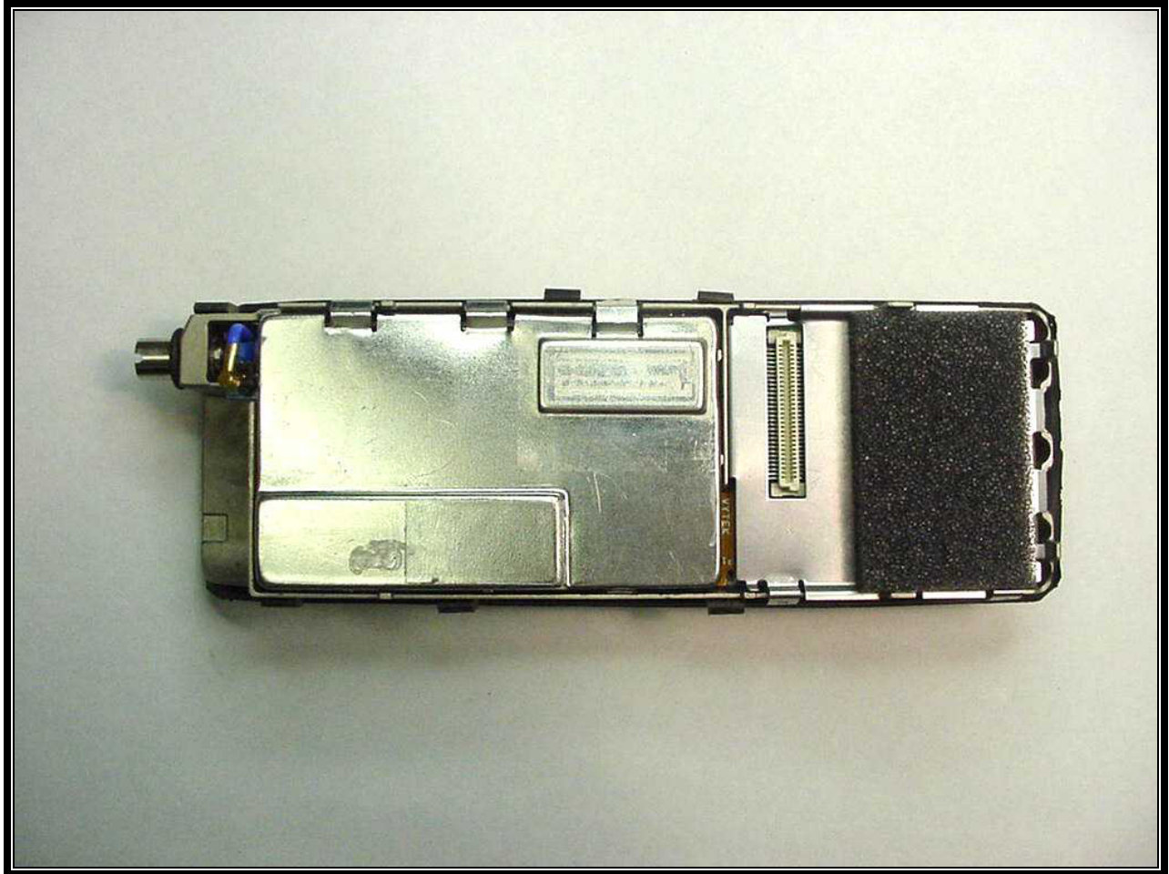
PHOTOGRAPH 10: CHASSIS WITH SHIELDS
