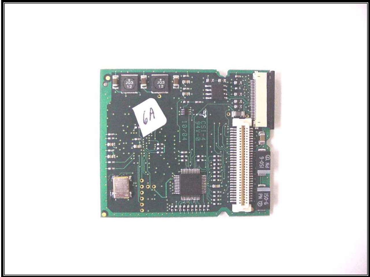
PHOTOGRAPH 12: LOGIC BOARD TOP VIEW
