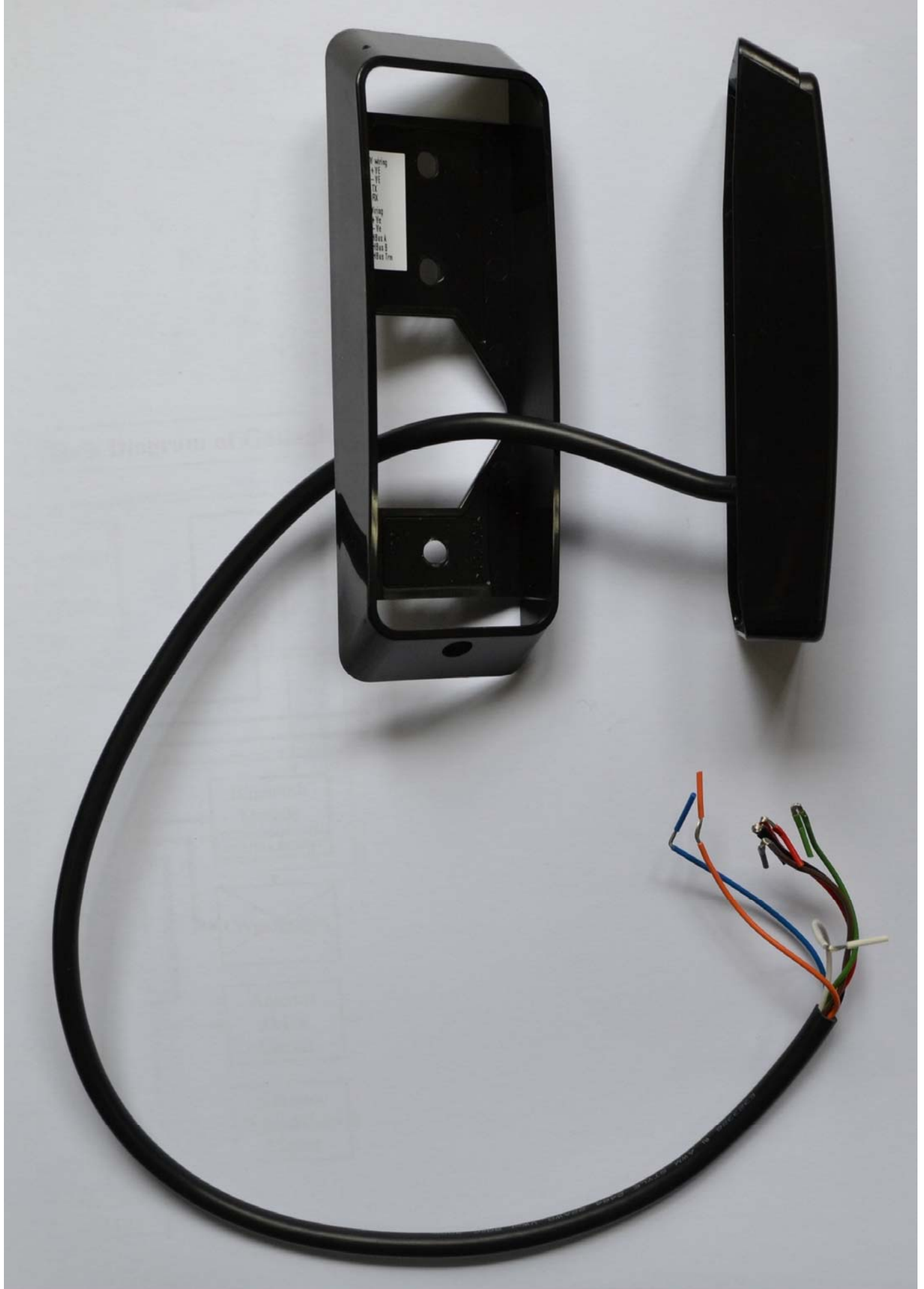
T15 Mifare Reader - Side View
