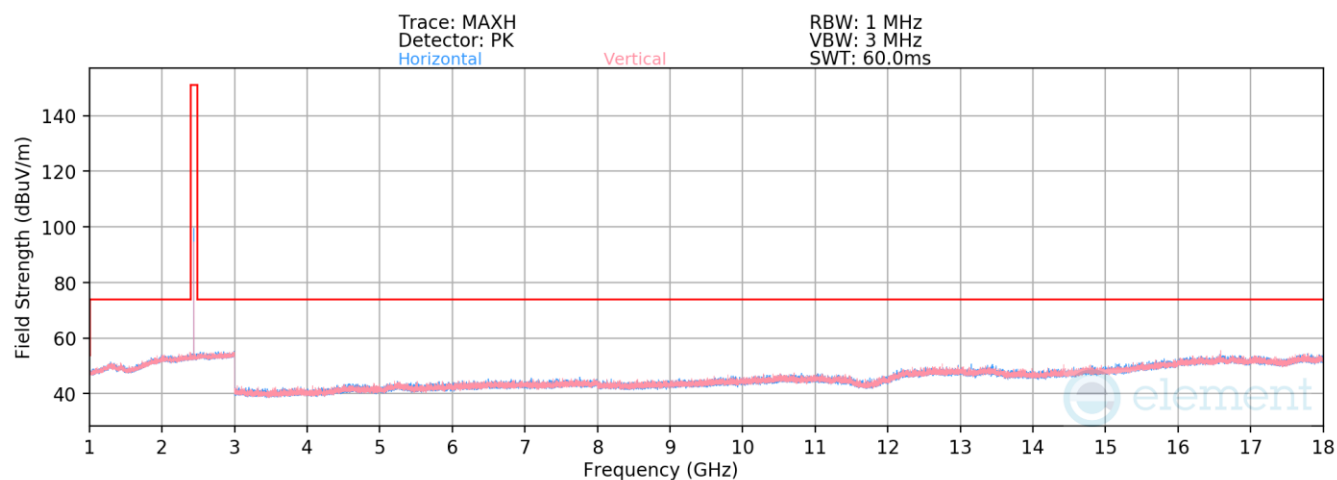
Plot 7-110. Radiated Spurious Emissions 1-18GHz Antenna WF2 (1Mbps, iPA – Ch. 19)
