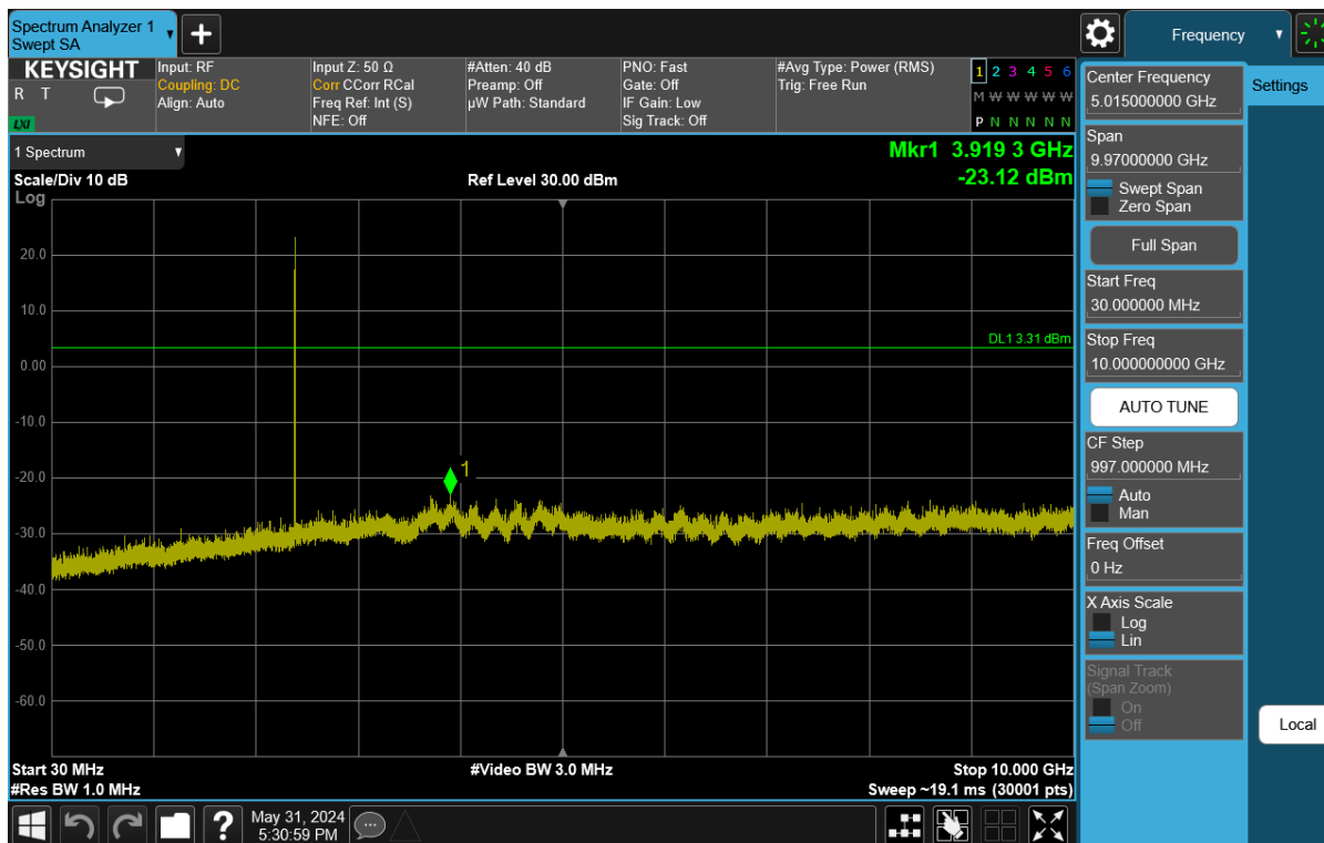
Plot 7-91. Conducted Spurious Plot Antenna WF7 (Bluetooth (LE), 1Mbps, ePA – Ch. 0)
