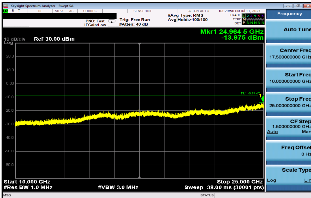
Plot 7-98. Conducted Spurious Plot Antenna WF2 (Bluetooth (LE), 1Mbps, iPA – Ch. 0)
