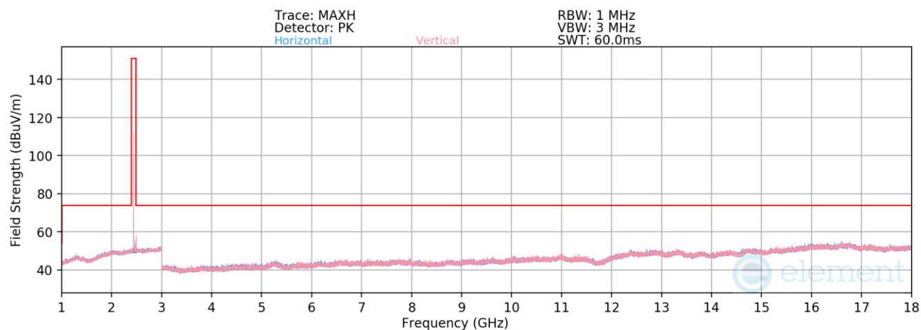
Plot 7-107. Radiated Spurious Emissions 1-18GHz Antenna WF7 (1Mbps, ePA – Ch. 19)
