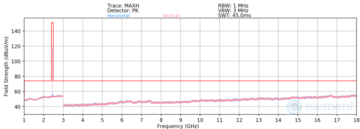
Plot 7-104. Radiated Spurious Emissions 1-18GHz Antenna WF8 (1Mbps, ePA – Ch. 19)
