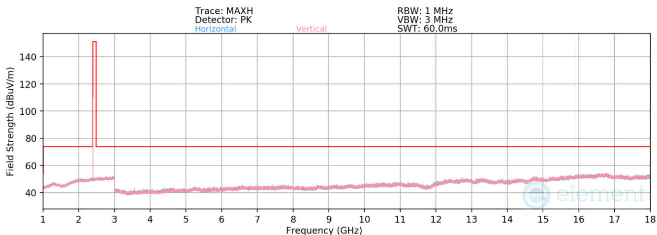
Plot 7-106. Radiated Spurious Emissions 1-18GHz Antenna WF7 (1Mbps, ePA – Ch. 0)
