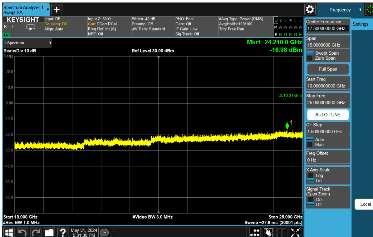
Plot 7-92. Conducted Spurious Plot Antenna WF7 (Bluetooth (LE), 1Mbps, ePA – Ch. 0)
