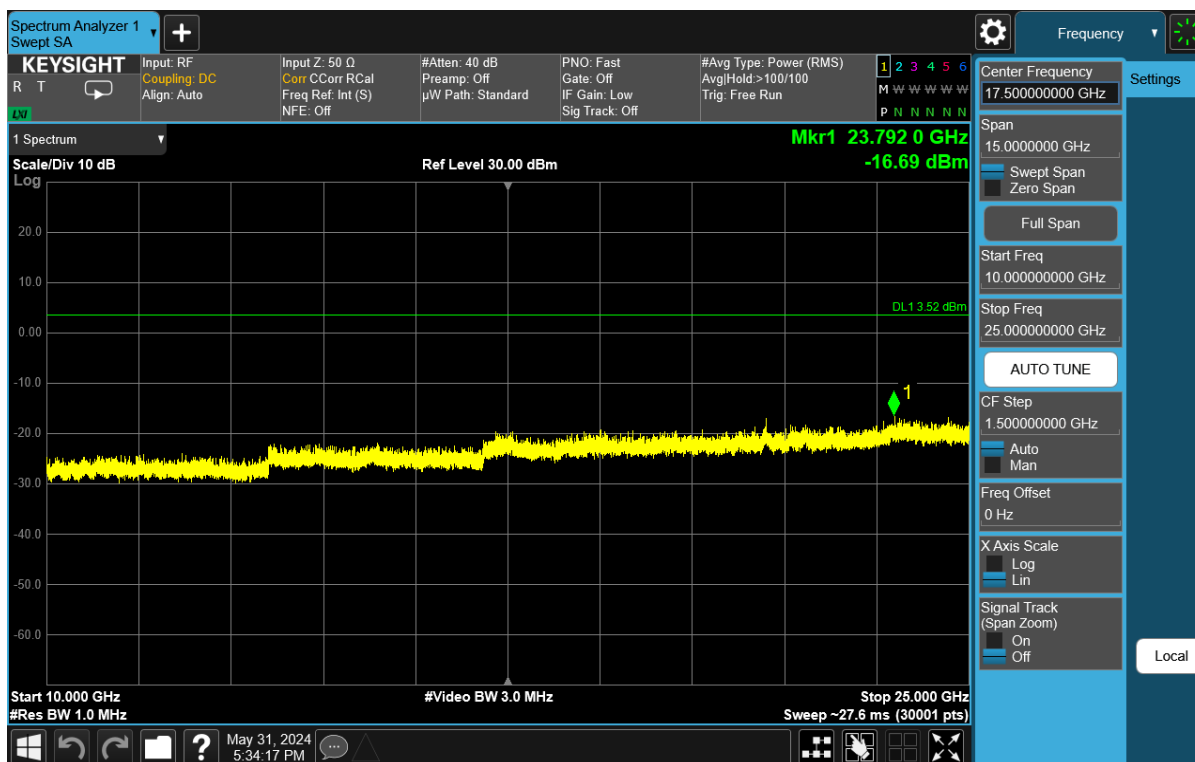
Plot 7-96. Conducted Spurious Plot Antenna WF7 (Bluetooth (LE), 1Mbps, ePA – Ch. 39)
