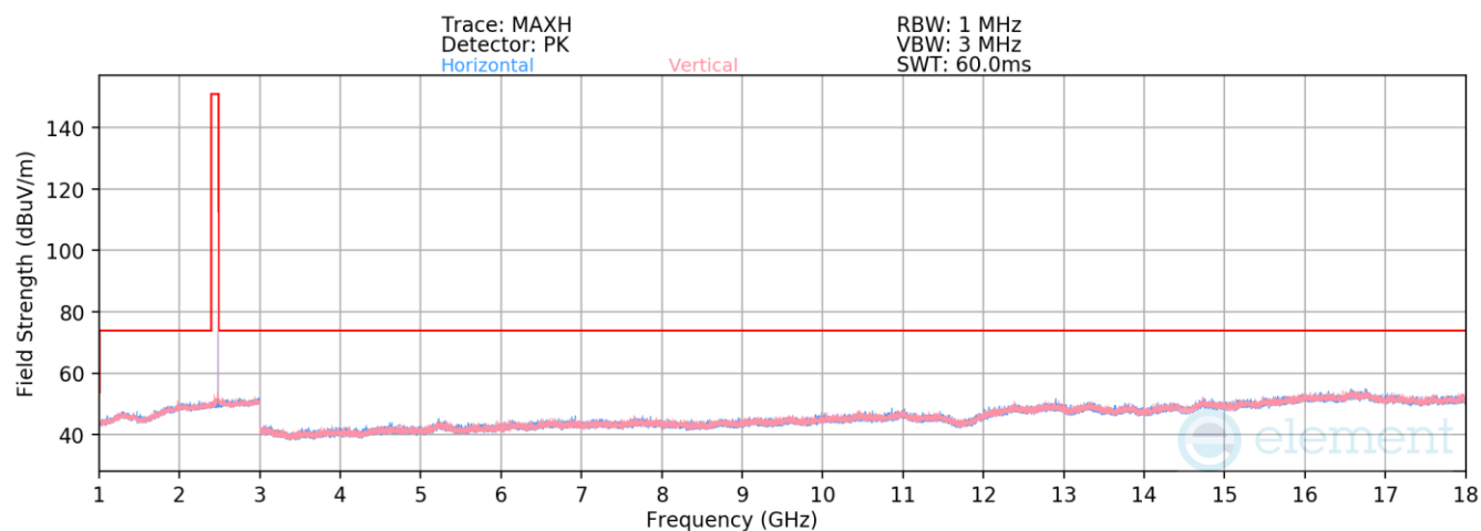
Plot 7-108. Radiated Spurious Emissions 1-18GHz Antenna WF7 (1Mbps, ePA – Ch. 39)
