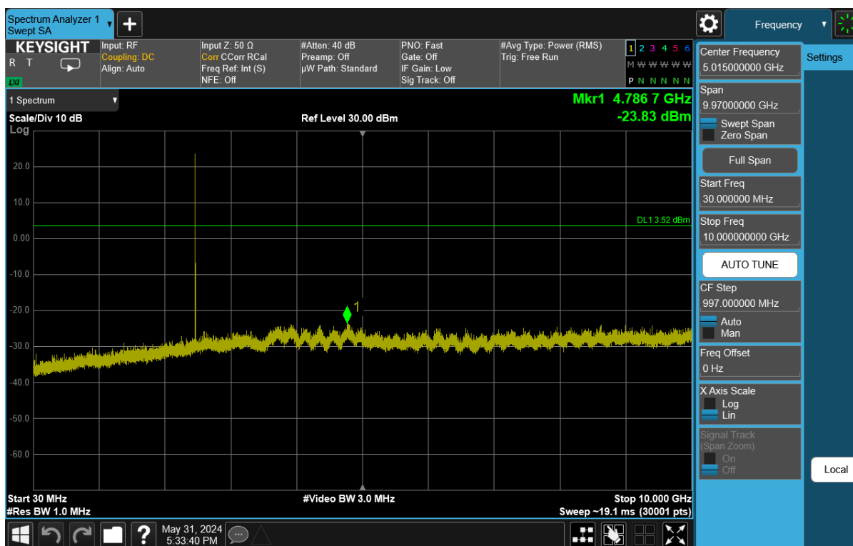
Plot 7-95. Conducted Spurious Plot Antenna WF7 (Bluetooth (LE), 1Mbps, ePA – Ch. 39)
