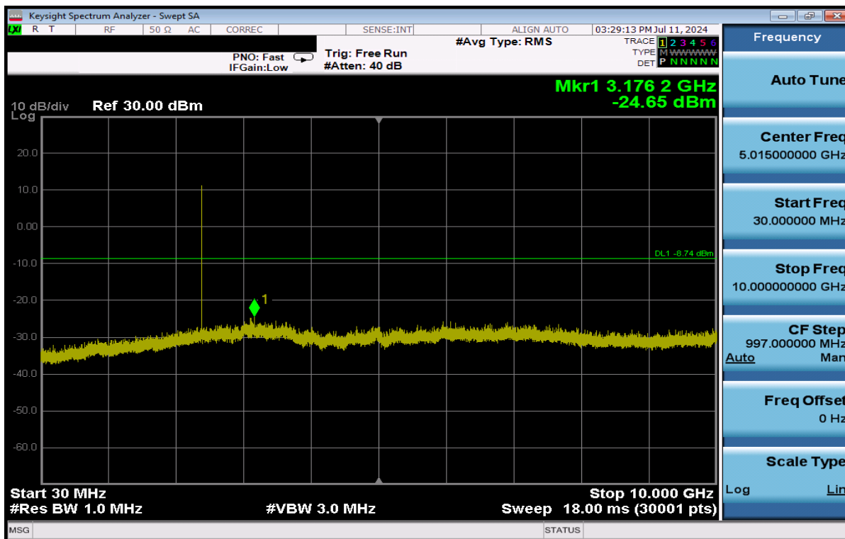
Plot 7-97. Conducted Spurious Plot Antenna WF2 (Bluetooth (LE), 1Mbps, iPA – Ch. 0)
