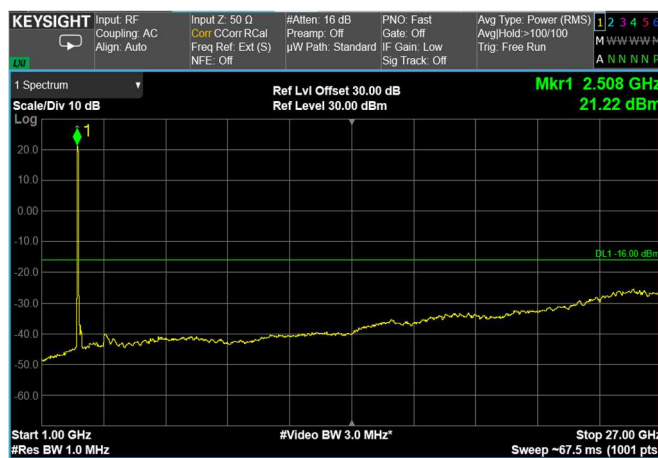
Channel: BOTTOM, Modulation: 64QAM, BW=40MHz, Range: Upper
