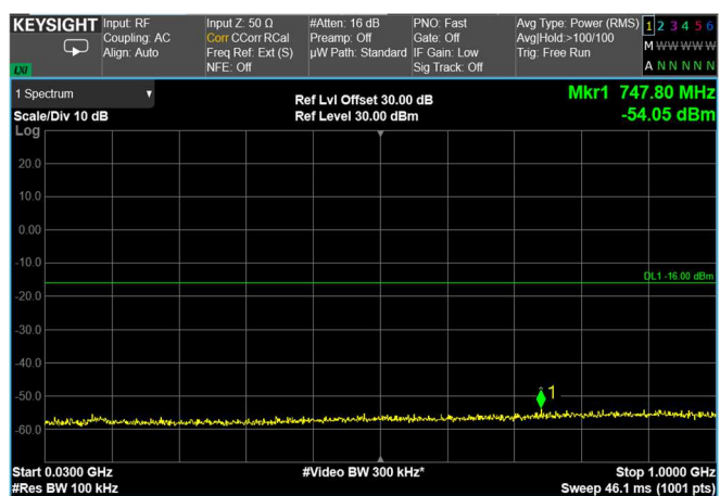
Channel: TOP, Modulation: 64QAM, BW=40MHz, Range: Lower
