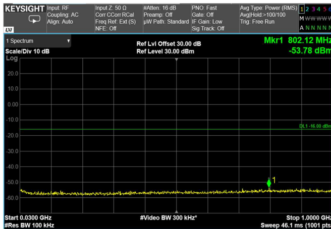
Channel: MIDDLE, Modulation: 64QAM, BW=70MHz, Range: Lower
