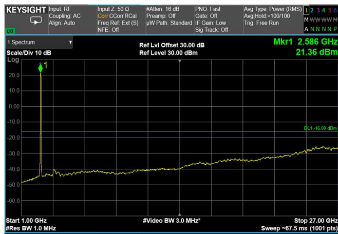
Channel: MIDDLE, Modulation: 64QAM, BW=40MHz, Range: Upper
