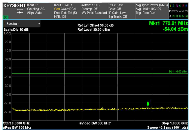
Channel: MIDDLE, Modulation: 64QAM, BW=40MHz, Range: Lower
