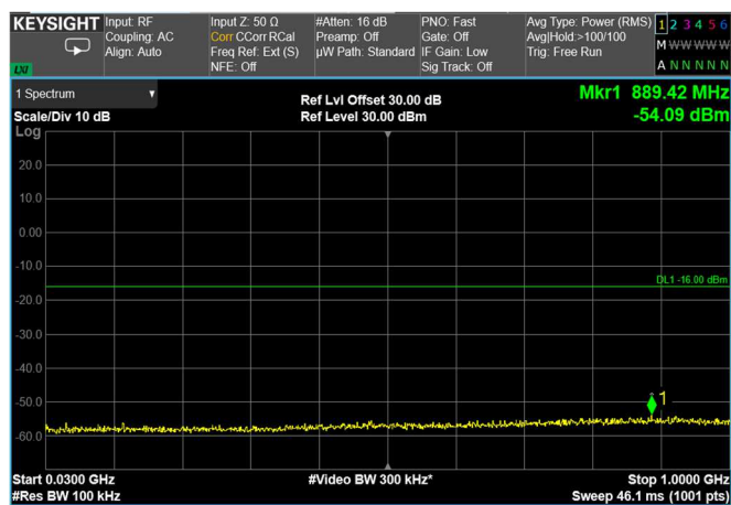
Channel: BOTTOM, Modulation: 64QAM, BW=40MHz, Range: Lower
