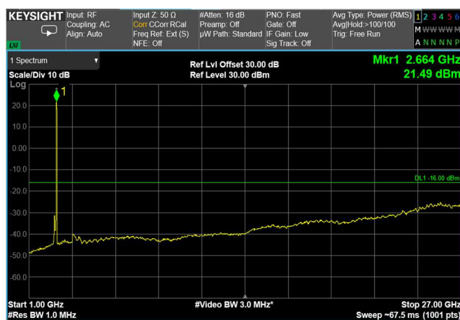
Channel: TOP, Modulation: 64QAM, BW=40MHz, Range: Upper
