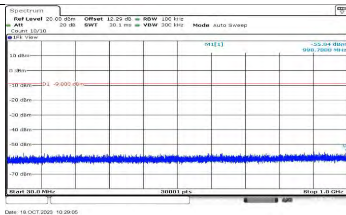
DH5_Ant1_2441_30~1000
