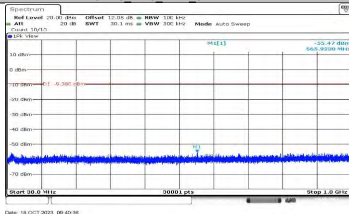
3DH5_Ant0_2441_30~1000
