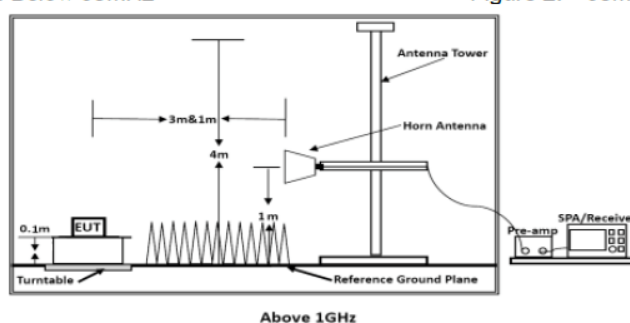
Figure 3. Above 1GHz
