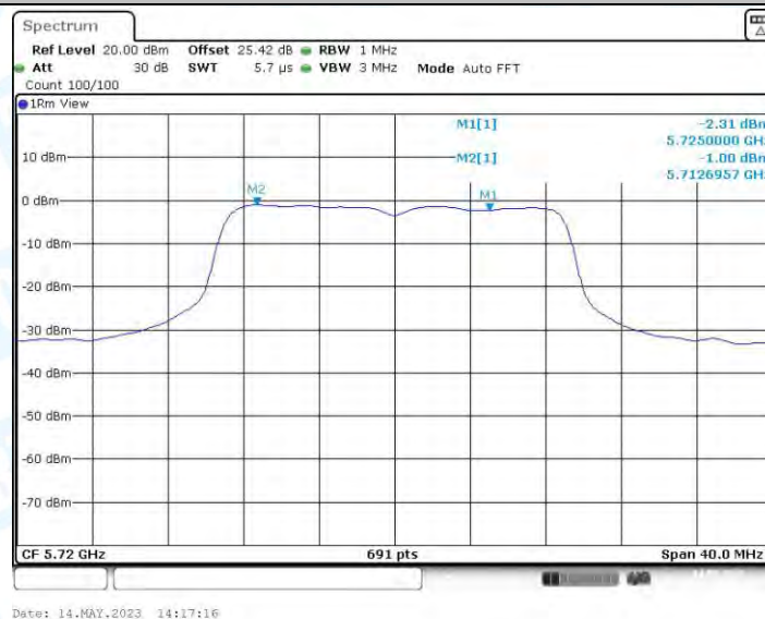
11AC20MIMO_Ant4_5720_UNII-2C
