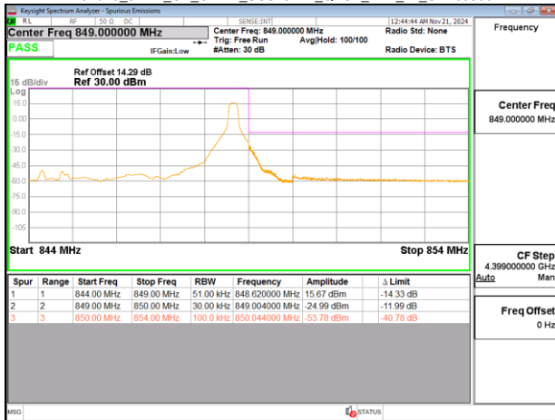
Band26_5MHz_CP_OFDM_SCS15kHz_QPSK_RB25_0_CH169300
