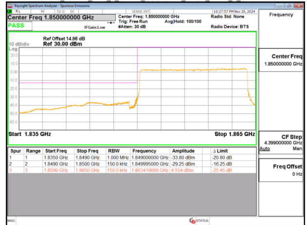
Band25_15MHz_DFT_s_OFDM_SCS15kHz_BPSK_RB1_78_CH371500
