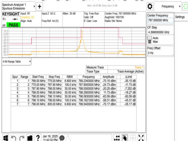
Band14_5MHz_CP_OFDM_SCS15kHz_QPSK_RB1_0_CH158100
