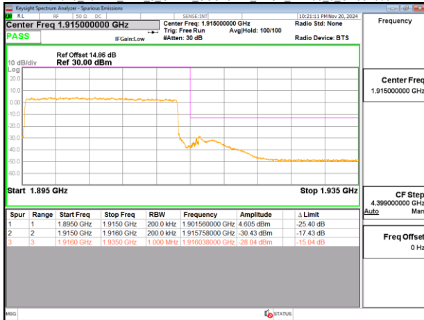
Band25_20MHz_DFT_s_OFDM_SCS15kHz_BPSK_RB1_105_CH381000
