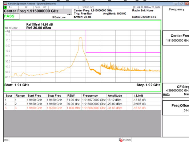
Band25_5MHz_CP_OFDM_SCS15kHz_QPSK_RB25_0_CH382500
