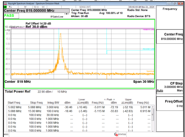
Band26-Part90s_10MHz_DFT_s_OFDM_SCS15kHz_BPSK_RB1_51_CH163800
