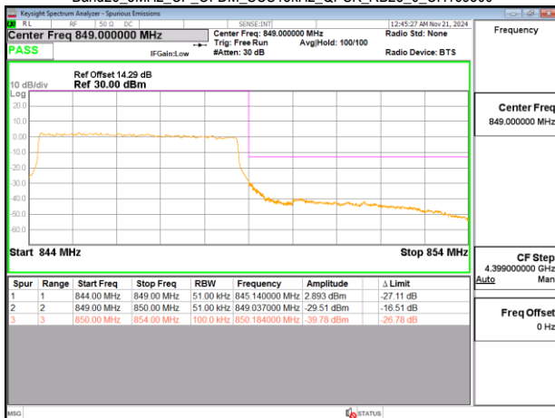
Band26_5MHz_CP_OFDM_SCS15kHz_QPSK_RB25_0_CH169300
