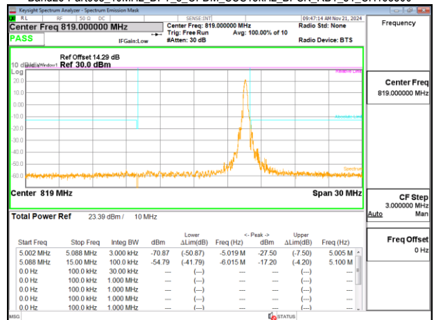
Band26-Part90s_10MHz_DFT_s_OFDM_SCS15kHz_BPSK_RB1_51_CH163800
