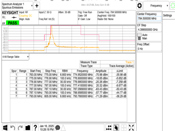
Band13_10MHz_DFT_s_OFDM_SCS15kHz_BPSK_RB50_0_CH156400
