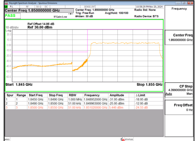
Band25_5MHz_DFT_s_OFDM_SCS15kHz_BPSK_RB25_0_CH370500
