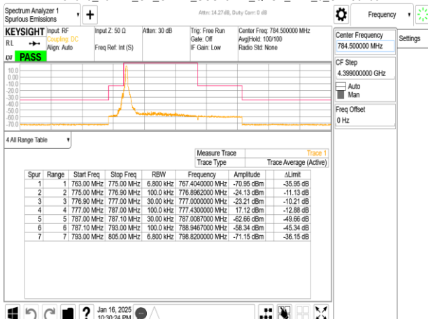
Band13_10MHz_CP_OFDM_SCS15kHz_QPSK_RB1_0_CH156400
