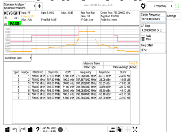
Band14_5MHz_DFT_s_OFDM_SCS15kHz_BPSK_RB25_0_CH158100
