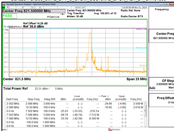
Band26-Part90s_5MHz_DFT_s_OFDM_SCS15kHz_BPSK_RB1_24_CH164300
