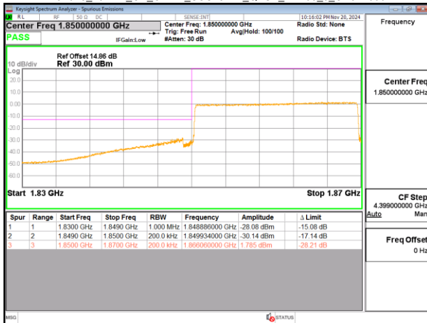
Band25_20MHz_CP_OFDM_SCS15kHz_QPSK_RB106_0_CH372000
