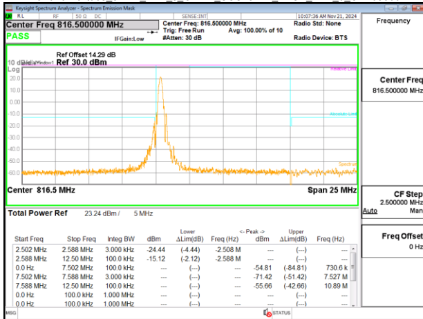
Band26-Part90s_5MHz_DFT_s_OFDM_SCS15kHz_BPSK_RB25_0_CH163300
