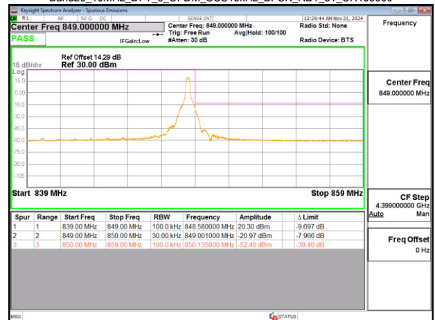
Band26_10MHz_DFT_s_OFDM_SCS15kHz_BPSK_RB1_51_CH168800
