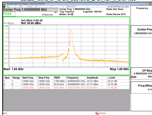
Band25_10MHz_CP_OFDM_SCS15kHz_QPSK_RB52_0_CH371000
