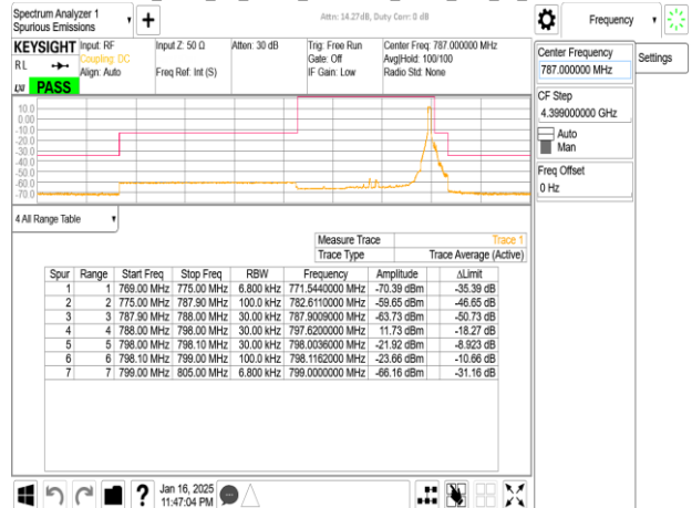
Band14_5MHz_CP_OFDM_SCS15kHz_QPSK_RB25_0_CH159100
