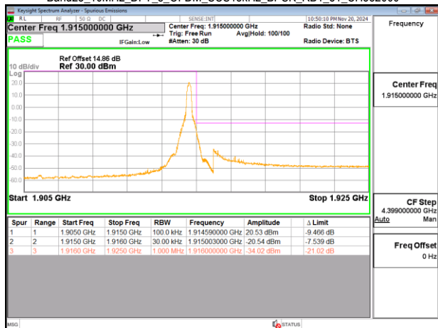
Band25_10MHz_DFT_s_OFDM_SCS15kHz_BPSK_RB1_51_CH382000
