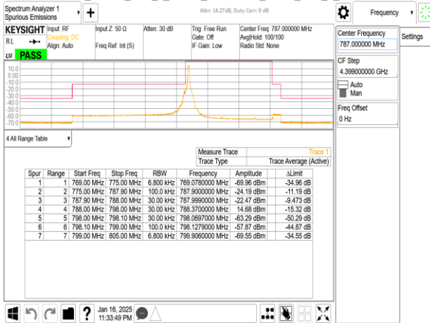
Band14_10MHz_DFT_s_OFDM_SCS15kHz_BPSK_RB50_0_CH158600
