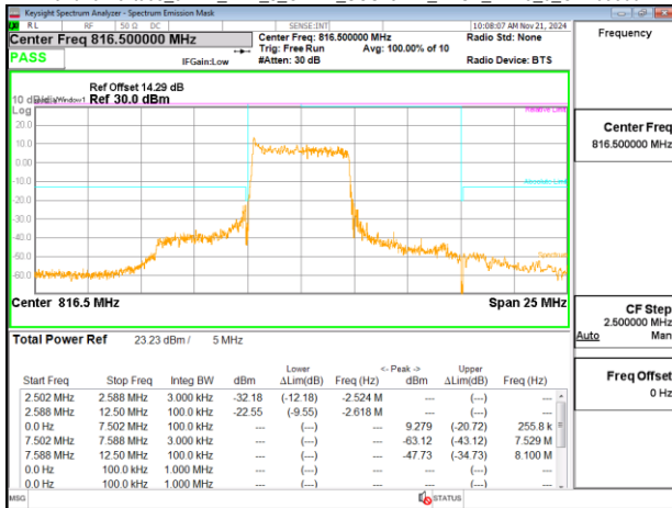
Band26-Part90s_5MHz_DFT_s_OFDM_SCS15kHz_BPSK_RB1_24_CH164300
