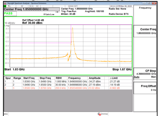
Band25_20MHz_DFT_s_OFDM_SCS15kHz_BPSK_RB1_0_CH372000
