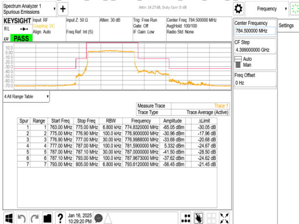
Band13_10MHz_CP_OFDM_SCS15kHz_QPSK_RB1_0_CH156400
