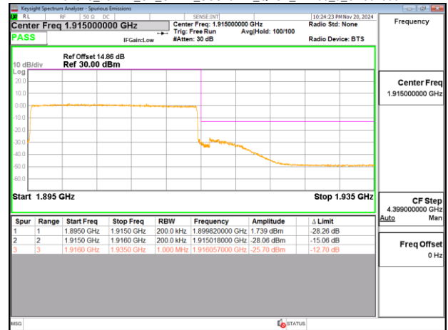
Band25_20MHz_CP_OFDM_SCS15kHz_QPSK_RB1_105_CH381000
