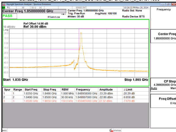
Band25_15MHz_DFT_s_OFDM_SCS15kHz_BPSK_RB1_0_CH371500
