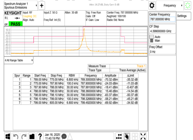
Band14_5MHz_DFT_s_OFDM_SCS15kHz_BPSK_RB25_0_CH158100
