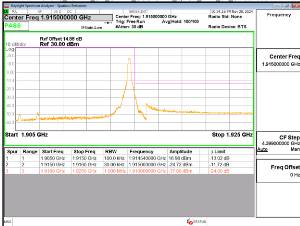
Band25_10MHz_CP_OFDM_SCS15kHz_QPSK_RB52_0_CH382000
