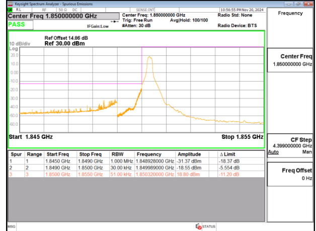
Band25_5MHz_DFT_s_OFDM_SCS15kHz_BPSK_RB25_0_CH370500
