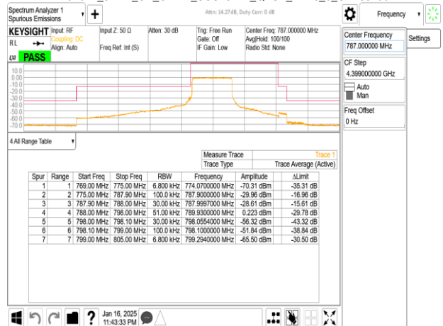
Band14_5MHz_CP_OFDM_SCS15kHz_QPSK_RB1_24_CH159100
