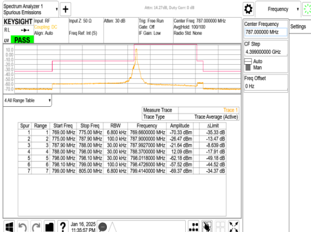
Band14_10MHz_CP_OFDM_SCS15kHz_QPSK_RB1_0_CH158600
