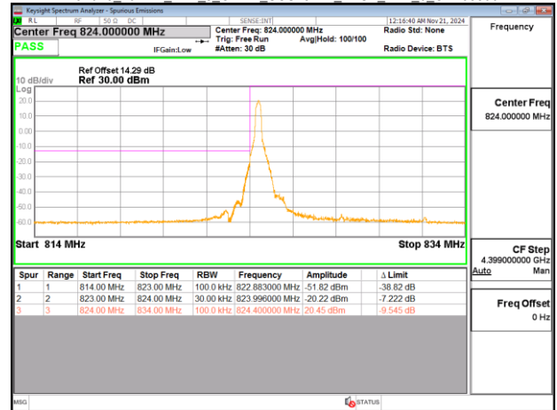
Band26_10MHz_DFT_s_OFDM_SCS15kHz_BPSK_RB50_0_CH165800
