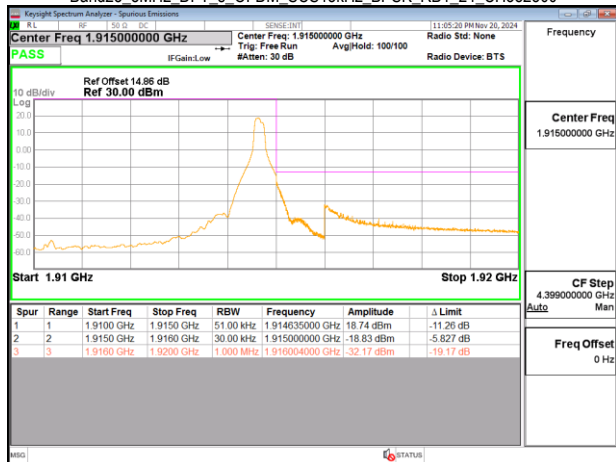
Band25_5MHz_DFT_s_OFDM_SCS15kHz_BPSK_RB25_0_CH382500
