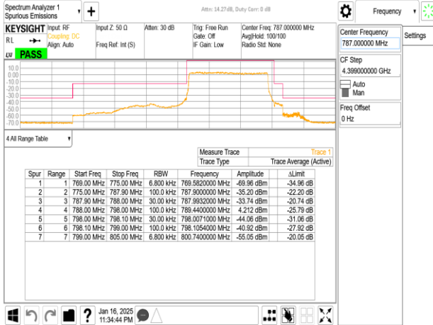
Band14_10MHz_CP_OFDM_SCS15kHz_QPSK_RB1_0_CH158600
