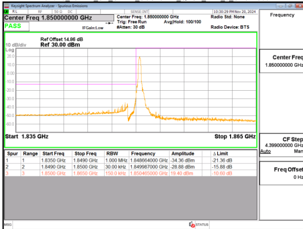
Band25_15MHz_CP_OFDM_SCS15kHz_QPSK_RB79_0_CH371500
