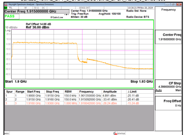
Band25_15MHz_DFT_s_OFDM_SCS15kHz_BPSK_RB75_0_CH371500
