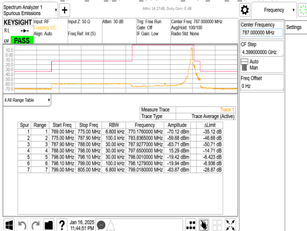
Band14_5MHz_DFT_s_OFDM_SCS15kHz_BPSK_RB25_0_CH159100
