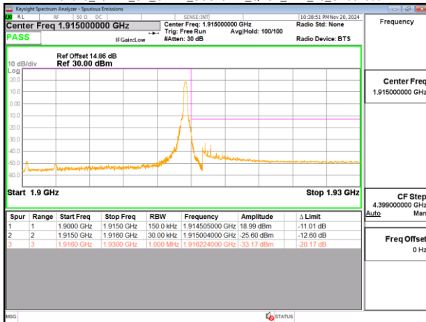
Band25_15MHz_CP_OFDM_SCS15kHz_QPSK_RB1_78_CH381500
