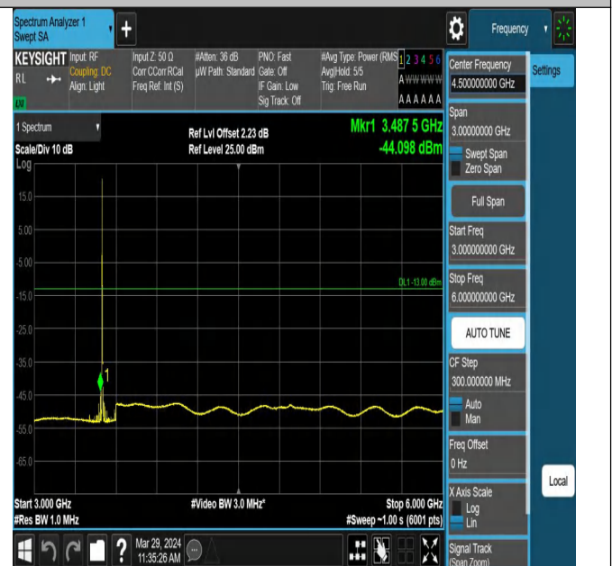
Band42_5MHz_QPSK_42590_1RB#0_3000~6000_3000~600
