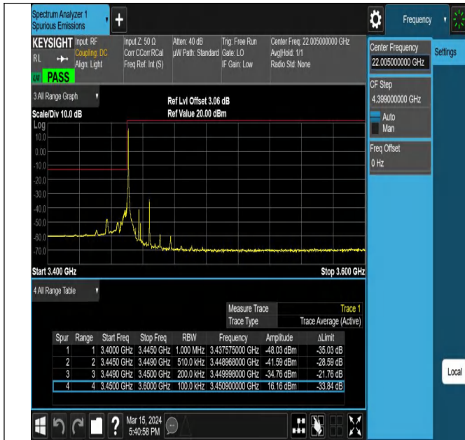
Band42_15MHz_QPSK_42165_1RB#0
