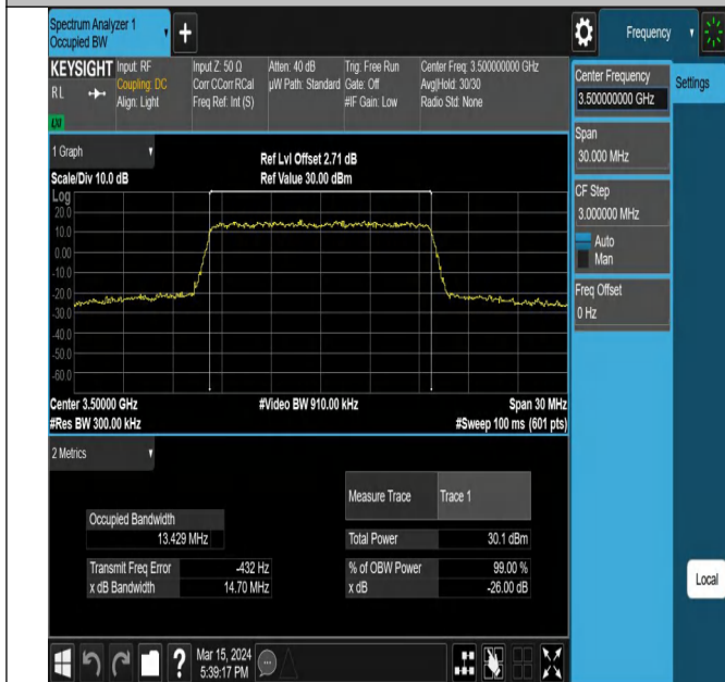
42(3450-3550)-15MHz-QPSK-42590-75RB#0-PASS
