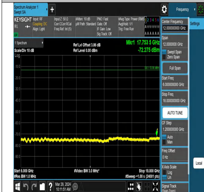
Band42_10MHz_QPSK_42140_1RB#0_6000~18000_6000~1
