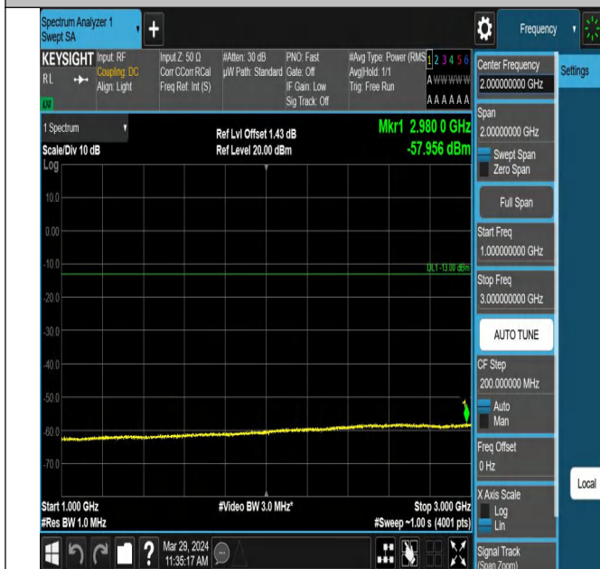
Band42_5MHz_QPSK_42590_1RB#0_1000~3000_1000~300
