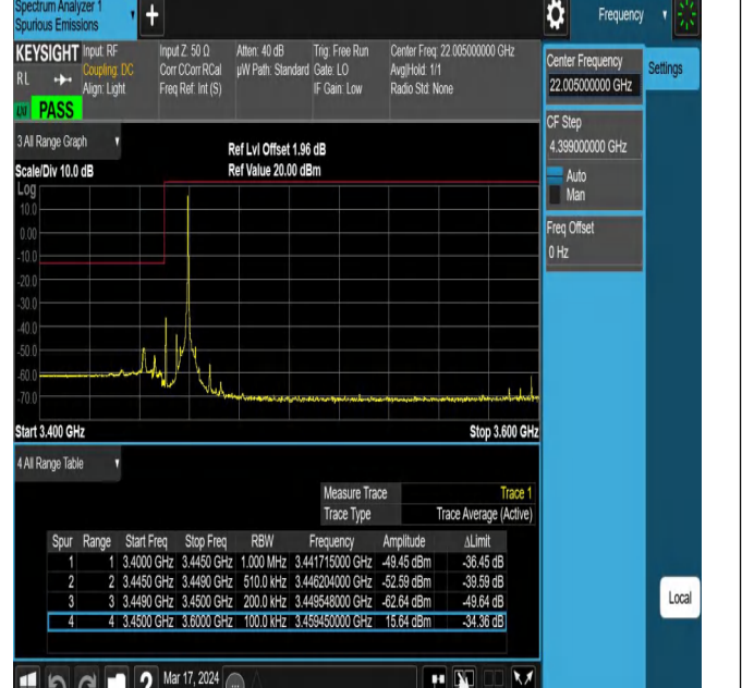
Band42_10MHz_QPSK_42140_1RB#49
