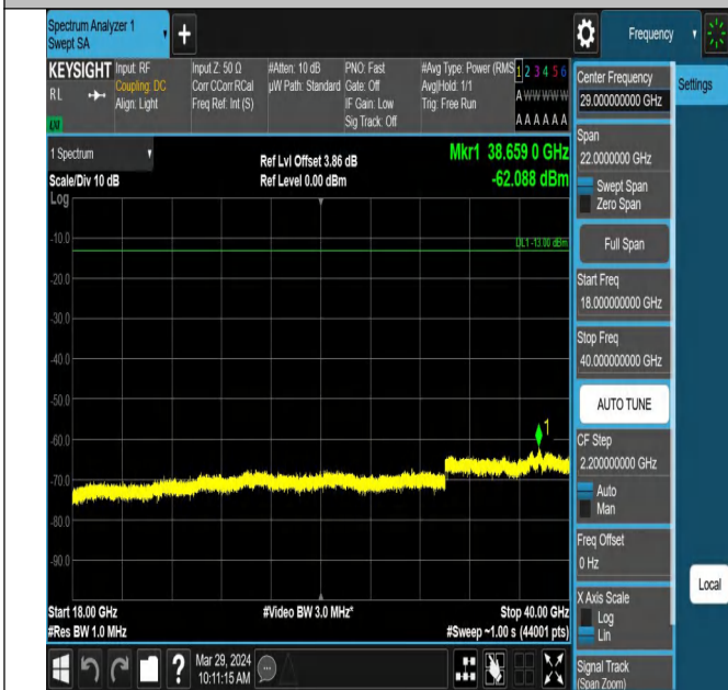
Band42_5MHz_QPSK_42115_1RB#0_18000~40000_18000~40000
