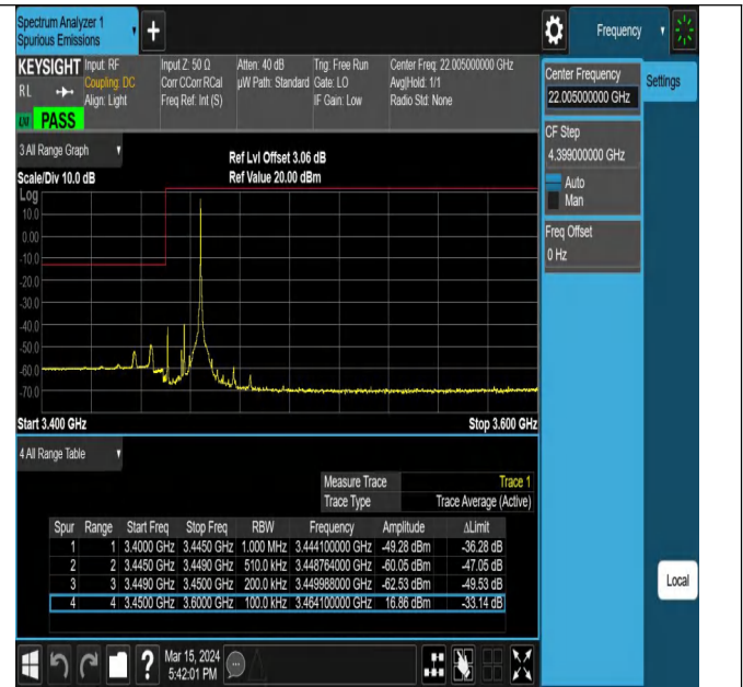
Band42_15MHz_QPSK_42165_1RB#74
