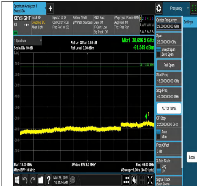
Band42_5MHz_QPSK_43065_1RB#0_18000~40000_18000~40000
