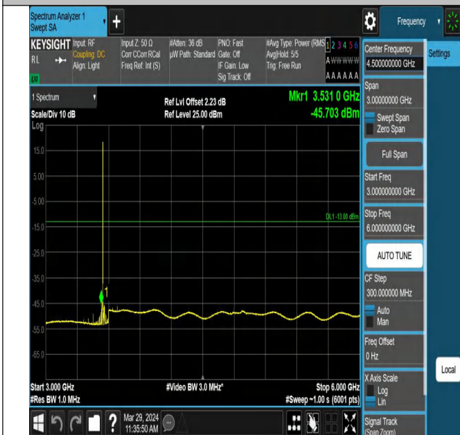
Band42_5MHz_QPSK_43065_1RB#0_3000~6000_3000~6000
