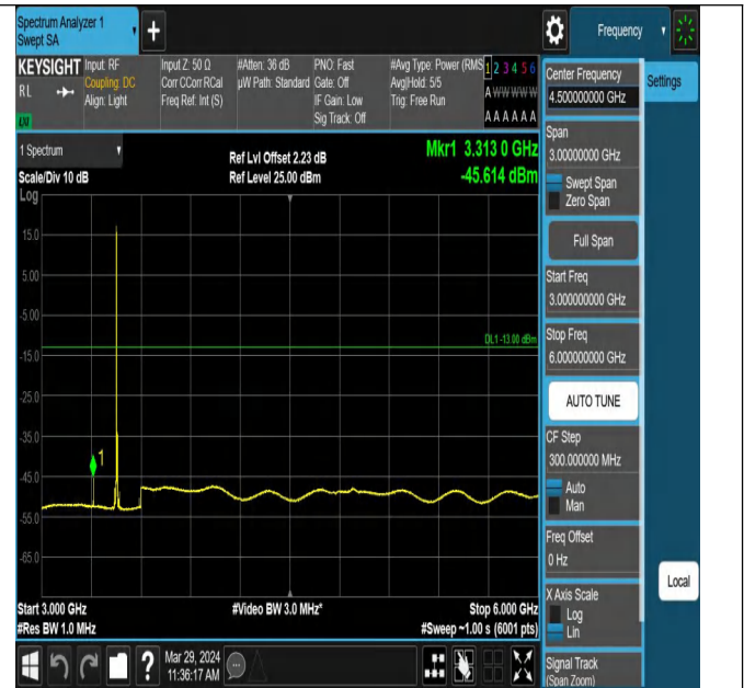
Band42_10MHz_QPSK_42140_1RB#0_3000~6000_3000~60
