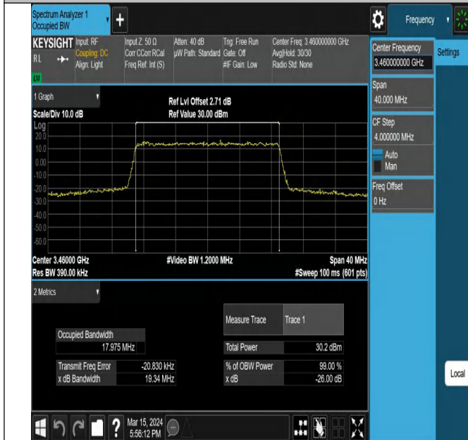
42(3450-3550)-20MHz-QPSK-42190-100RB#0-PASS
