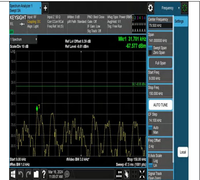
Band42_10MHz_QPSK_42140_1RB#0_0.009~0.15_0.009~0.15
