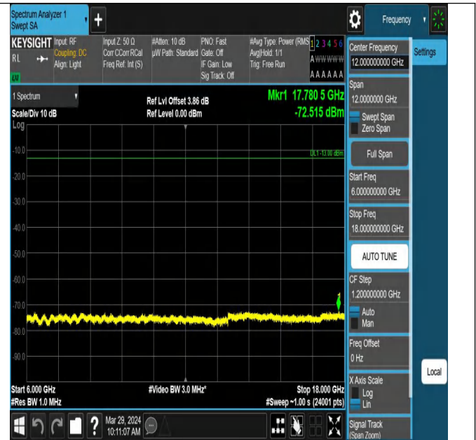
Band42_5MHz_QPSK_42115_1RB#0_6000~18000_6000~18000
