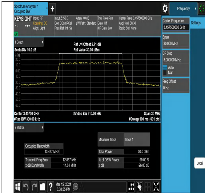
42(3450-3550)-15MHz-QPSK-42165-75RB#0-PASS
