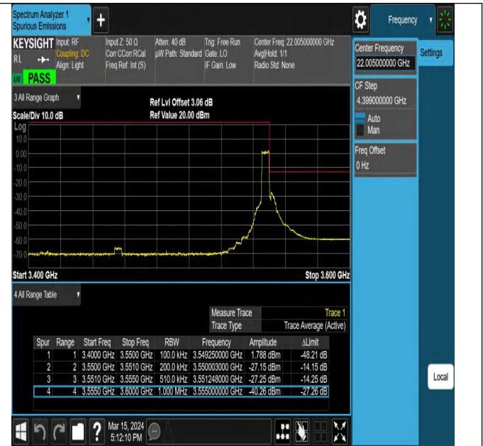
Band42_5MHz_QPSK_43065_25RB#0
