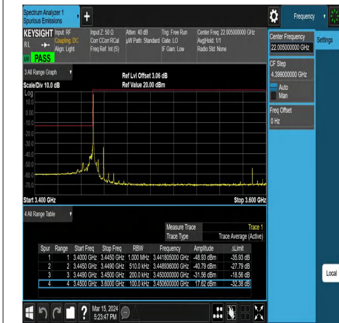
Band42_10MHz_QPSK_42140_1RB#0
