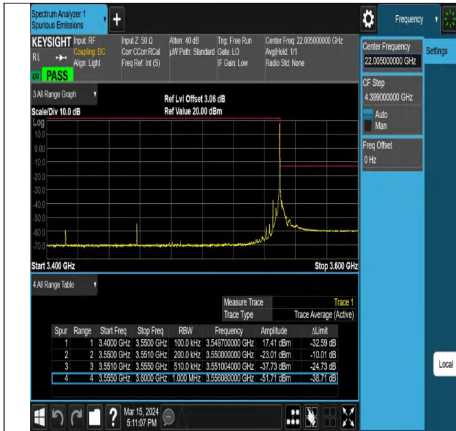
Band42_5MHz_QPSK_43065_1RB#24
