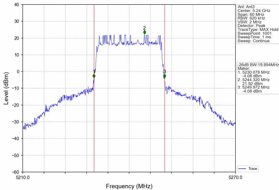
20_HCH_5240MHz_Ant3_NTNV
