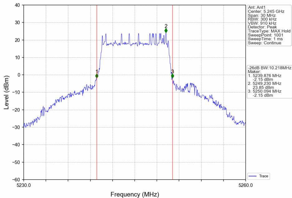
10_HCH_5245MHz_Ant1_NTNV
