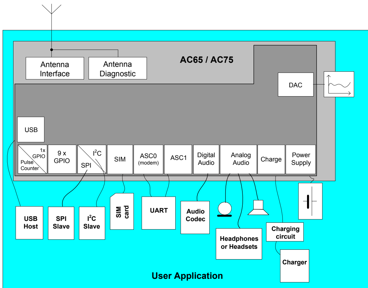
Figure 1: AC65/AC75 system overview
