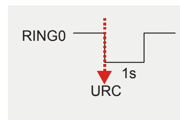
Figure 37: URC transmission
