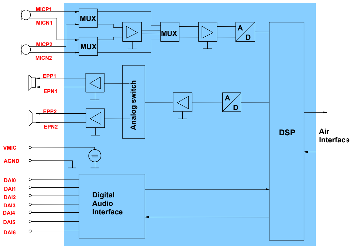
Figure 23: Audio block diagram
