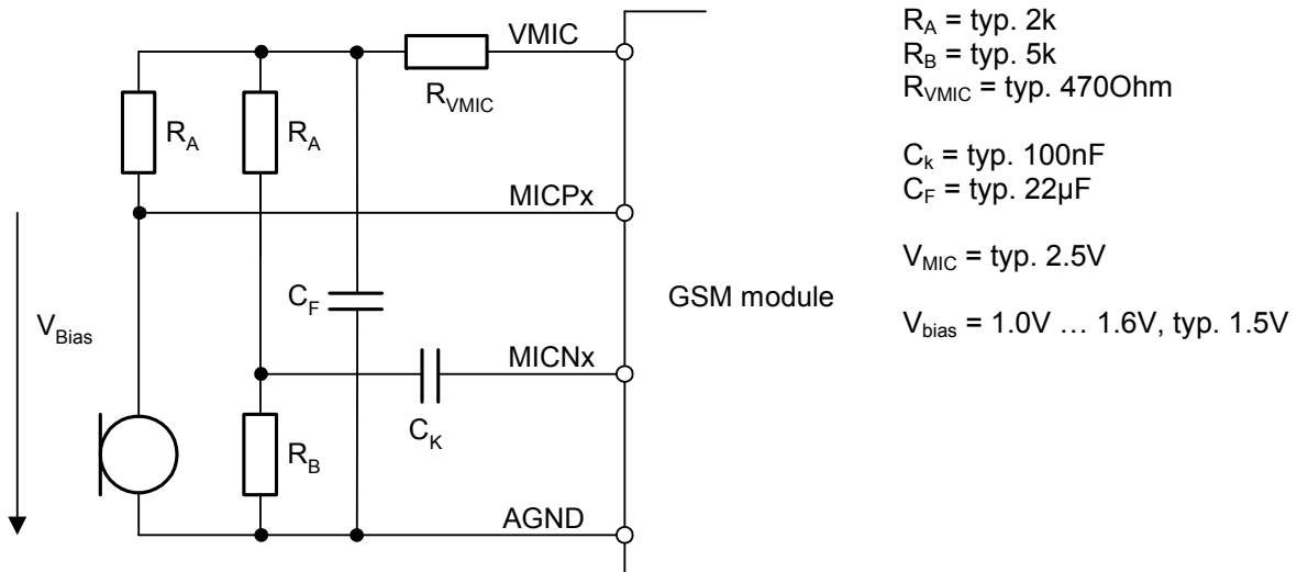
Figure 24: Single ended microphone input
