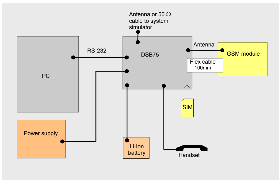
Figure 47: Reference equipment for Type Approval
