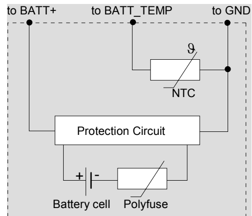
Figure 9: Battery pack circuit diagram
