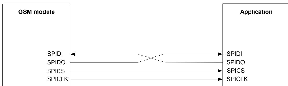
Figure 21: SPI interface
