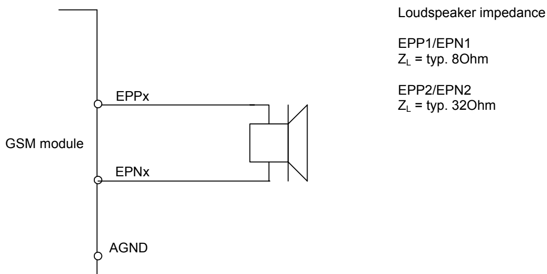
Figure 27: Differential loudspeaker configuration
