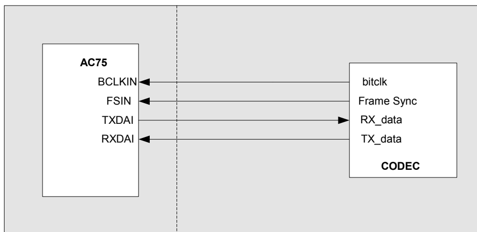
Figure 31: Slave PCM interface application
