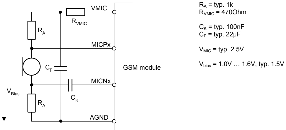
Figure 25: Differential microphone input
