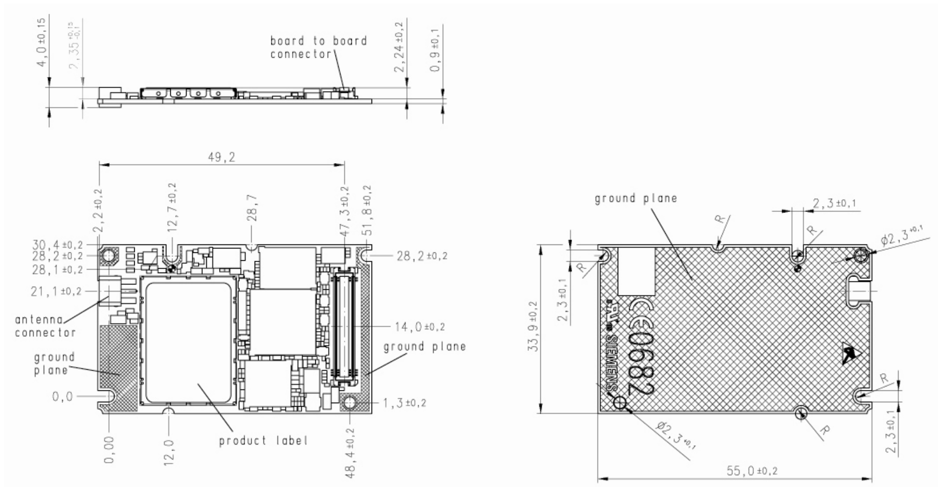
Figure 43: Dimensions of AC65/AC75
