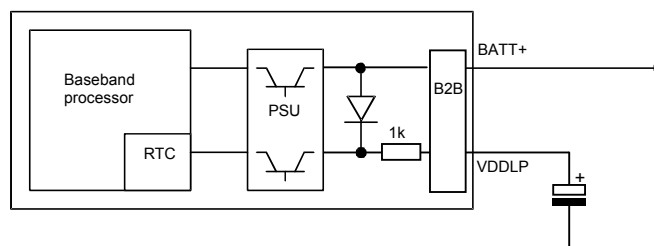
Figure 13: RTC supply from capacitor
