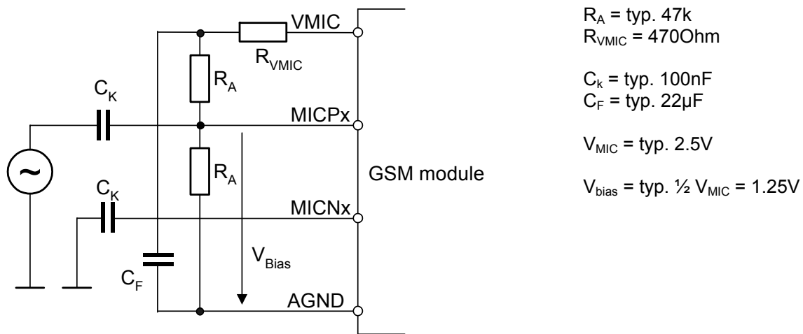
Figure 26: Line input configuration with OpAmp
