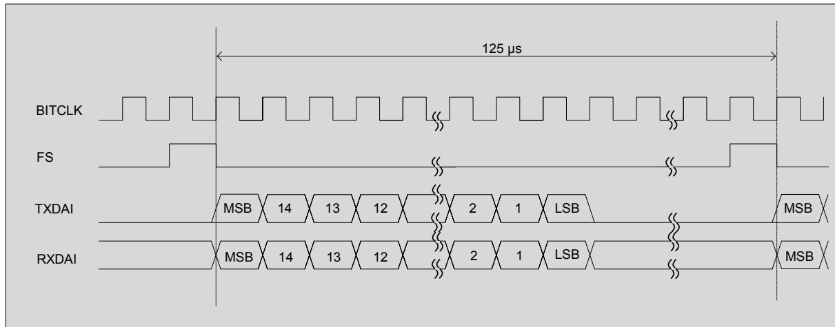
Figure 29: Master PCM timing, short frame selected
