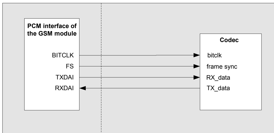
Figure 28: Master PCM interface Application
