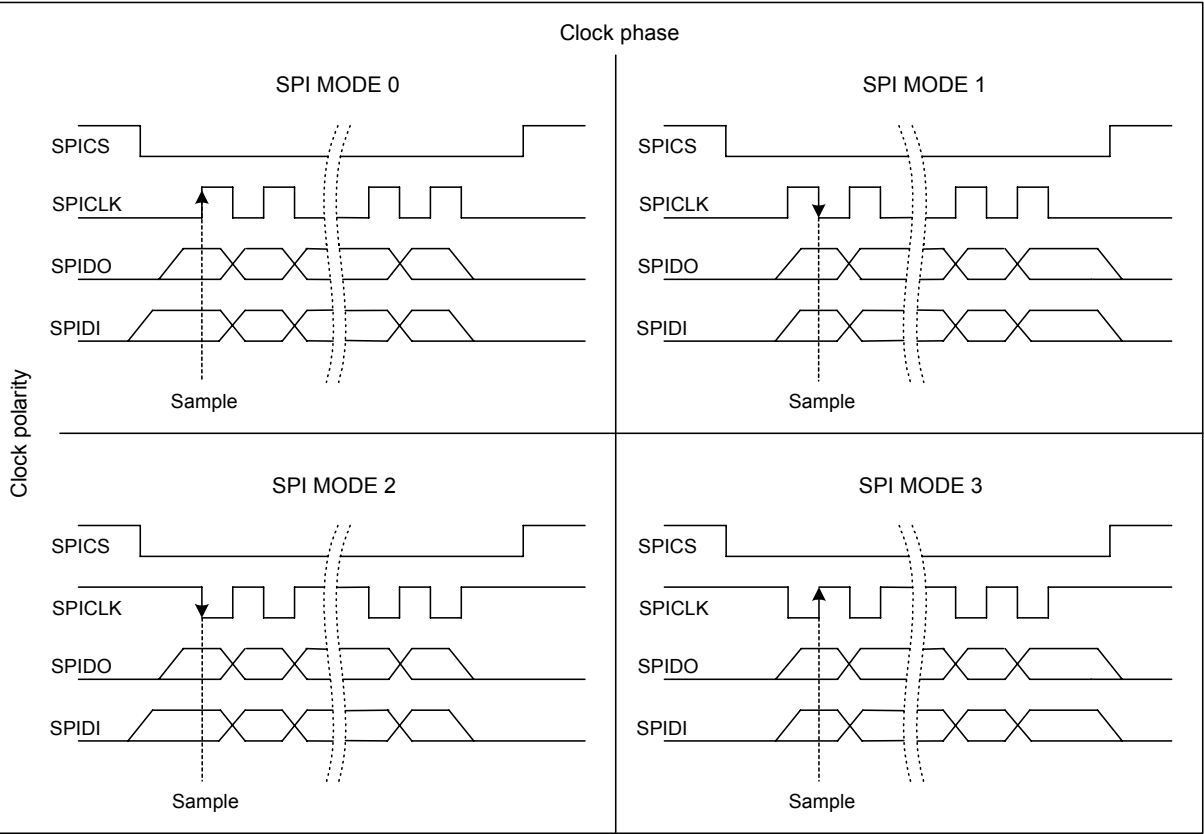
Figure 22: Characteristics of SPI modes
