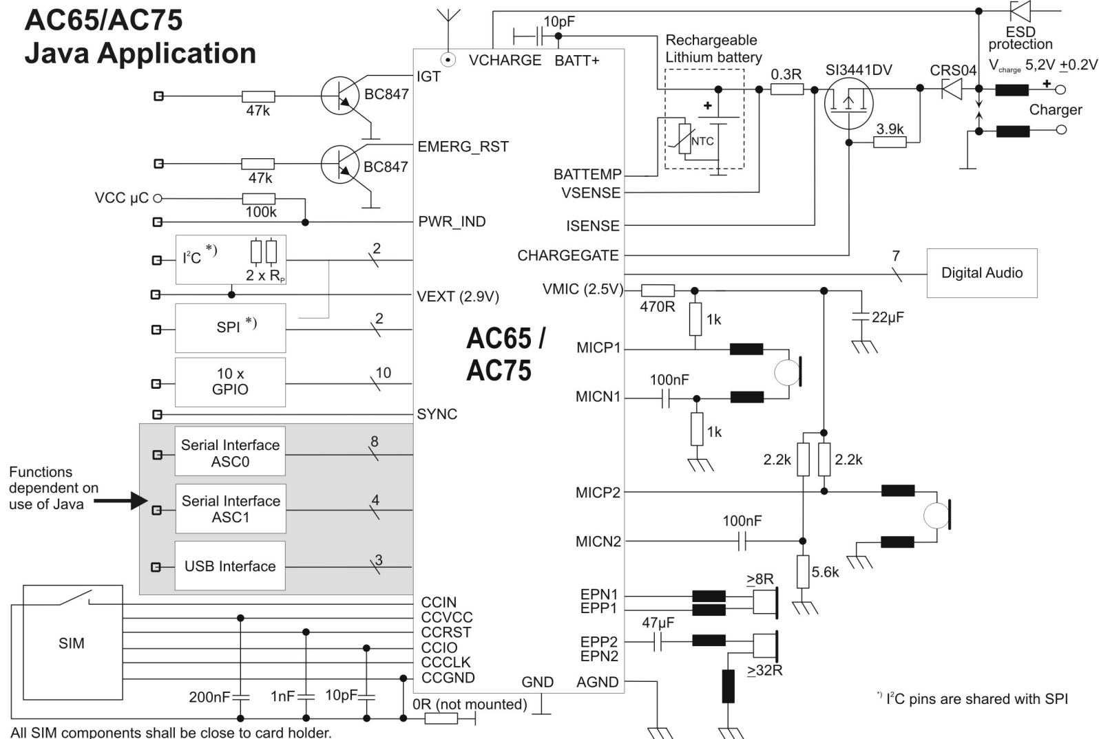
Figure 46: AC65/AC75 sample application for Java
