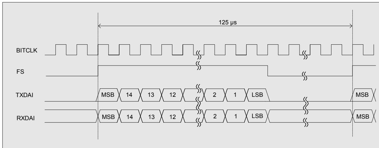
Figure 30: Master PCM timing, long frame selected
