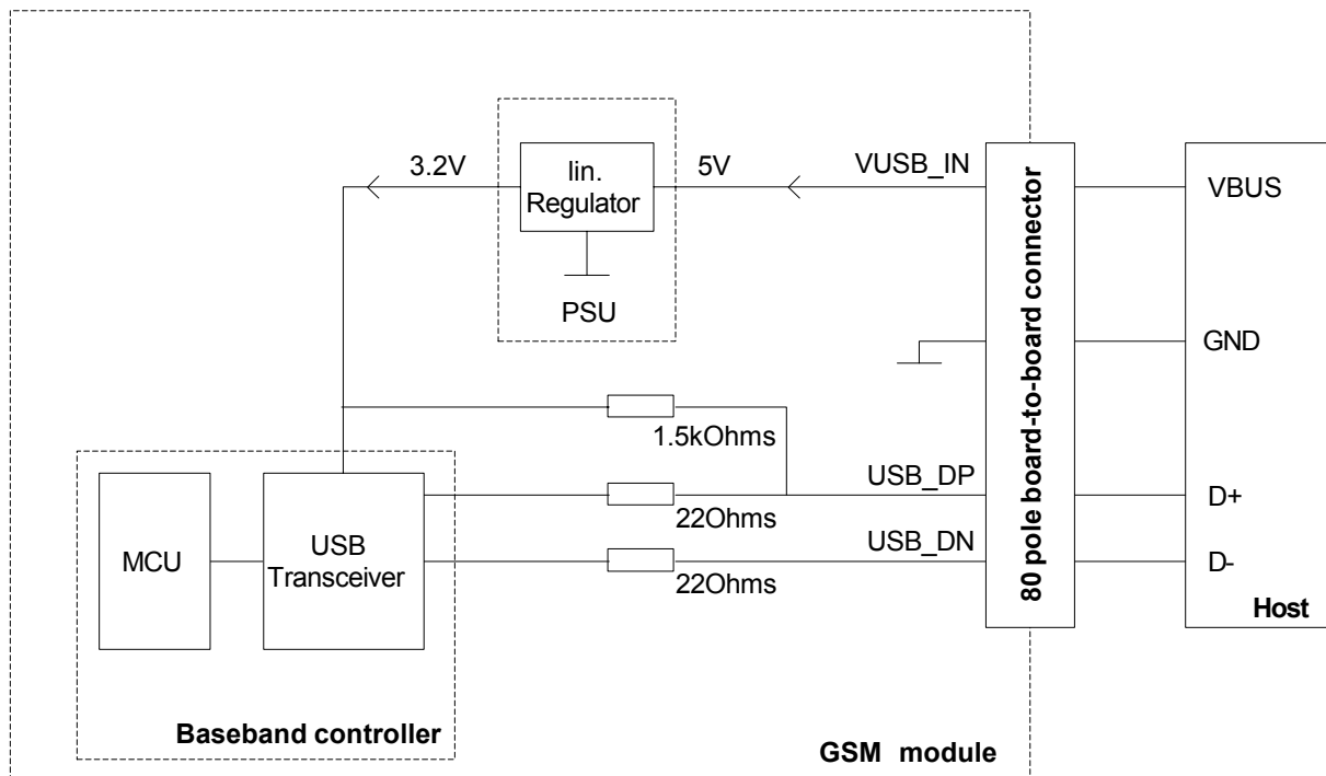
Figure 18: USB circuit
