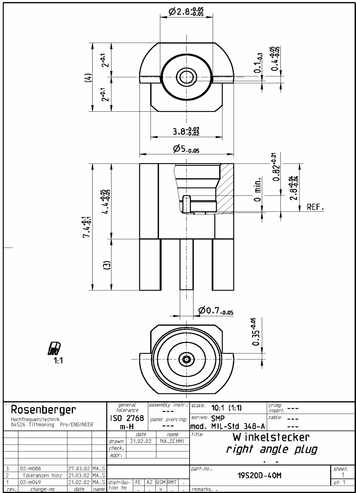
Figure 39: Datasheet of Rosenberger SMP MIL-Std 348-A connector
