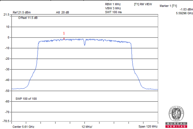
802.11ac (VHT160(80+80)) / Chain 3 / Ch 122
