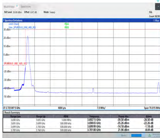
1-N77-3700-3980-PC1-30-60-L-1-DFT-PI2BPSK-Edg e_1RB_Left-1@0-Ant1-1--PASS-see graph
