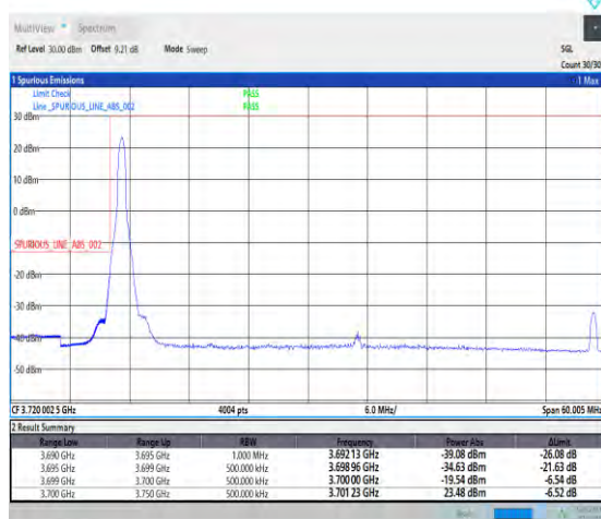
1-N77-3700-3980-PC1-30-50-L-4-CP-QPSK-Edge_1 RB_Left-1@0-Ant1-1--PASS-see graph
