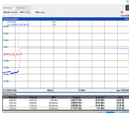
1-N77-3700-3980-PC1-30-70-L-6-CP-QPSK-Outer_Full-189@0-Ant1-1--PASS-see graph
