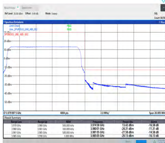
1-N77-3700-3980-PC1-30-10-H-6-CP-QPSK-Outer_Full-24@0-Ant1-1--PASS-see graph
