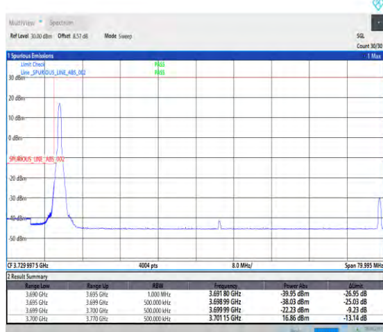
1-N77-3700-3980-PC1-30-70-L-4-CP-QPSK-Edge_1RB_Left-1@0-Ant1-1--PASS-see graph
