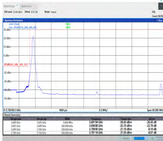
1-N77-3700-3980-PC1-30-50-L-1-DFT-PI2BPSK-Edg e_1RB_Left-1@0-Ant1-1--PASS-see graph
