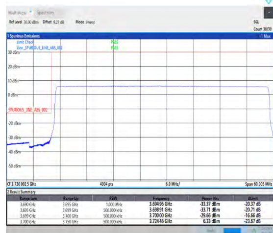
1-N77-3700-3980-PC1-30-50-L-6-CP-QPSK-Outer_ Full-133@0-Ant1-1--PASS-see graph
