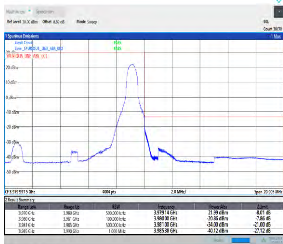
1-N77-3700-3980-PC1-30-10-H-2-DFT-PI2BPSK-Edge_1RB_Right-1@23-Ant1-1--PASS-see graph
