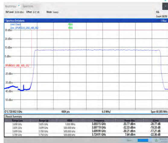
1-N77-3700-3980-PC1-30-50-L-3-DFT-PI2BPSK-O uter_Full-128@0-Ant1-1--PASS-see graph
