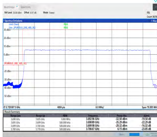
1-N77-3700-3980-PC1-30-70-L-3-DFT-PI2BPSK-Outer_Full-180@0-Ant1-1--PASS-see graph
