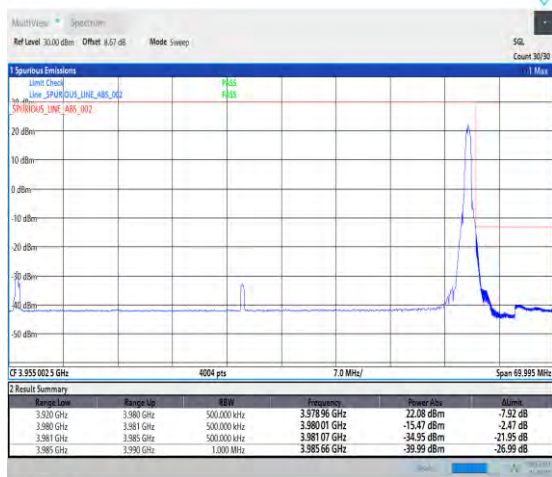
1-N77-3700-3980-PC1-30-60-H-2-DFT-PI2BPSK-Edge_1RB_Right-1@161-Ant1-1--PASS-see graph
