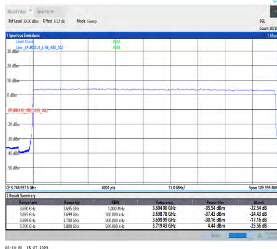
1-N77-3700-3980-PC1-30-100-L-3-DFT-PI2BPSK-Outer_Full-270@0-Ant1-1--PASS-see graph
