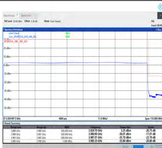
1-N77-3700-3980-PC1-30-100-H-3-DFT-PI2BPSK-Outer_Full-270@0-Ant1-1--PASS-see graph
