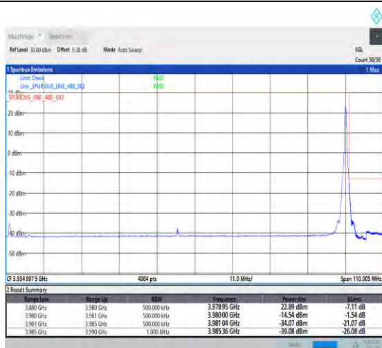
1-N77-3700-3980-PC1-30-100-H-2-DFT-PI2BPSK-Edg e_1RB_Right-1@272-Ant1-1--PASS-see graph
