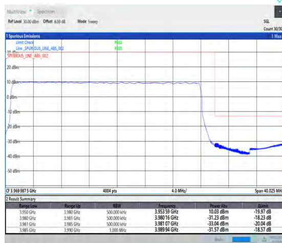
1-N77-3700-3980-PC1-30-30-H-3-DFT-PI2BPSK-Outer_Full-75@0-Ant1-1--PASS-see graph
