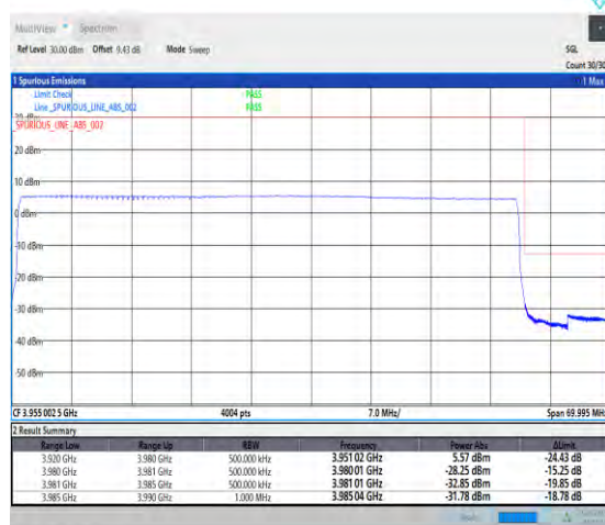
1-N77-3700-3980-PC1-30-60-H-6-CP-QPSK-Outer_Full-162@0-Ant1-1--PASS-see graph
