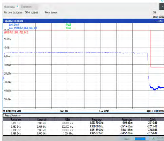
1-N77-3700-3980-PC1-30-100-H-3-DFT-PI2BPSK-Outer_Full-270@0-Ant1-1--PASS-see graph
