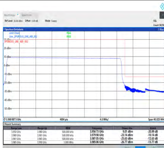
1-N77-3700-3980-PC1-30-30-H-3-DFT-PI2BPSK-Outer_Full-75@0-Ant1-1--PASS-see graph
