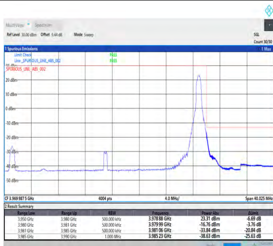
1-N77-3700-3980-PC1-30-30-H-2-DFT-PI2BPSK-Edge_1RB_Right-1@77-Ant1-1--PASS-see graph
