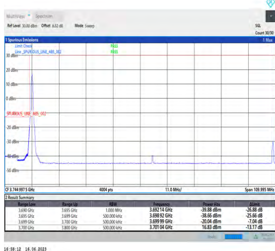
1-N77-3700-3980-PC1-30-100-L-4-CP-QPSK-Edge_1RB_Left-1@0-Ant1-1--PASS-see graph
