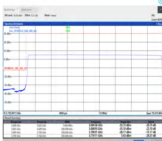
1-N77-3700-3980-PC1-30-60-L-6-CP-QPSK-Outer_ Full-162@0-Ant1-1--PASS-see graph
