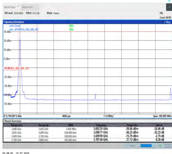
1-N77-3700-3980-PC1-30-100-L-1-DFT-PI2BPSK-Edge_1RB_Left-1@0-Ant1-1--PASS-see graph
