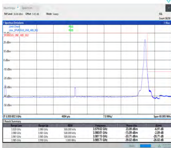
1-N77-3700-3980-PC1-30-60-H-5-CP-QPSK-Edge_1RB_Right-1@161-Ant1-1--PASS-see graph
