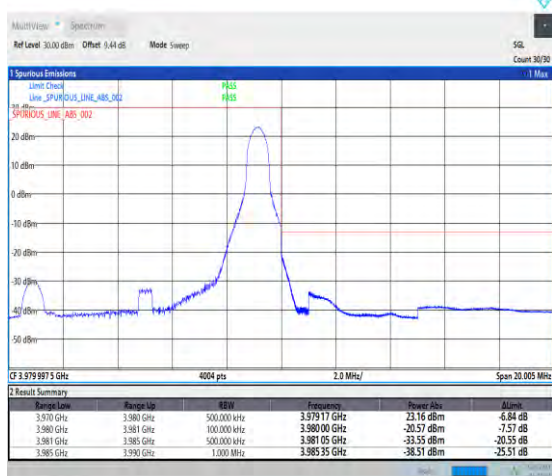
1-N77-3700-3980-PC1-30-10-H-5-CP-QPSK-Edge_1RB_Right-1@23-Ant1-1--PASS-see graph
