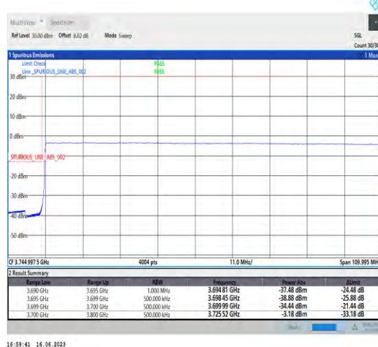
1-N77-3700-3980-PC1-30-100-L-6-CP-QPSK-Outer_Full-273@0-Ant1-1--PASS-see graph
