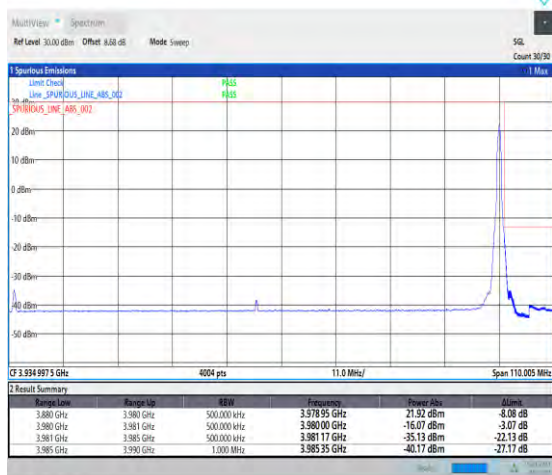
1-N77-3700-3980-PC1-30-100-H-2-DFT-PI2BPSK-Edg e_1RB_Right-1@272-Ant1-1--PASS-see graph
