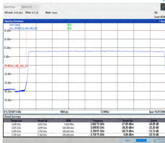
1-N77-3700-3980-PC1-30-60-L-3-DFT-PI2BPSK-O uter_Full-162@0-Ant1-1--PASS-see graph
