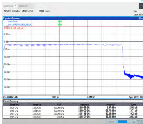
1-N77-3700-3980-PC1-30-60-H-3-DFT-PI2BPSK-Outer_Full-162@0-Ant1-1--PASS-see graph
