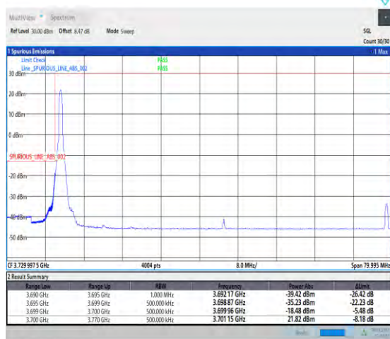
1-N77-3700-3980-PC1-30-70-L-1-DFT-PI2BPSK-Edg_e_1RB_Left-1@0-Ant1-1--PASS-see graph
