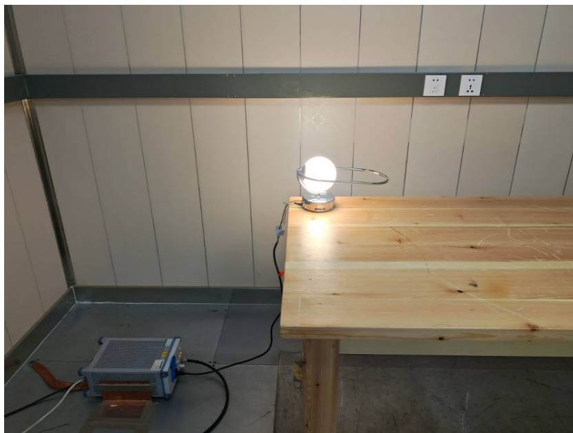
Conducted Disturbance
