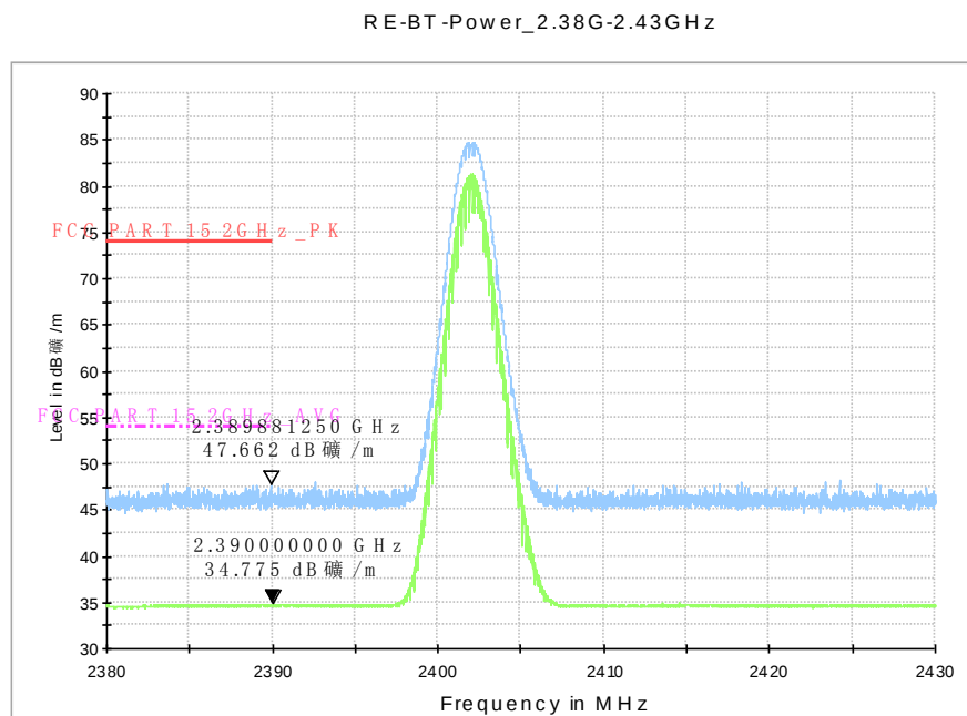
Fig.76. Radiated emission (Power): \pi/4 DQPSK, low channel
