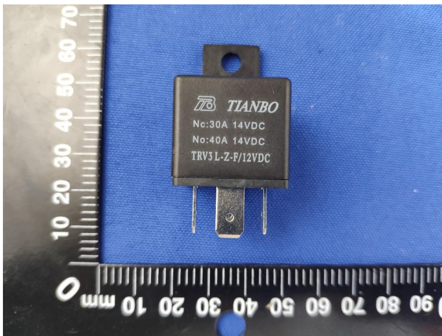
Accessory-4-Pin Relay
